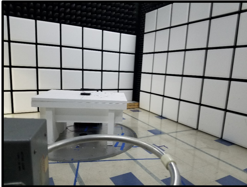
Radiated Emissions
