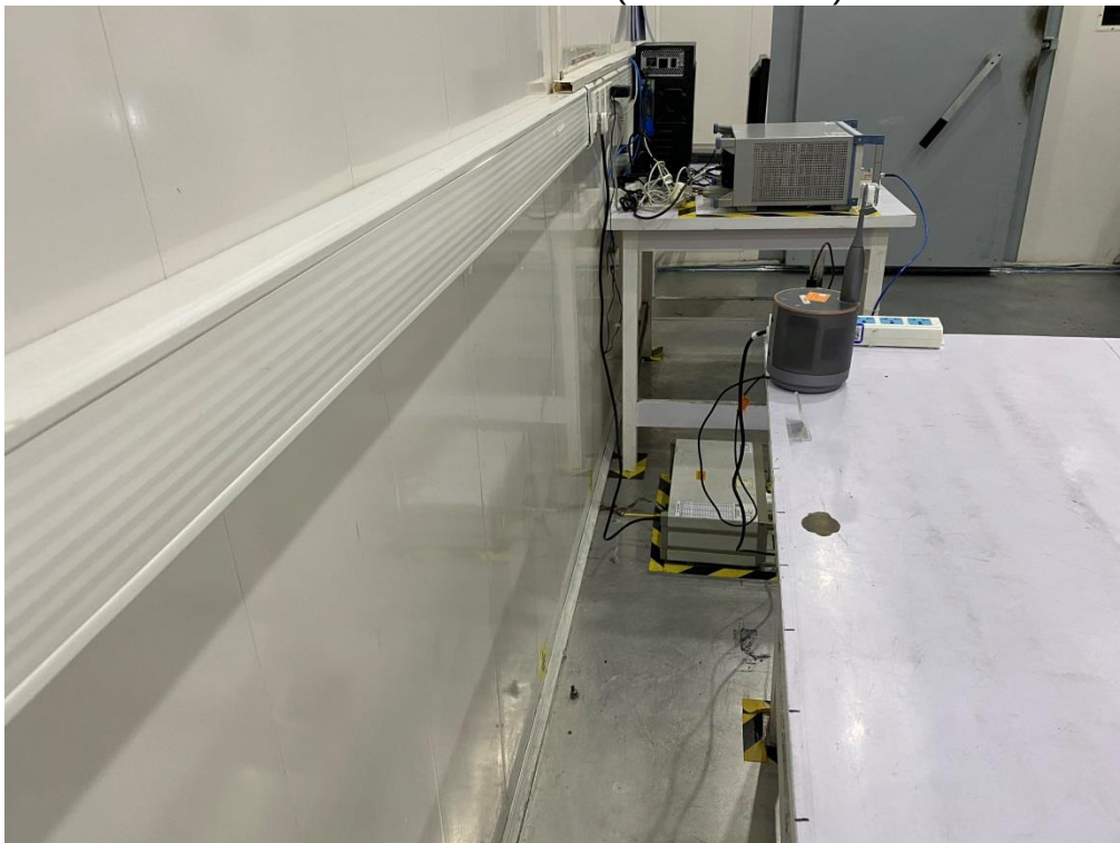
Conducted Emission(For side face)
