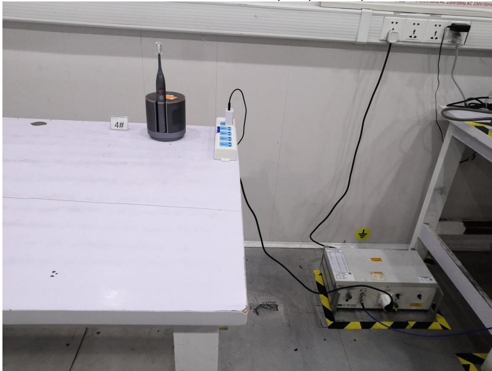
Conducted Emission(For positive)
