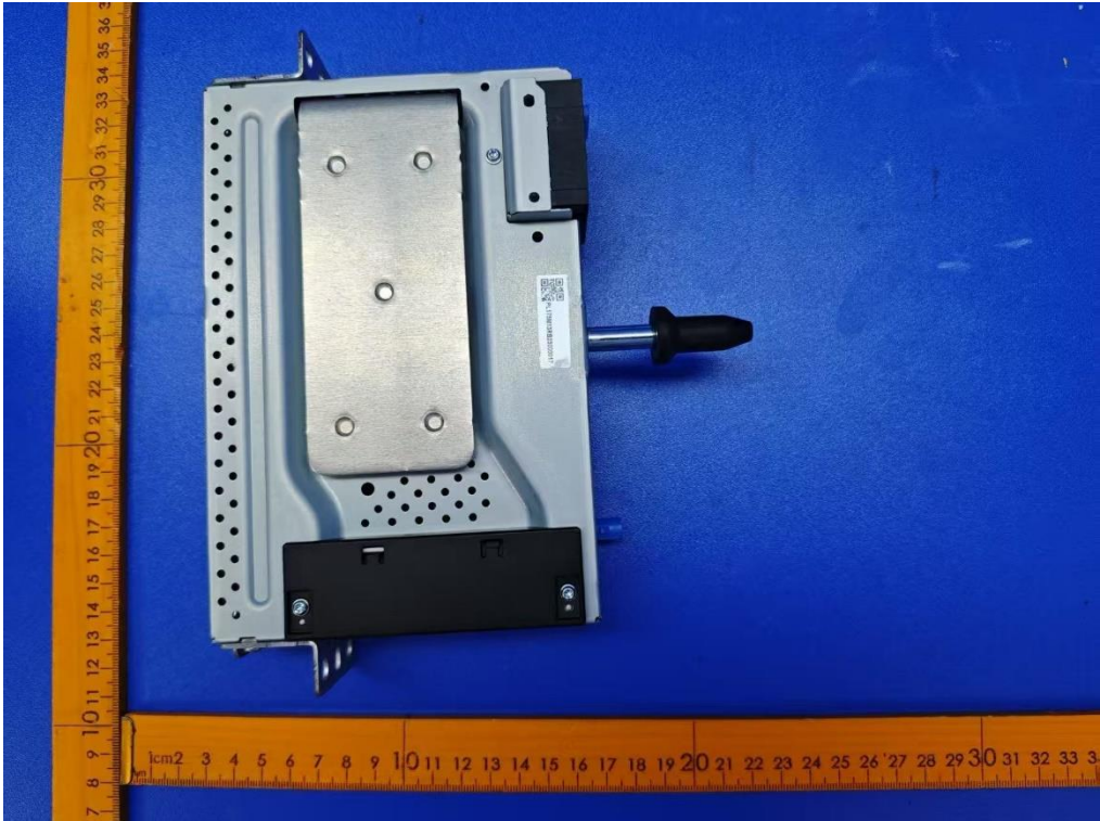
Figure 1 External view
