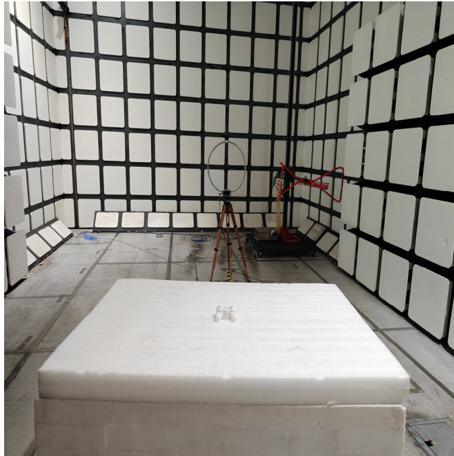
Radiated Emissions View (Below 30MHz)
