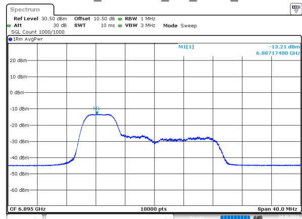
802.11ax20_6895MHz_RU_52/37_Chain 0
