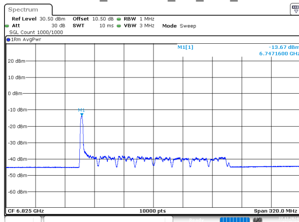
802.11ax160_6825MHz_RU_26/0_Chain 3
