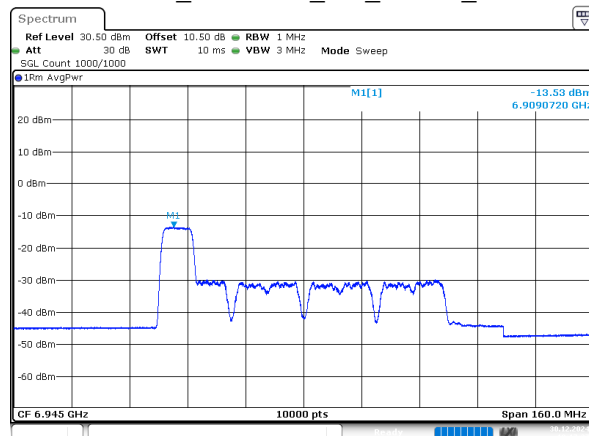
802.11ax80_6945MHz_RU_106/53_Chain 1
