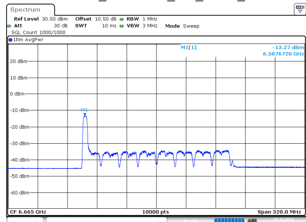
802.11ax160_6665MHz_RU_52/37_Chain 2
