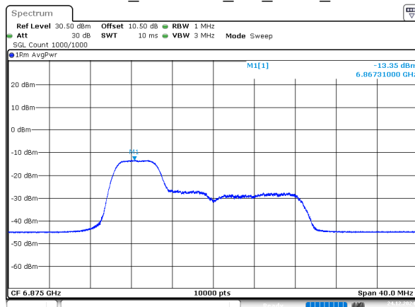
802.11ax20_6875MHz_RU_52/37_Chain 0
