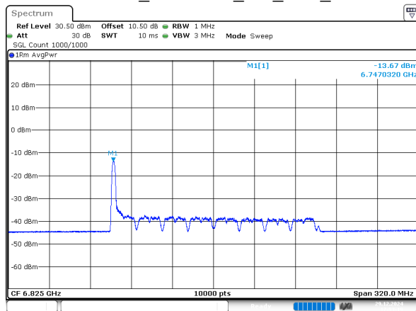
802.11ax160_6825MHz_RU_26/0_Chain 2
