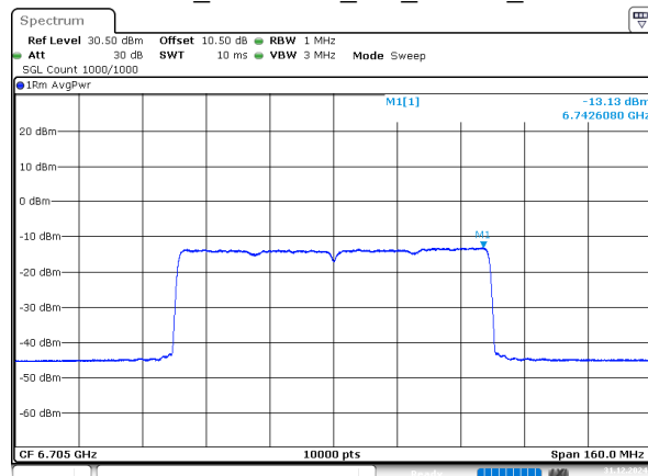
802.11ax80_6705MHz_RU_996/67_Chain 2
