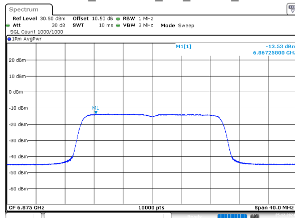
802.11ax20_6875MHz_RU_242/61_Chain 2
