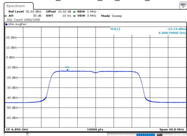
802.11ax20_6895MHz_RU_242/61_Chain 2
