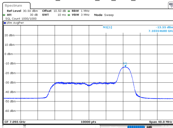
802.11ax20_7095MHz_RU_26/8_Chain 2
