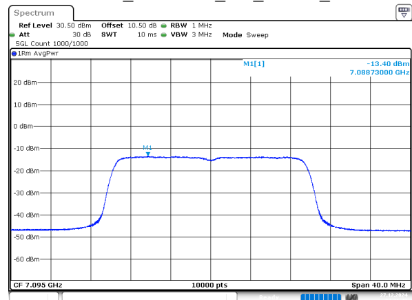
802.11ax20_7095MHz_RU_242/61_Chain 1
