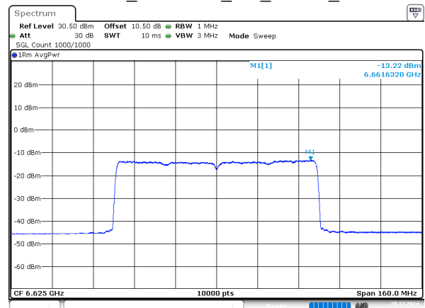
802.11ax80_6625MHz_RU_996/67_Chain 2
