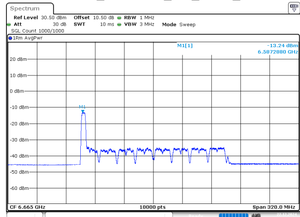
802.11ax160_6665MHz_RU_52/37_Chain 0
