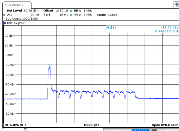
802.11ax160_6825MHz_RU_52/37_Chain 0
