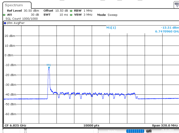
802.11ax160_6825MHz_RU_26/0_Chain 1
