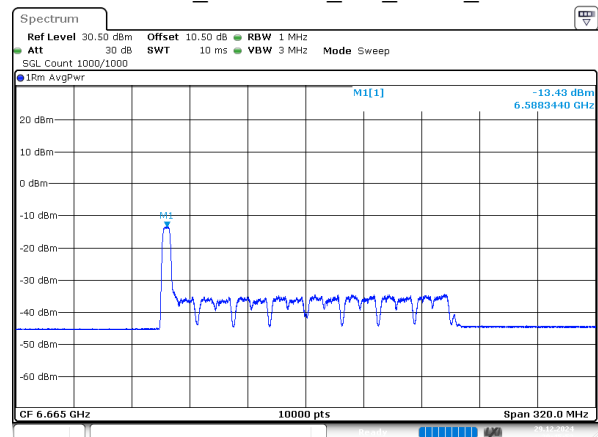
802.11ax160_6665MHz_RU_52/37_Chain 1
