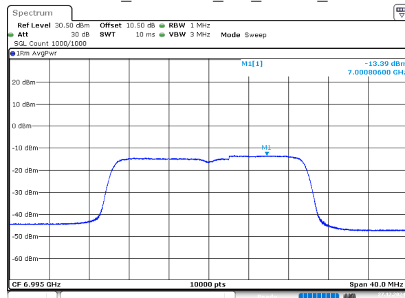
802.11ax20_6995MHz_RU_242/61_Chain 2
