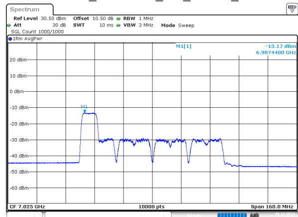
802.11ax80_7025MHz_RU_106/53_Chain 2
