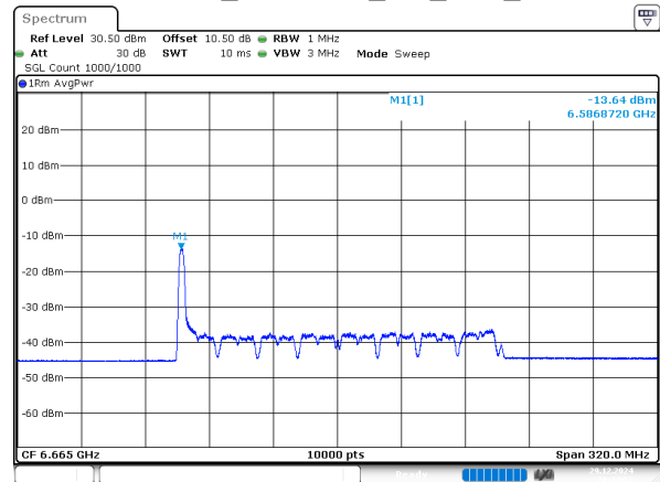
802.11ax160_6665MHz_RU_26/0_Chain 1
