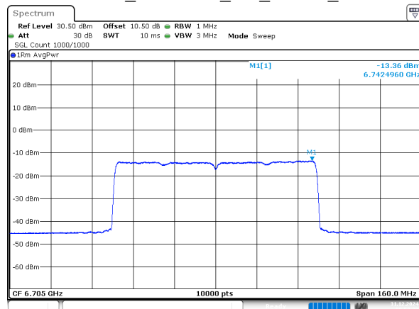
802.11ax80_6705MHz_RU_996/67_Chain 1
