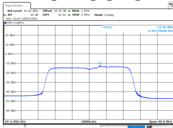
802.11ax20_6995MHz_RU_242/61_Chain 1
