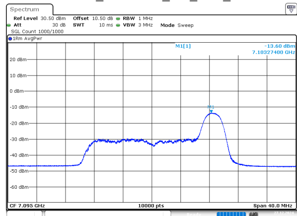
802.11ax20_7095MHz_RU_26/8_Chain 3
