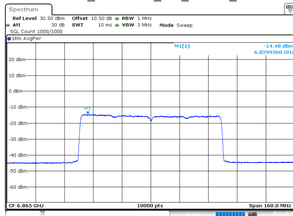
802.11ax80_6865MHz_RU_996/67_Chain 2
