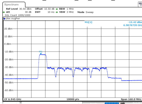
802.11ax80_6945MHz_RU_106/53_Chain 3
