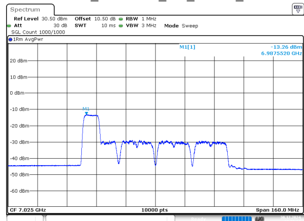
802.11ax80_7025MHz_RU_106/53_Chain 1
