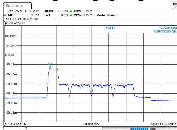
802.11ax80_6945MHz_RU_106/53_Chain 2
