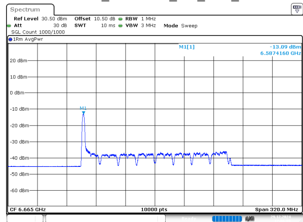
802.11ax160_6665MHz_RU_26/0_Chain 2
