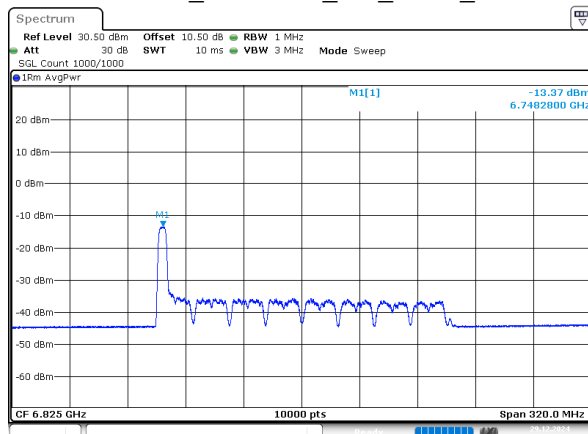
802.11ax160_6825MHz_RU_52/37_Chain 2
