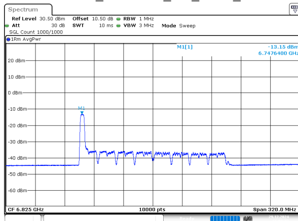
802.11ax160_6825MHz_RU_52/37_Chain 1
