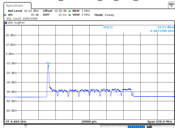
802.11ax160_6665MHz_RU_26/0_Chain 3
