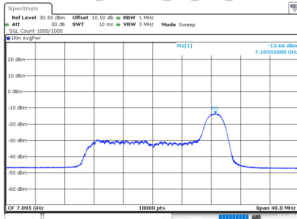
802.11ax20_7095MHz_RU_26/8_Chain 0
