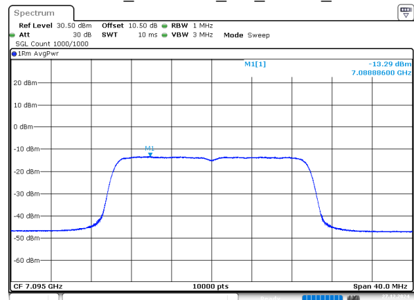
802.11ax20_7095MHz_RU_242/61_Chain 2
