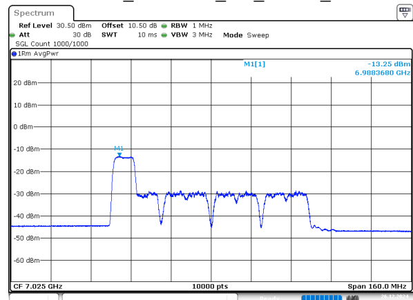
802.11ax80_7025MHz_RU_106/53_Chain 3
