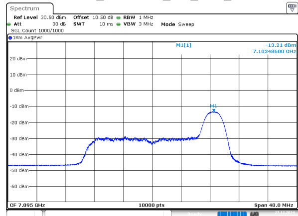
802.11ax20_7095MHz_RU_26/8_Chain 1
