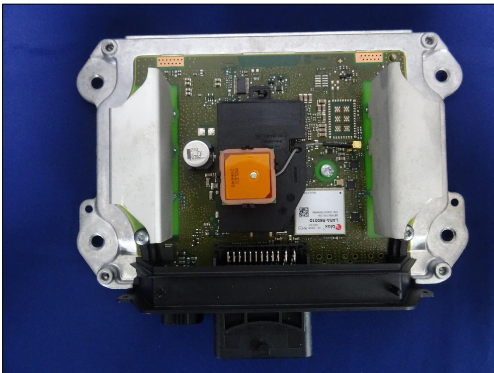
Figure 2: Front view of the PCB
