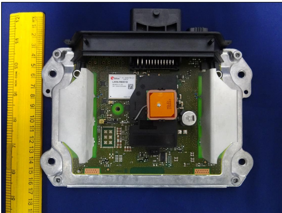
Figure 6: Dimensional view of PCB
