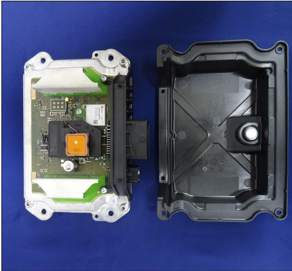
Figure 1: VCU Front panel removed
