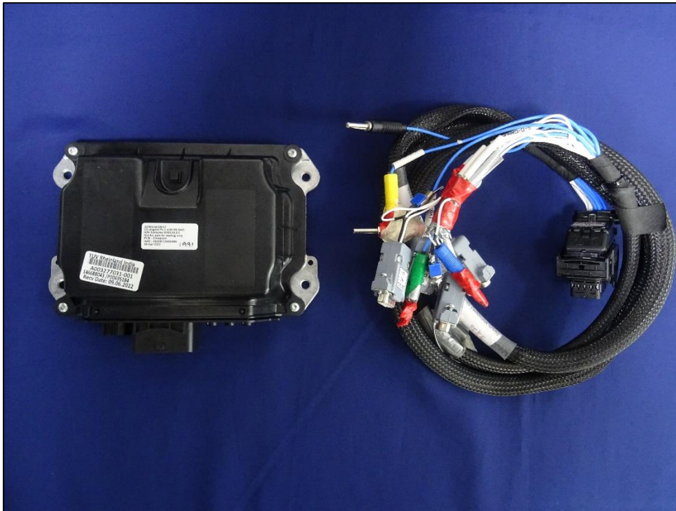
Figur 11: VCU with Power Cable
