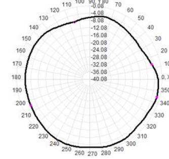
Total(H-XY), Max=-1.81dBi, CirD=5.05
