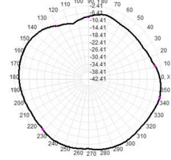
Total(H-XY), Max=-2.41dBi, CirD=8.88
