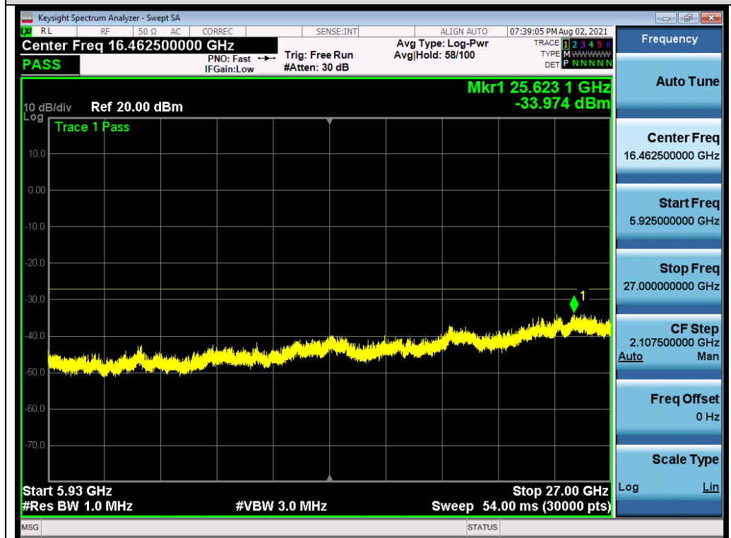
Test_Graph_802.11ac80_ANT1_5775_MCS9_Frequency Band4
