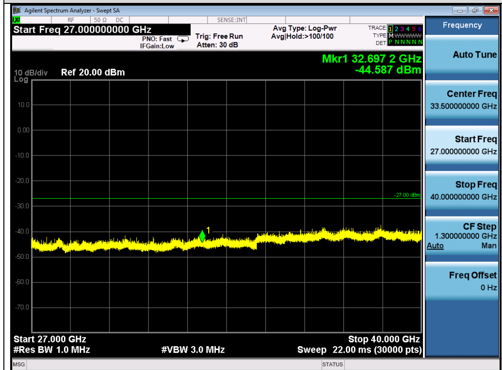
Test_Graph_802.11ac80_ANT1_5530_MCS9_Frequency Band 5
