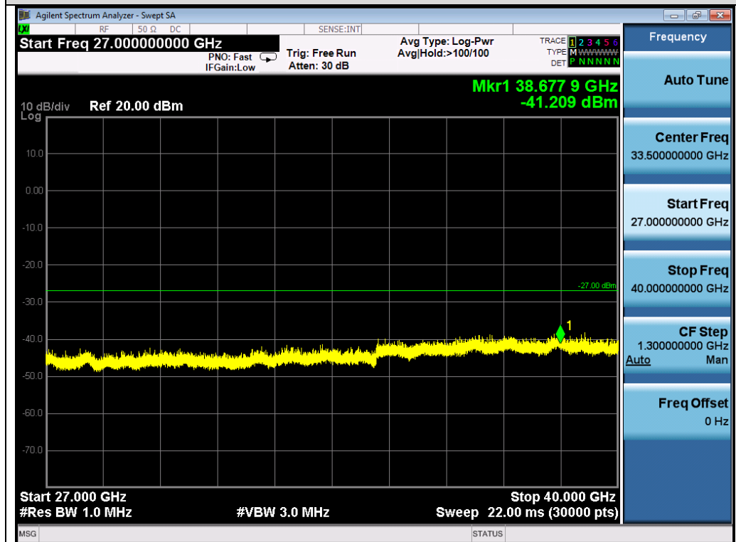
Test_Graph_802.11n40_ANT1_5230_MCS0_Frequency Band 5
