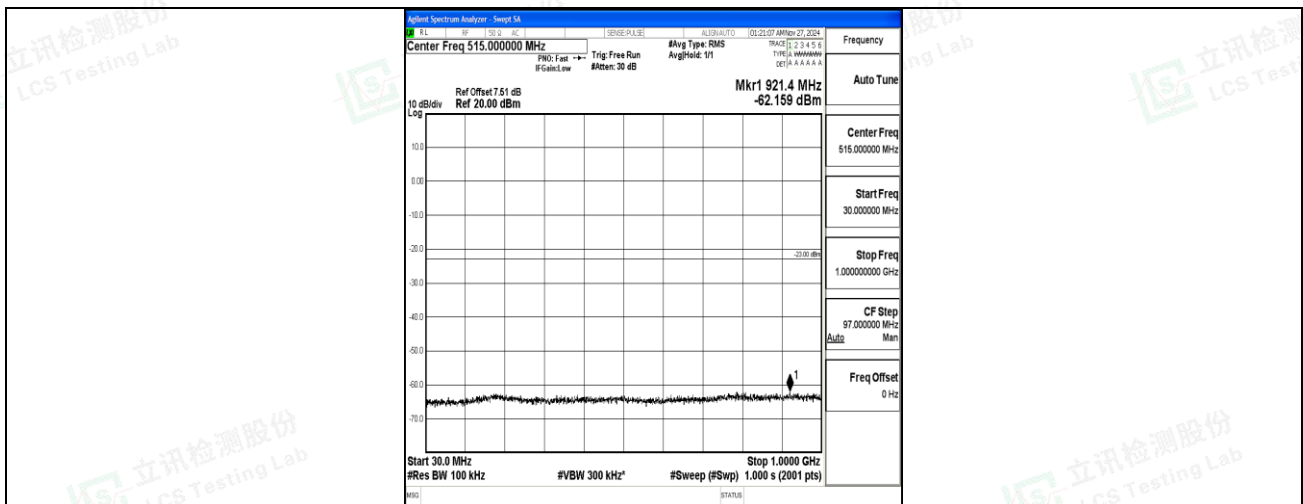
Band66_15MHz_16QAM_132047_1RB#0_30~1000_30~1000
