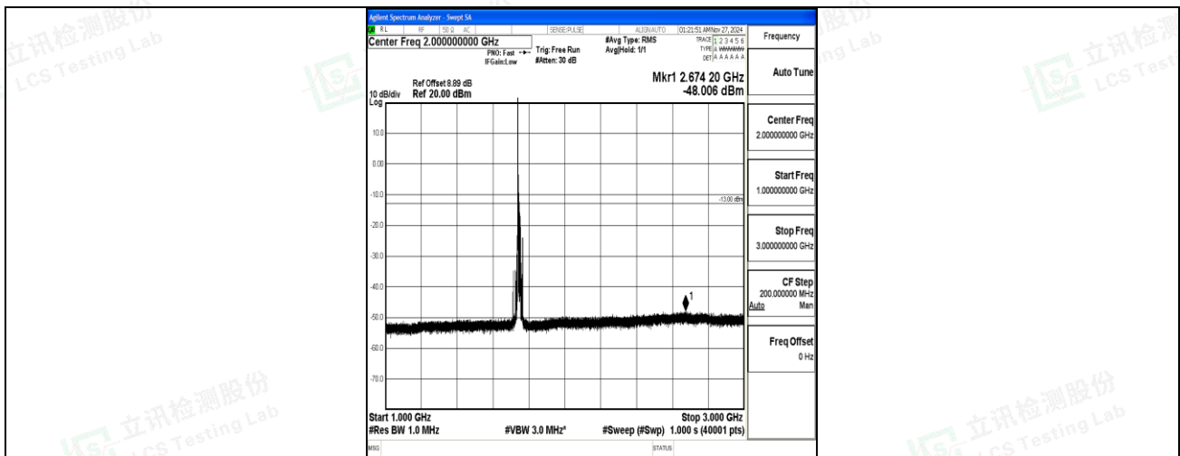
Band66_15MHz_QPSK_132322_1RB#0_1000~3000_1000~3000
