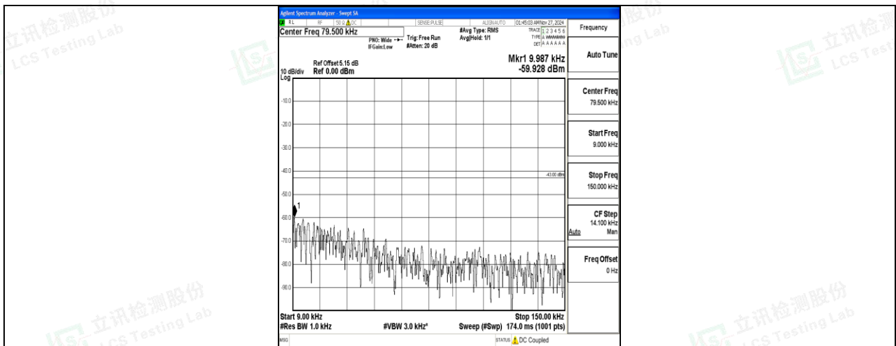
Band66_20MHz_16QAM_132572_1RB#0_0.009~0.15_0.009~0.15
