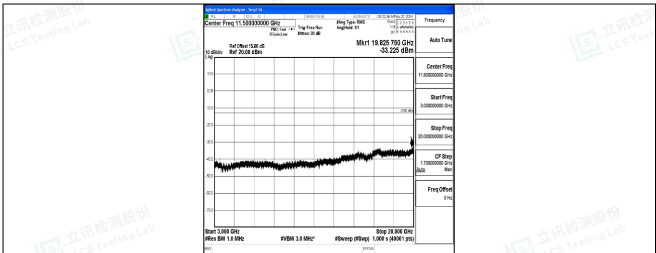
Band66_15MHz_16QAM_132322_1RB#0_3000~20000_3000~20000
