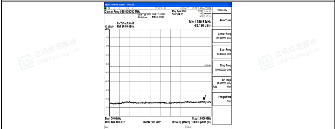
Band66_10MHz_16QAM_132622_1RB#0_30~1000_30~1000
