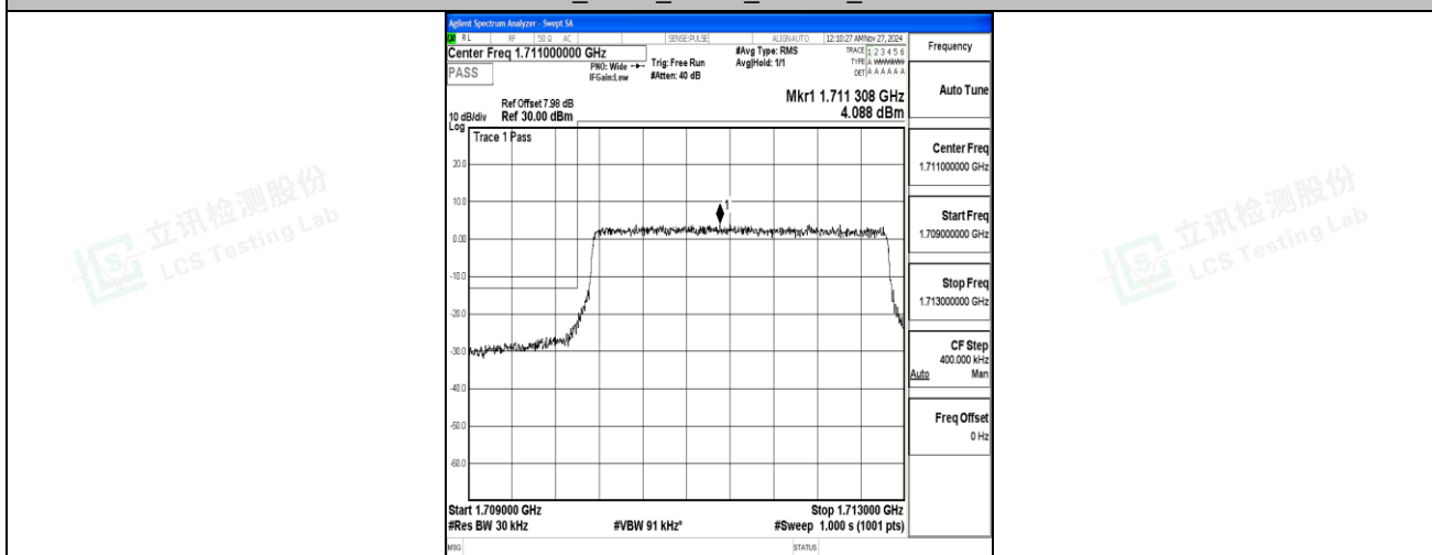
Band66_3MHz_16QAM_131987_15RB#0
