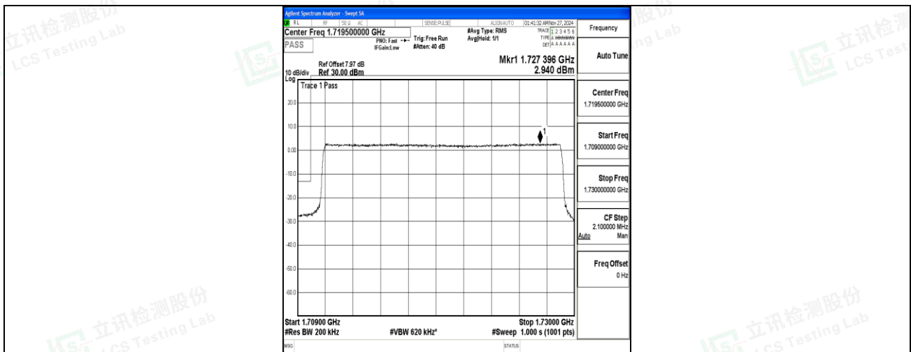
Band66_20MHz_16QAM_132072_100RB#0
