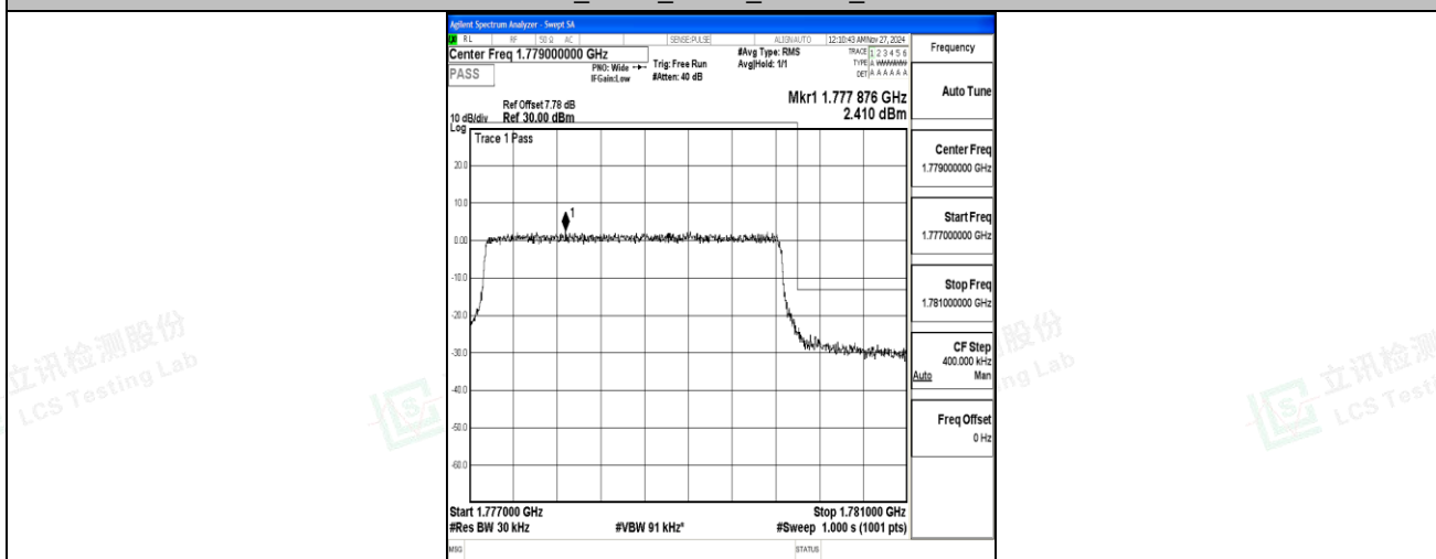
Band66_3MHz_16QAM_132657_15RB#0
