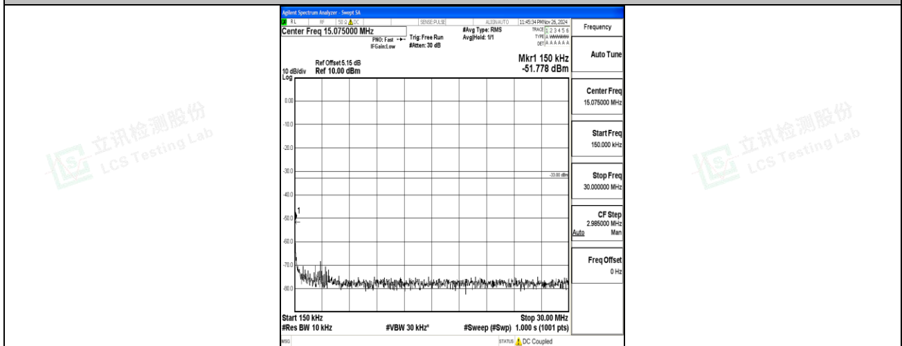
Band66_1.4MHz_QPSK_132665_1RB#0_0.15~30_0.15~30
