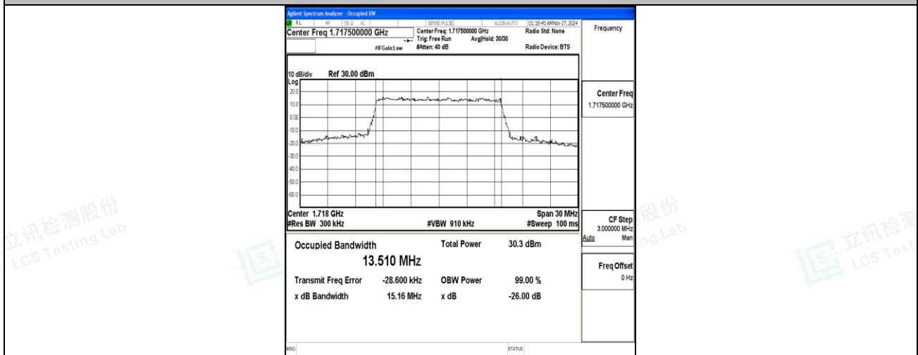
Band66-15MHz-16QAM-132047-75RB#0-PASS
