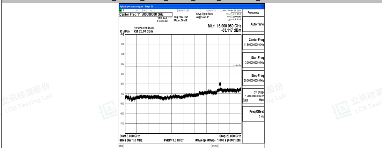
Band66_1.4MHz_QPSK_132322_1RB#0_3000~20000_3000~20000
