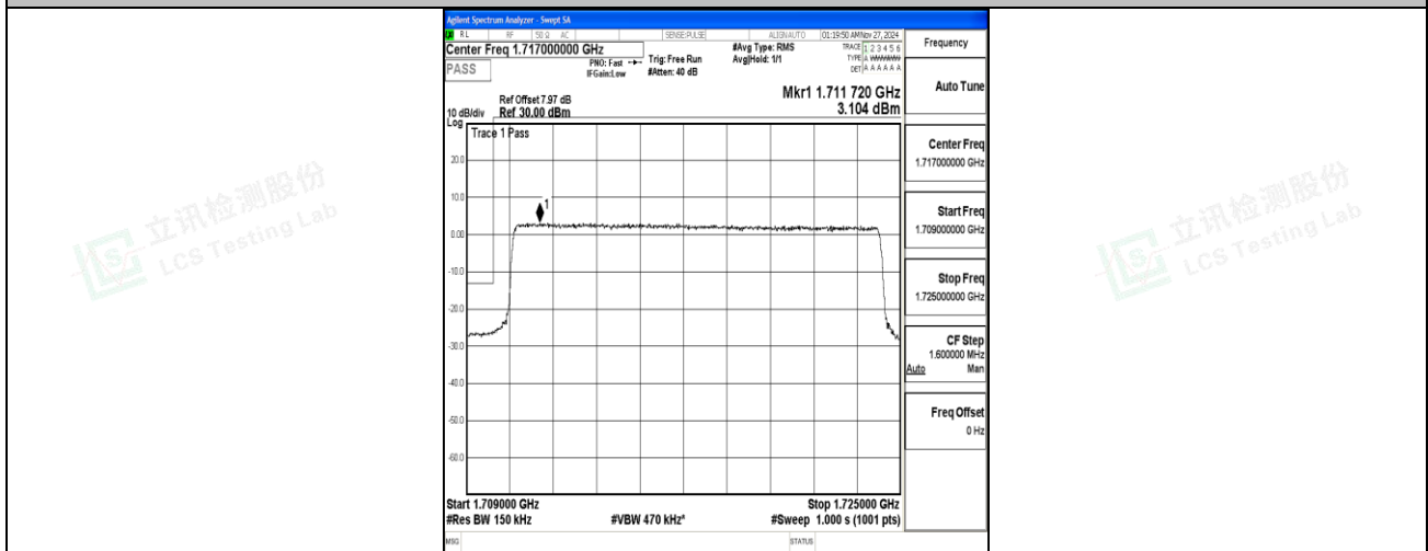
Band66_15MHz_16QAM_132047_75RB#0
