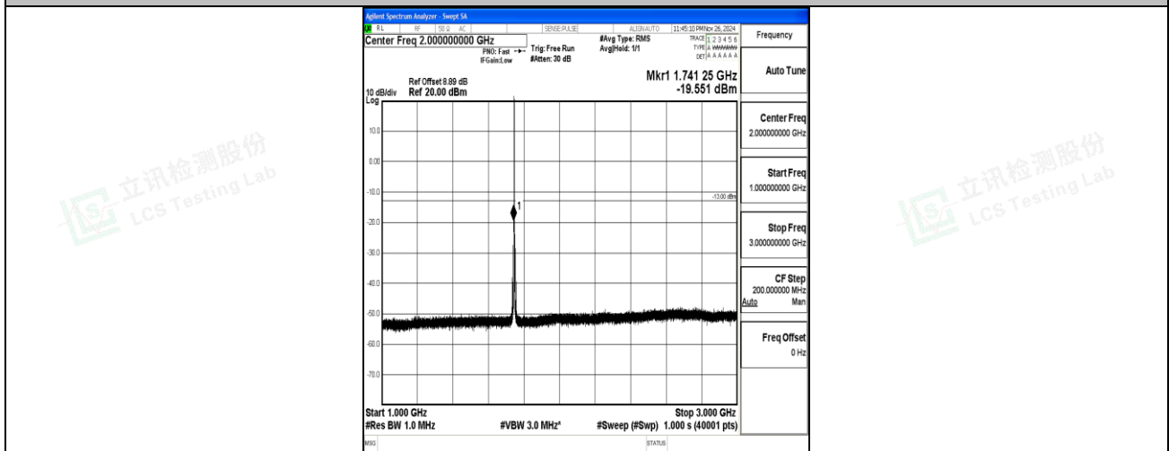
Band66_1.4MHz_16QAM_132322_1RB#0_1000~3000_1000~3000
