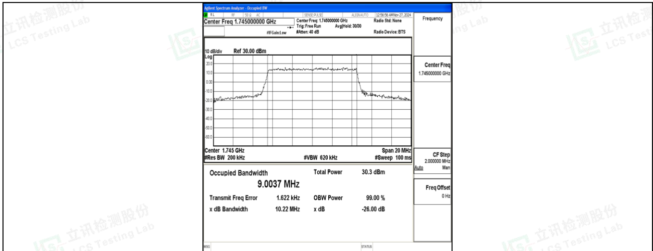
Band66-10MHz-16QAM-132322-50RB#0-PASS
