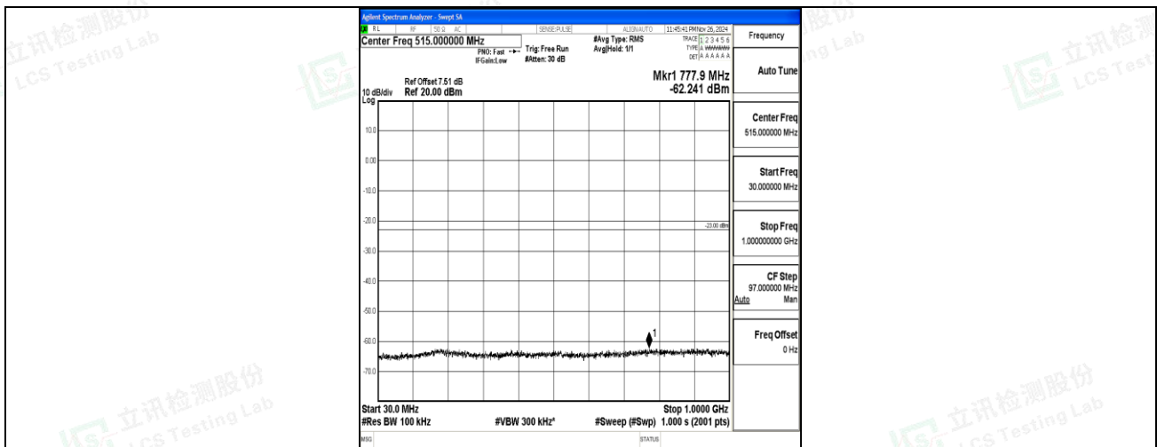
Band66_1.4MHz_QPSK_132665_1RB#0_30~1000_30~1000
