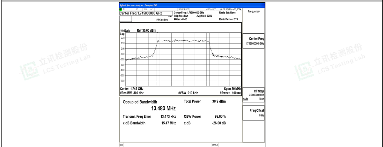
Band66-15MHz-QPSK-132322-75RB#0-PASS
