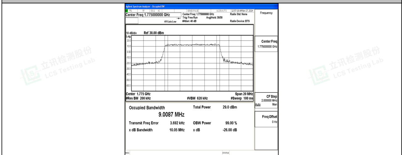
Band66-10MHz-16QAM-132622-50RB#0-PASS
