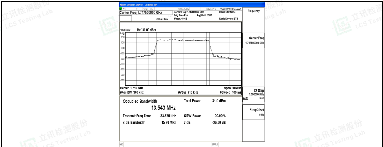
Band66-15MHz-QPSK-132047-75RB#0-PASS
