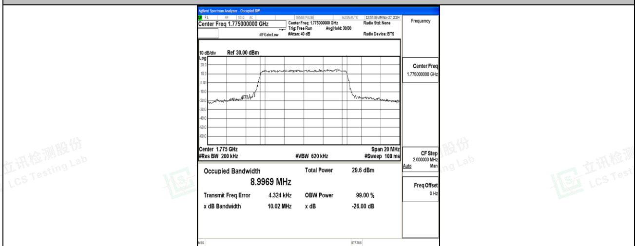
Band66-10MHz-QPSK-132622-50RB#0-PASS
