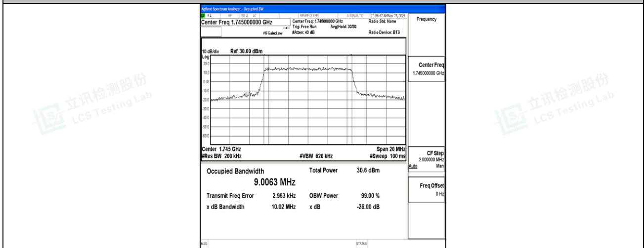
Band66-10MHz-QPSK-132322-50RB#0-PASS
