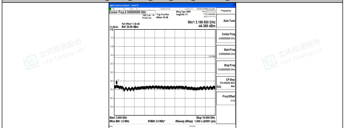
Band17_10MHz_QPSK_23800_1RB#0_3000~10000_3000~10000
