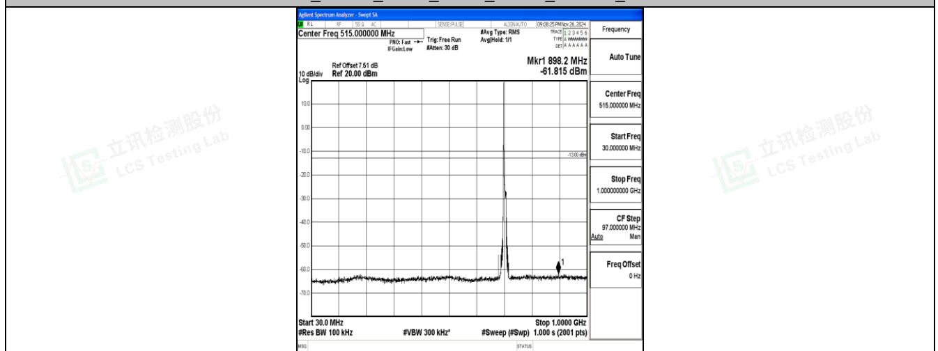
Band17_10MHz_QPSK_23790_1RB#0_30~1000_30~1000
