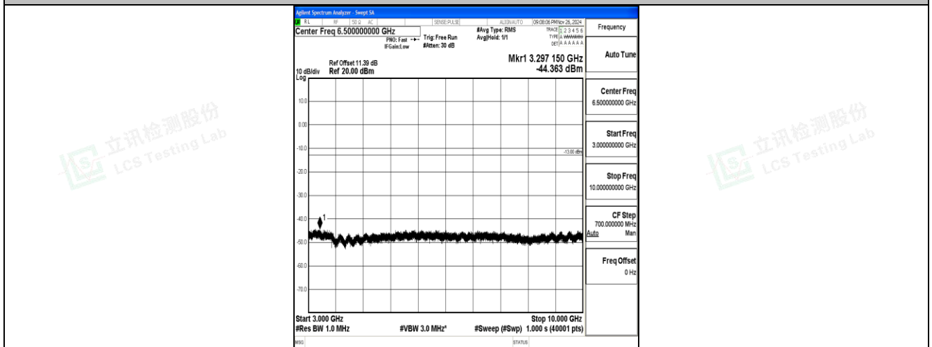
Band17_10MHz_16QAM_23780_1RB#0_3000~10000_3000~10000
