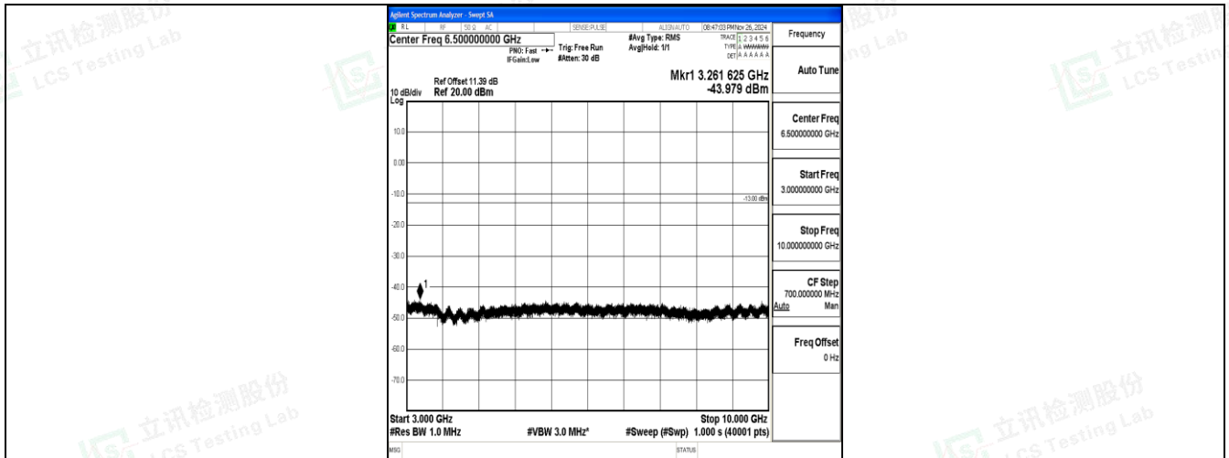
Band17_5MHz_16QAM_23790_1RB#0_3000~10000_3000~10000
