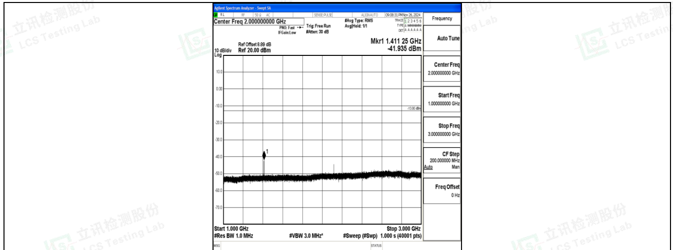
Band17_10MHz_QPSK_23790_1RB#0_1000~3000_1000~3000
