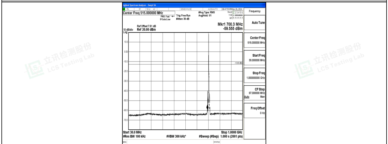
Band17_5MHz_16QAM_23825_1RB#0_30~1000_30~1000
