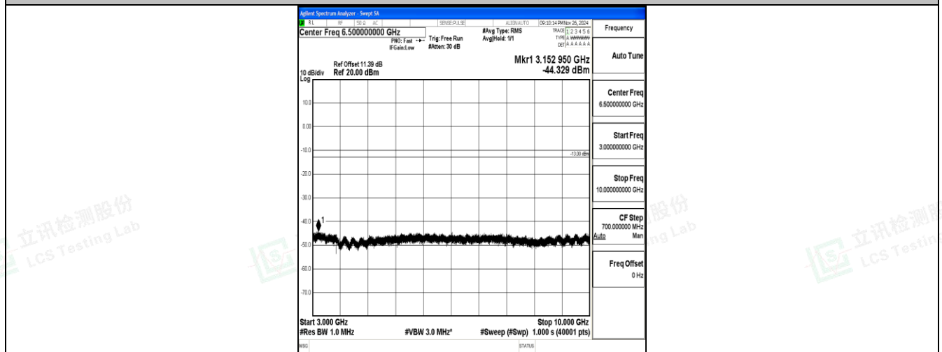
Band17_10MHz_16QAM_23800_1RB#0_3000~10000_3000~10000
