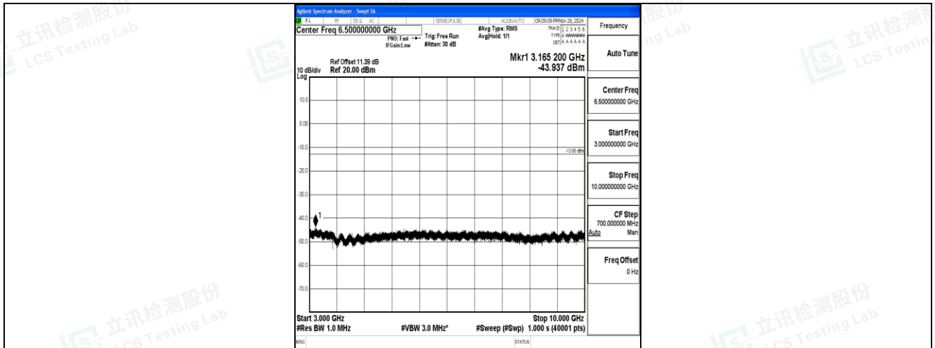
Band17_10MHz_16QAM_23790_1RB#0_3000~10000_3000~10000
