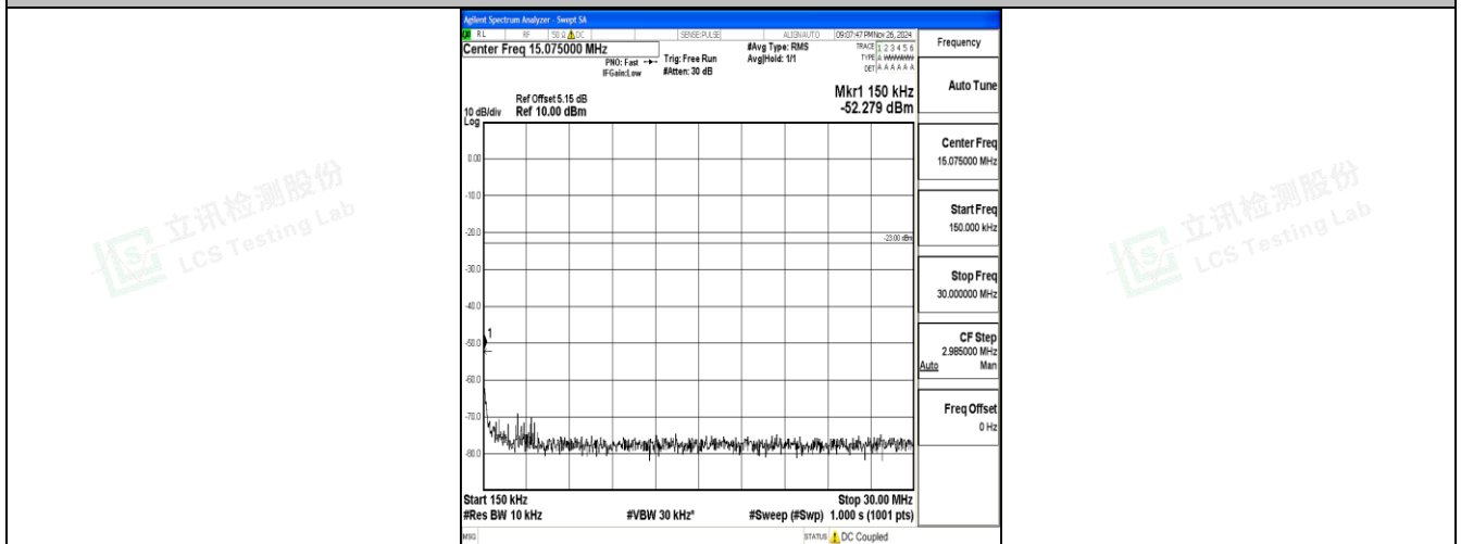
Band17_10MHz_16QAM_23780_1RB#0_0.15~30_0.15~30
