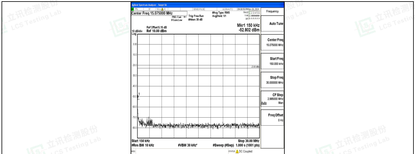
Band17_10MHz_16QAM_23790_1RB#0_0.15~30_0.15~30
