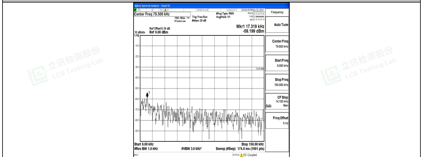
Band17_10MHz_16QAM_23790_1RB#0_0.009~0.15_0.009~0.15
