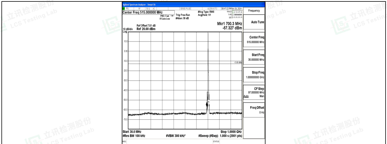
Band17_5MHz_QPSK_23825_1RB#0_30~1000_30~1000
