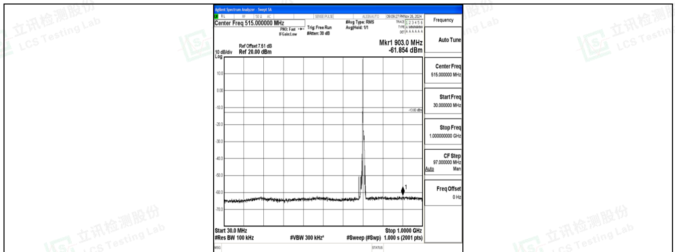
Band17_10MHz_QPSK_23800_1RB#0_30~1000_30~1000
