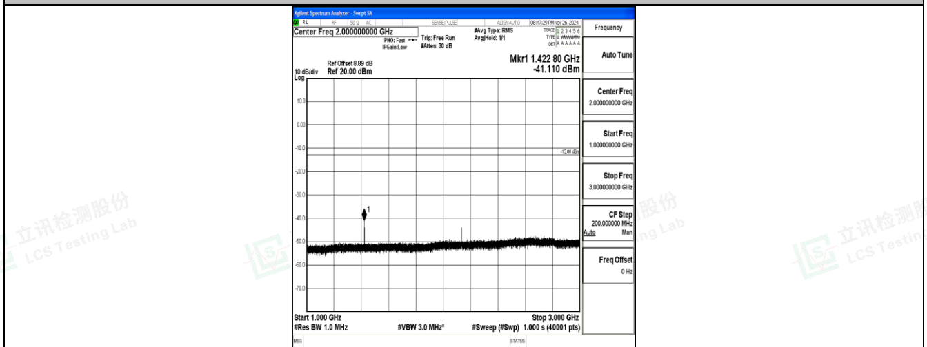
Band17_5MHz_QPSK_23825_1RB#0_1000~3000_1000~3000
