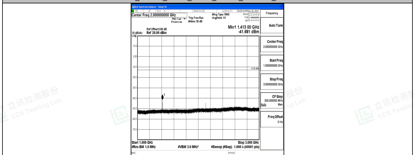
Band17_10MHz_QPSK_23800_1RB#0_1000~3000_1000~3000
