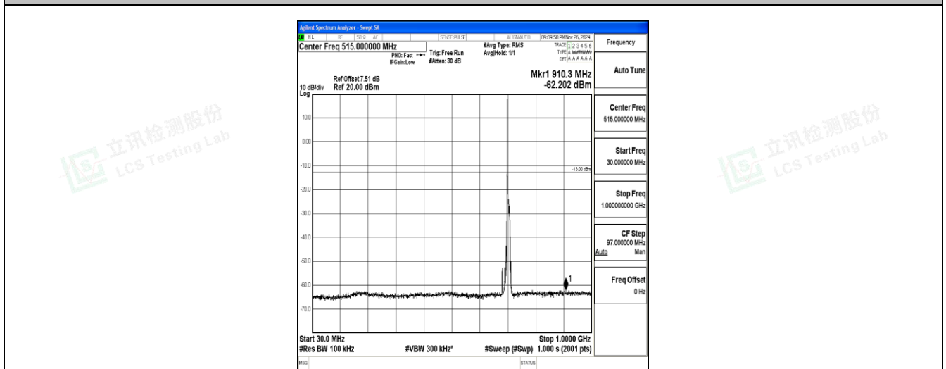
Band17_10MHz_16QAM_23800_1RB#0_30~1000_30~1000
