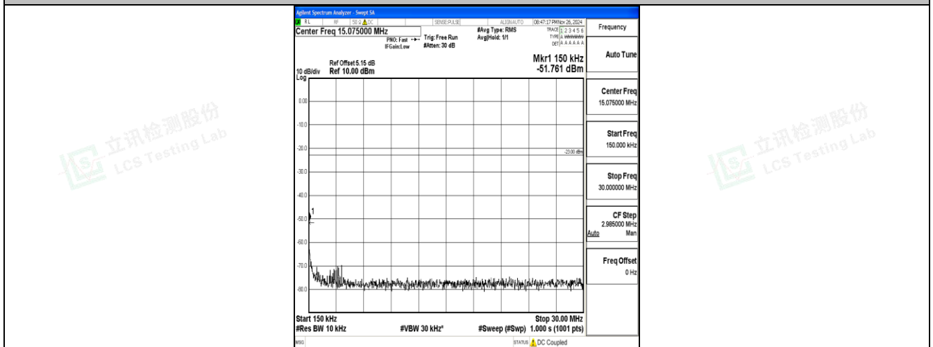
Band17_5MHz_QPSK_23825_1RB#0_0.15~30_0.15~30
