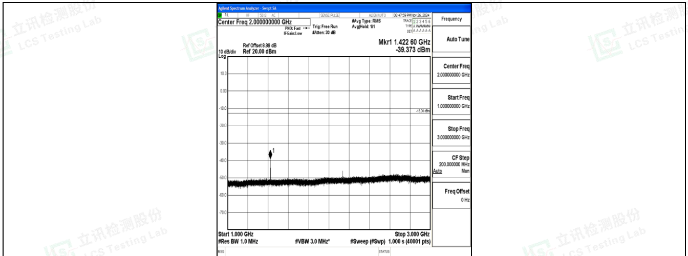
Band17_5MHz_16QAM_23825_1RB#0_1000~3000_1000~3000
