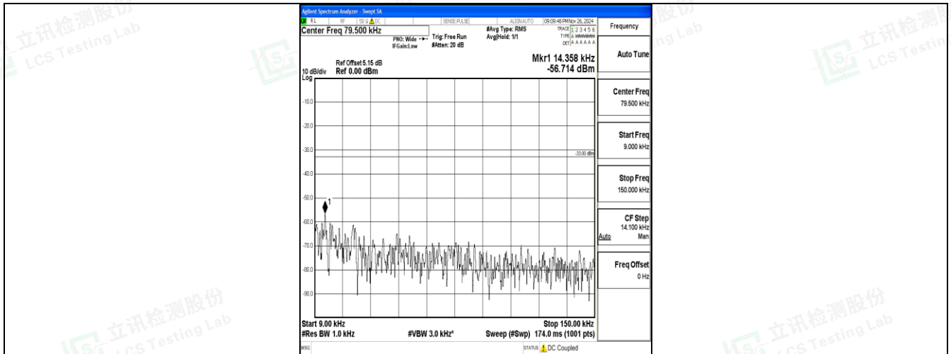
Band17_10MHz_16QAM_23800_1RB#0_0.009~0.15_0.009~0.15
