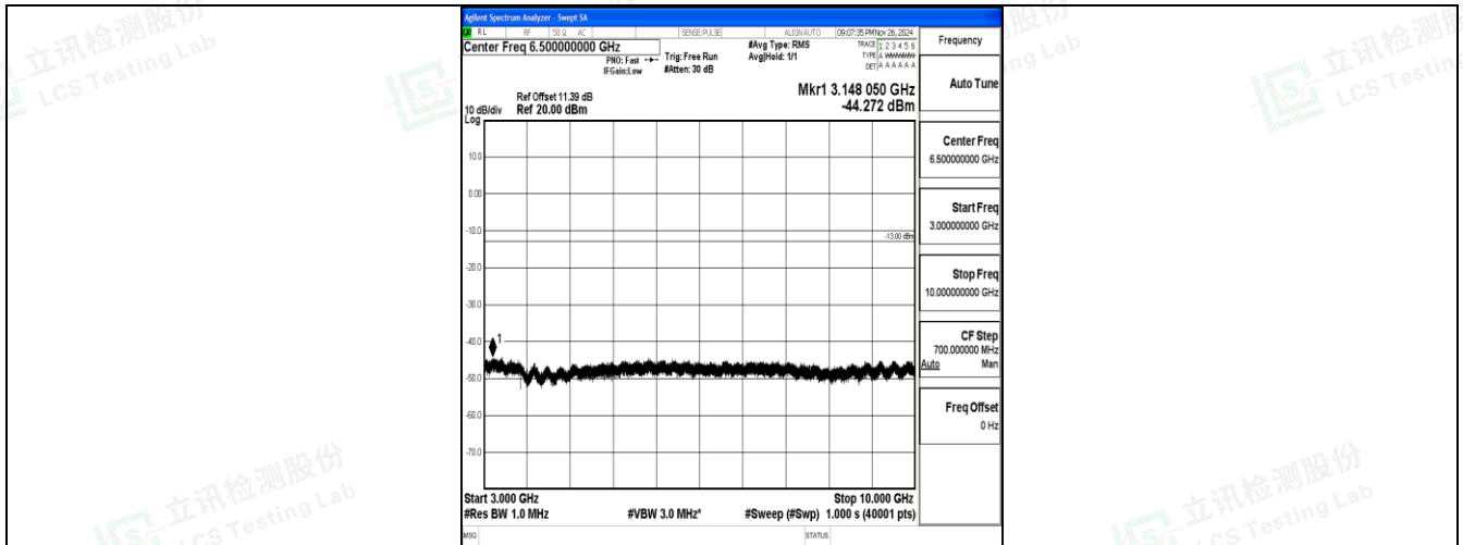
Band17_10MHz_QPSK_23780_1RB#0_3000~10000_3000~10000
