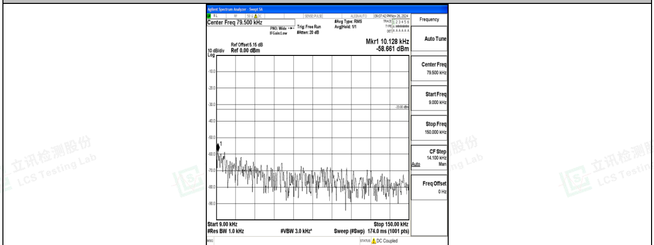
Band17_10MHz_16QAM_23780_1RB#0_0.009~0.15_0.009~0.15
