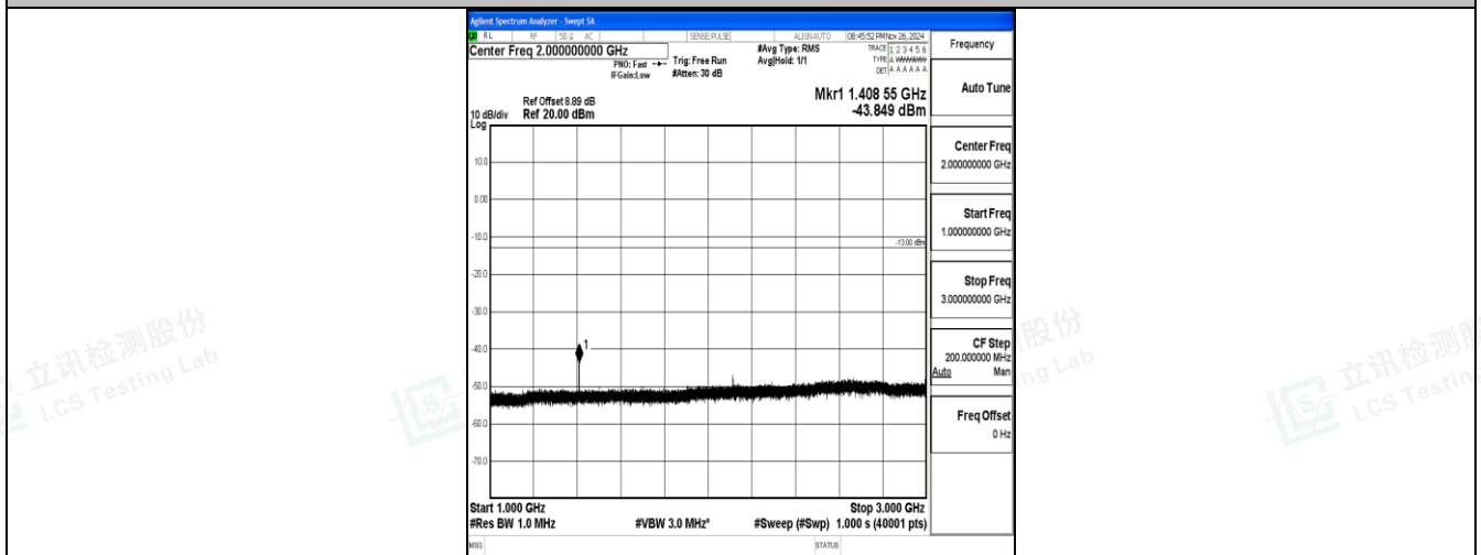
Band17_5MHz_16QAM_23755_1RB#0_1000~3000_1000~3000
