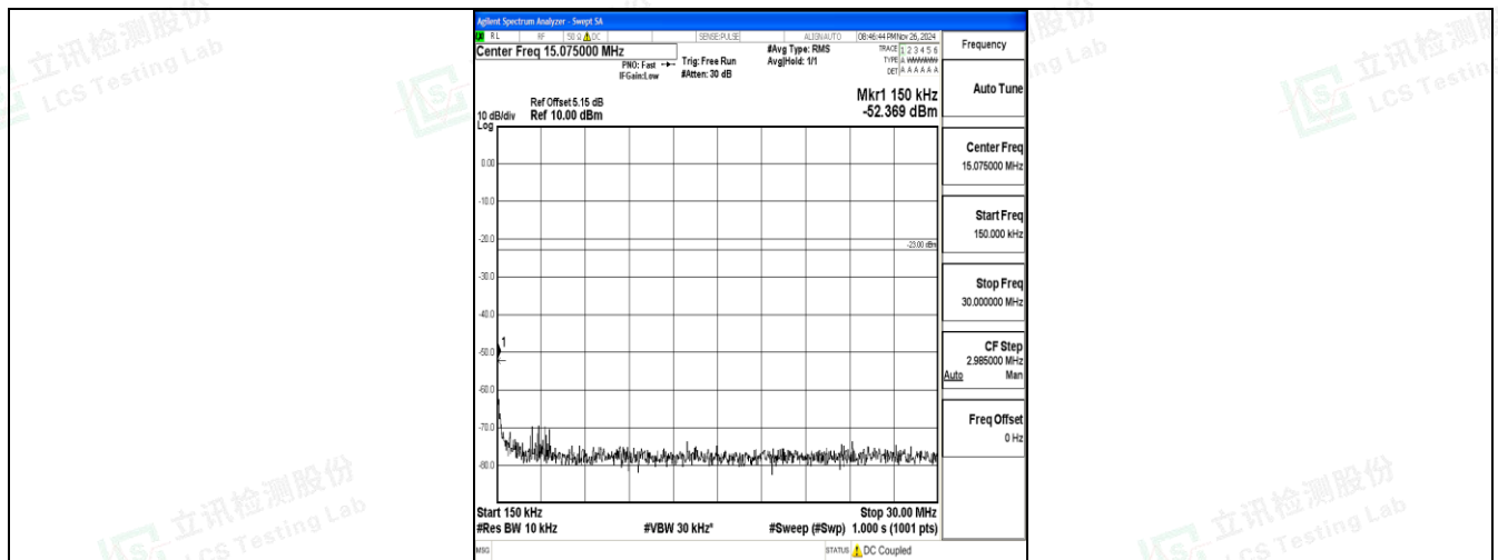
Band17_5MHz_16QAM_23790_1RB#0_0.15~30_0.15~30
