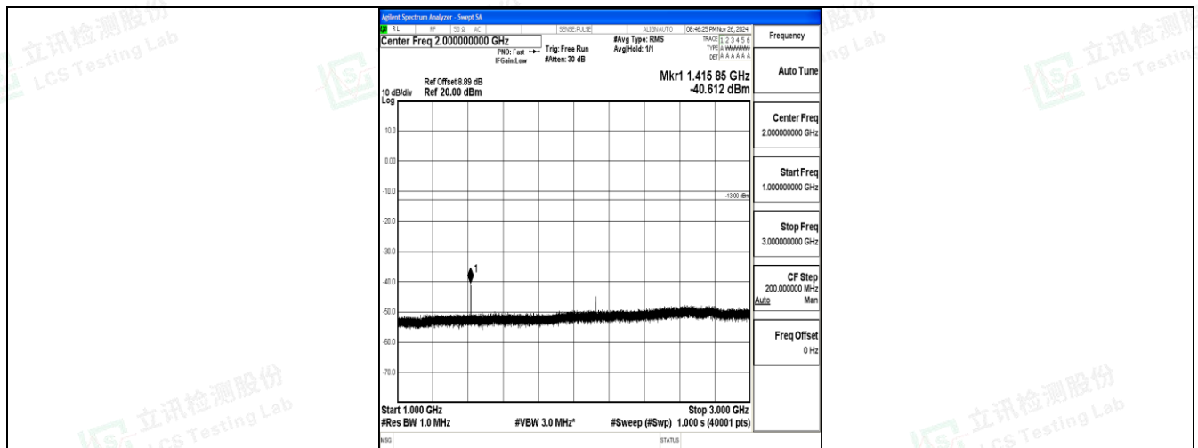
Band17_5MHz_QPSK_23790_1RB#0_1000~3000_1000~3000
