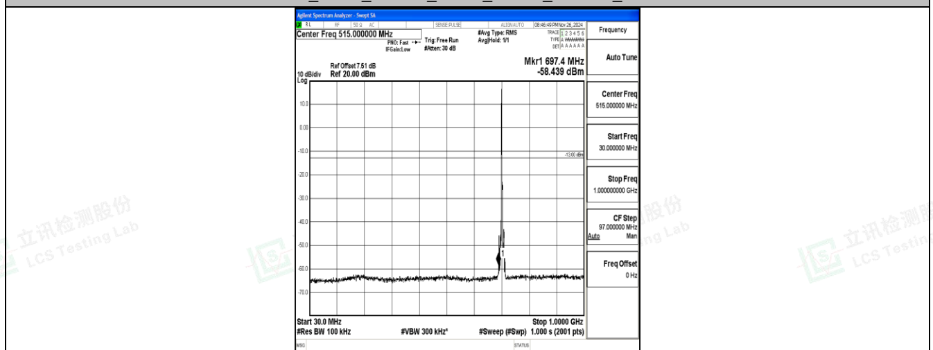
Band17_5MHz_16QAM_23790_1RB#0_30~1000_30~1000
