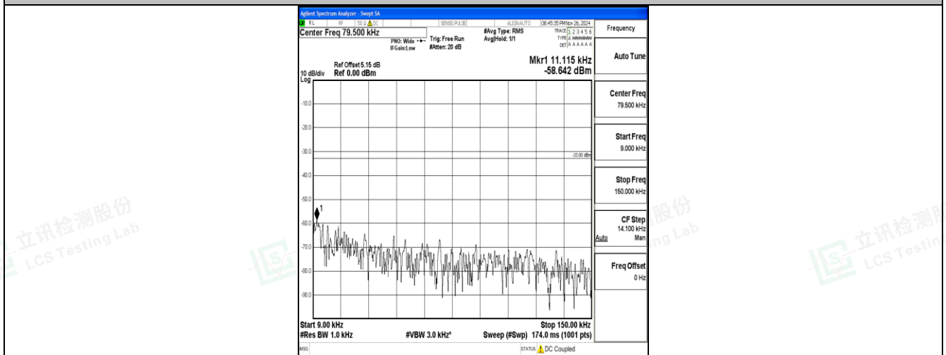
Band17_5MHz_16QAM_23755_1RB#0_0.009~0.15_0.009~0.15
