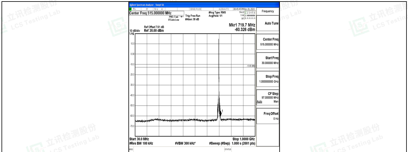
Band17_5MHz_16QAM_23755_1RB#0_30~1000_30~1000
