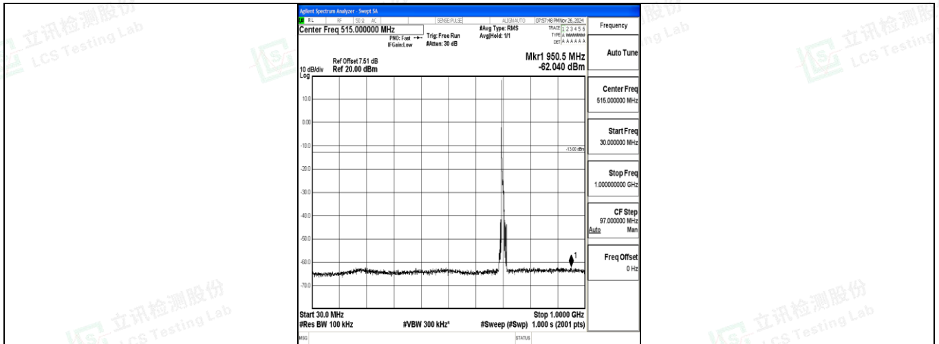
Band12_10MHz_16QAM_23095_1RB#0_30~1000_30~1000
