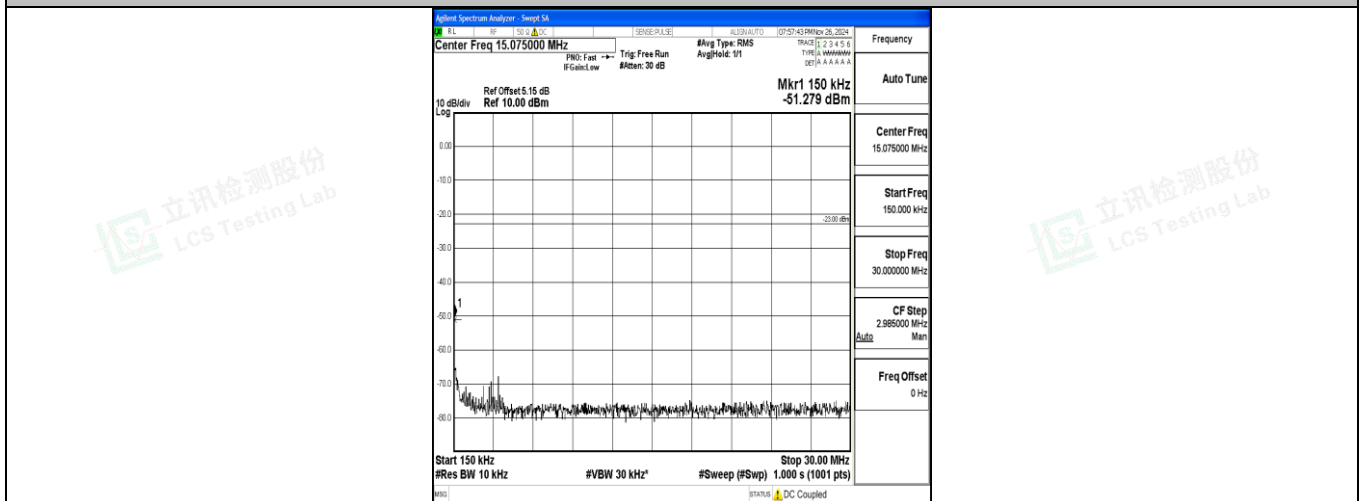
Band12_10MHz_16QAM_23095_1RB#0_0.15~30_0.15~30
