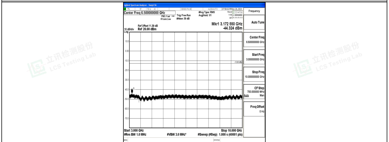
Band12_10MHz_16QAM_23095_1RB#0_3000~10000_3000~10000
