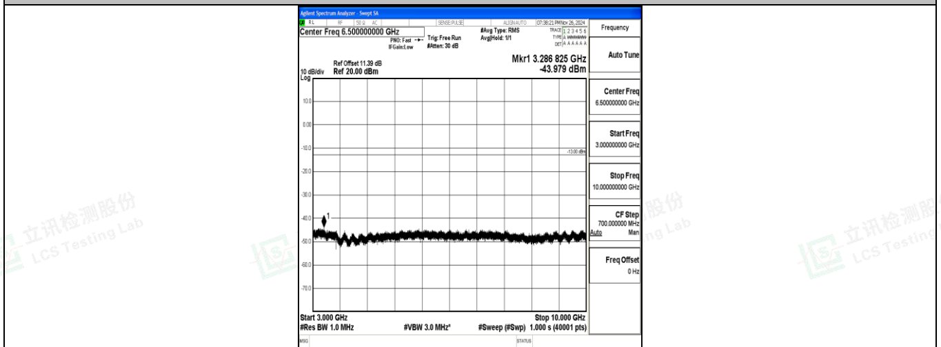
Band12_5MHz_QPSK_23155_1RB#0_3000~10000_3000~10000
