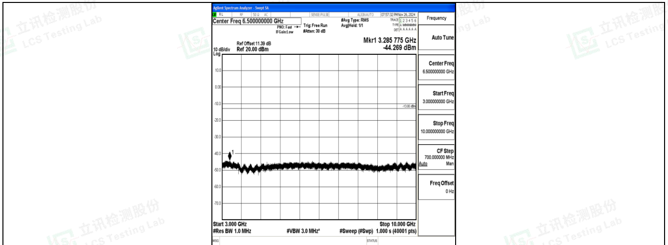
Band12_10MHz_QPSK_23095_1RB#0_3000~10000_3000~10000
