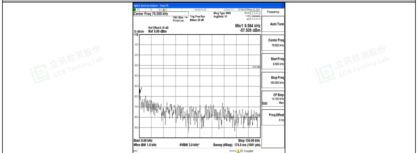
Band12_10MHz_16QAM_23130_1RB#0_0.009~0.15_0.009~0.15
