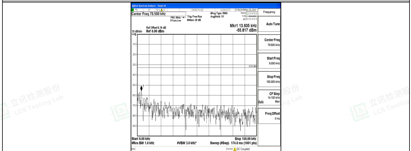
Band12_10MHz_QPSK_23060_1RB#0_0.009~0.15_0.009~0.15
