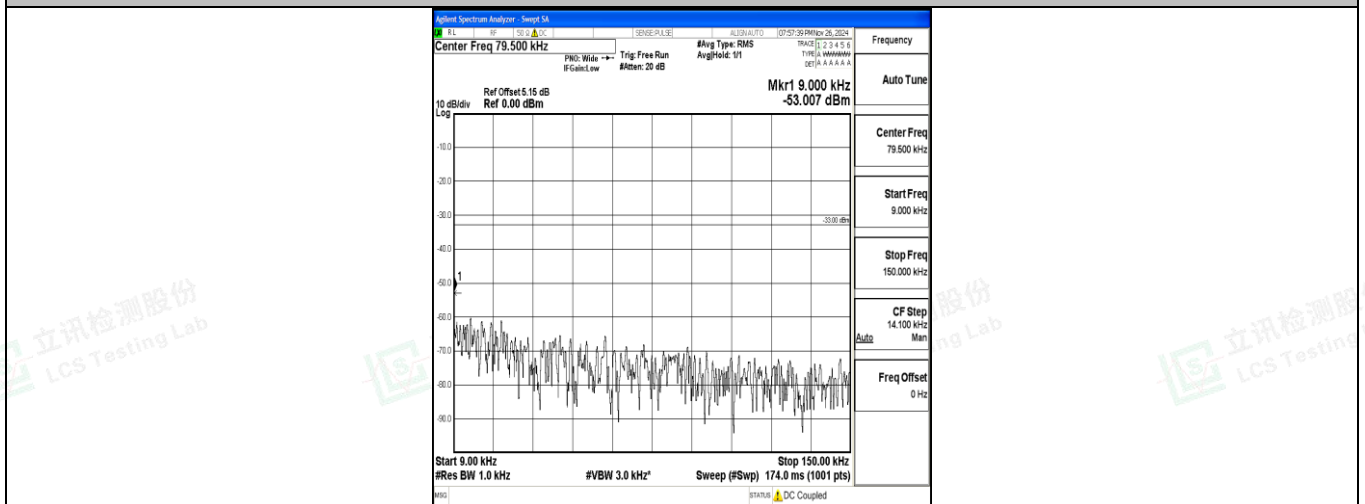
Band12_10MHz_16QAM_23095_1RB#0_0.009~0.15_0.009~0.15
