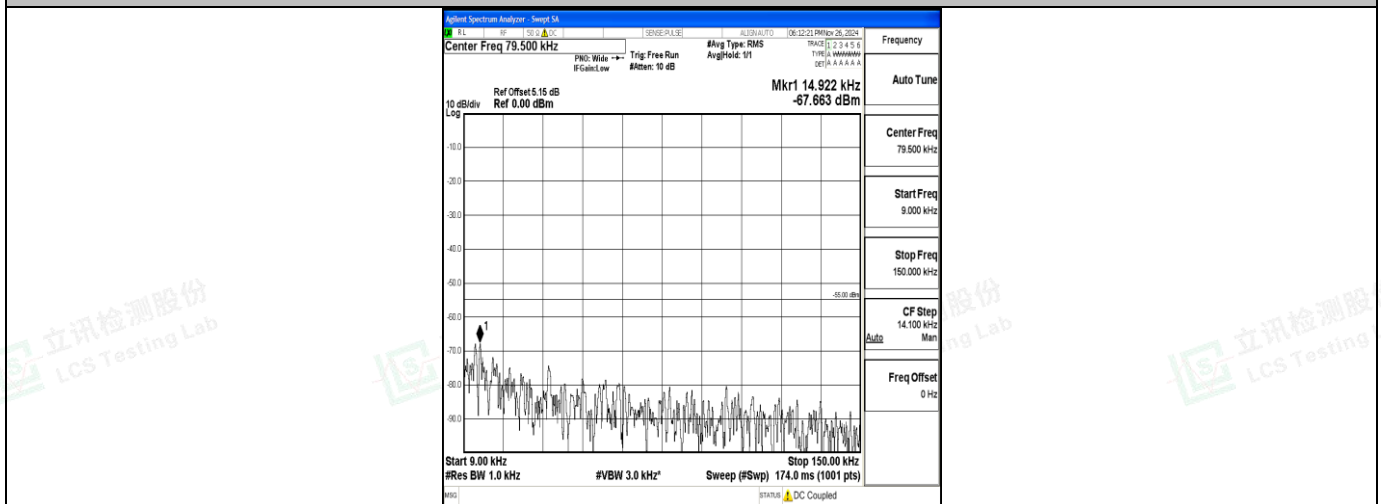
Band7_15MHz_QPSK_20825_1RB#0_0.009~0.15_0.009~0.15
