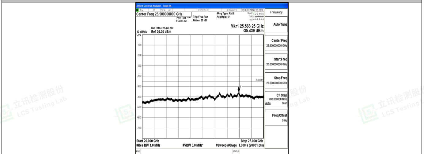
Band7_5MHz_16QAM_20775_1RB#0_20000~27000_20000~27000
