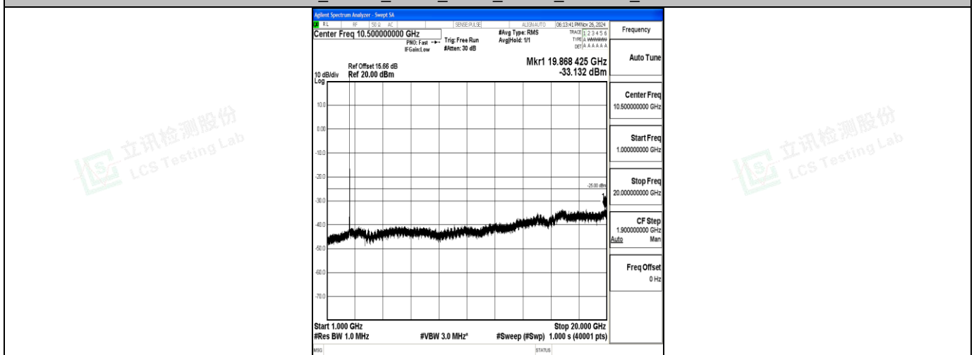
Band7_15MHz_QPSK_21100_1RB#0_1000~20000_1000~20000
