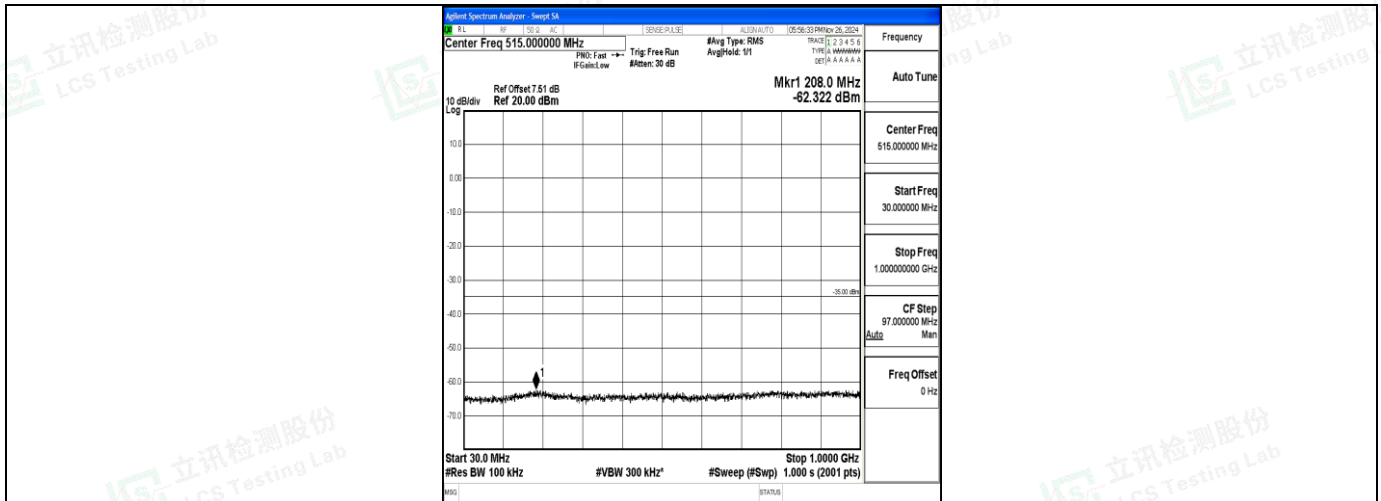
Band7_10MHz_16QAM_21100_1RB#0_30~1000_30~1000
