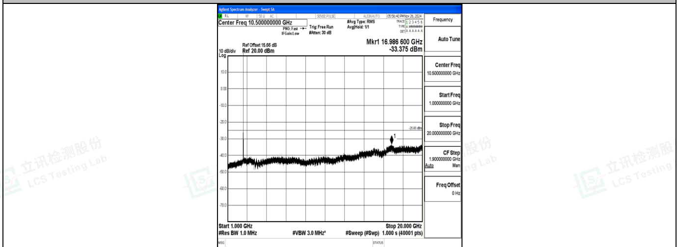
Band7_10MHz_16QAM_21100_1RB#0_1000~20000_1000~20000
