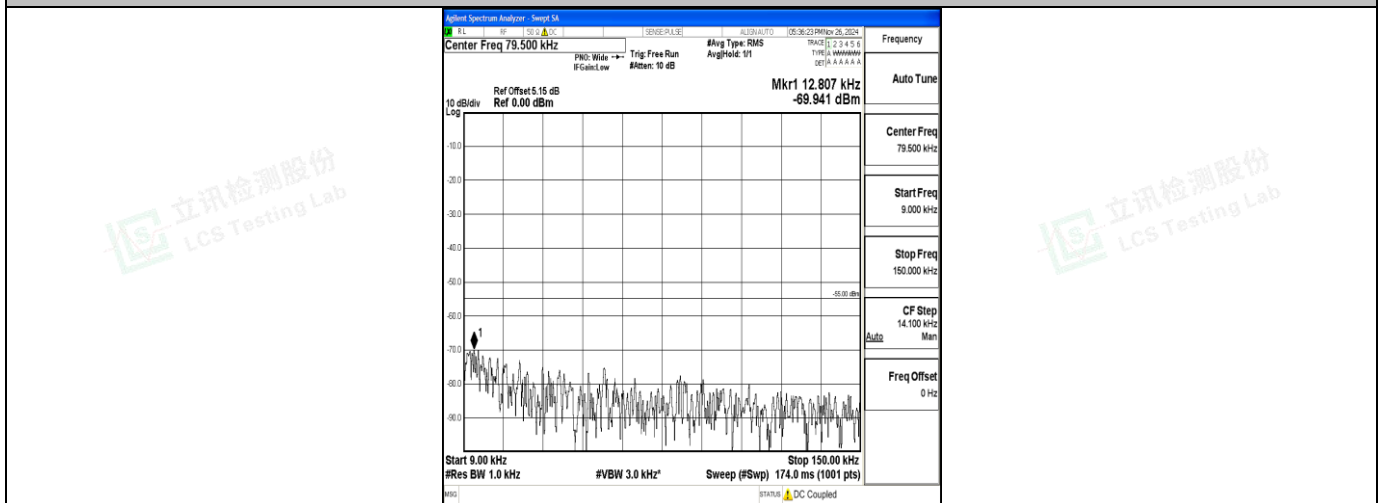
Band7_5MHz_QPSK_21100_1RB#0_0.009~0.15_0.009~0.15
