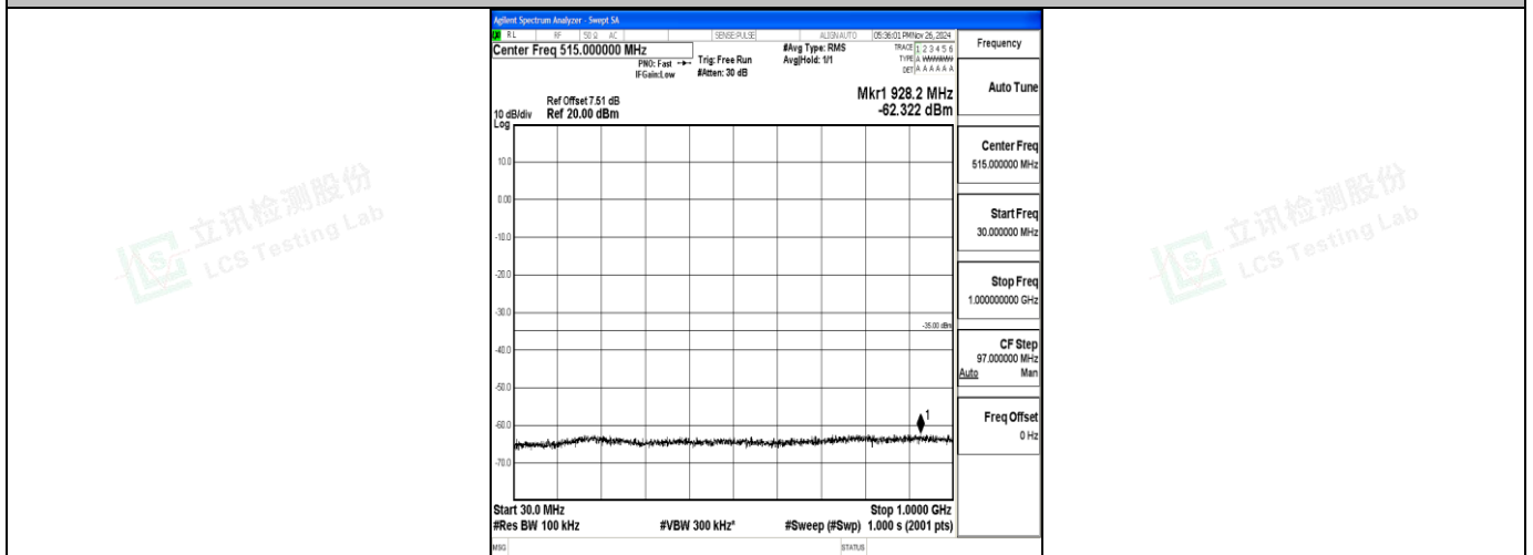
Band7_5MHz_16QAM_20775_1RB#0_30~1000_30~1000
