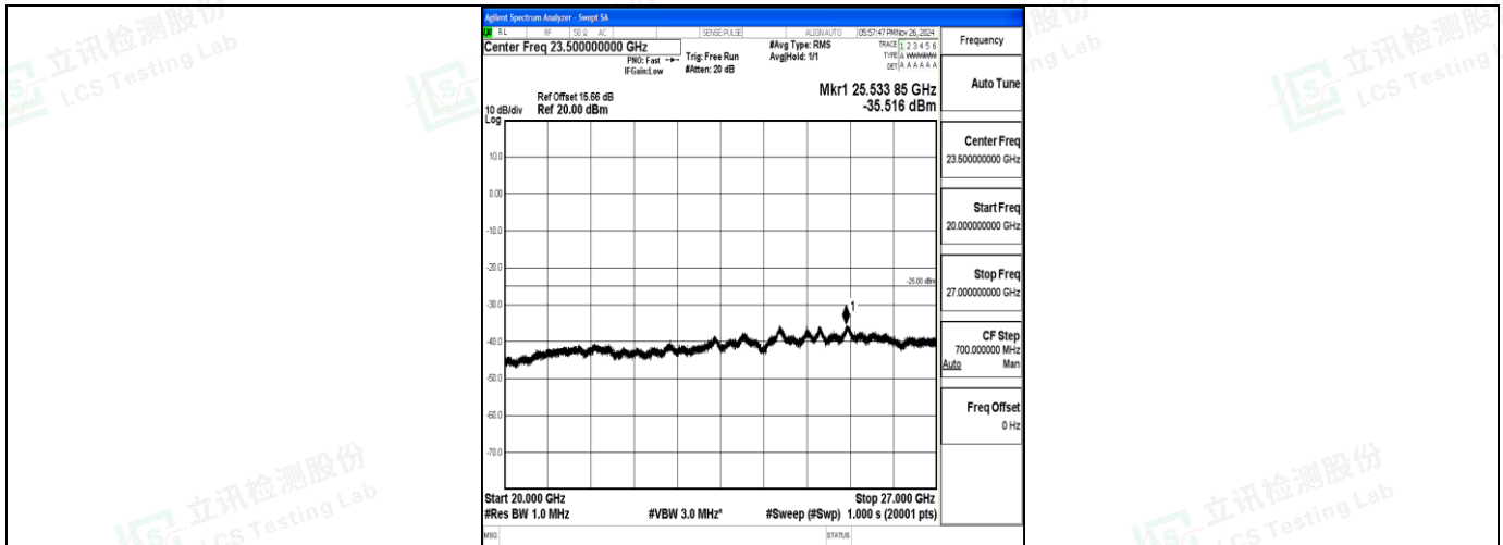
Band7_10MHz_16QAM_21400_1RB#0_20000~27000_20000~27000
