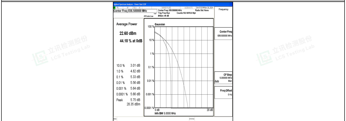
Band5-3MHz-16QAM-20525-1RB#0-PASS
