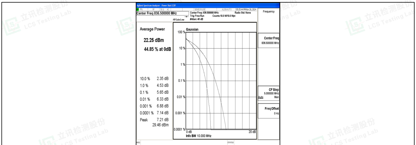
Band5-10MHz-QPSK-20525-50RB#0-PASS
