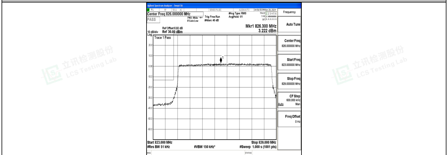
Band5_5MHz_16QAM_20425_25RB#0
