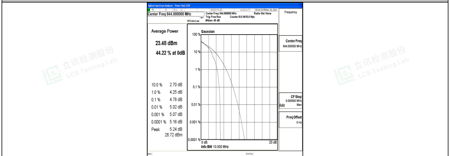
Band5-10MHz-QPSK-20600-1RB#0-PASS
