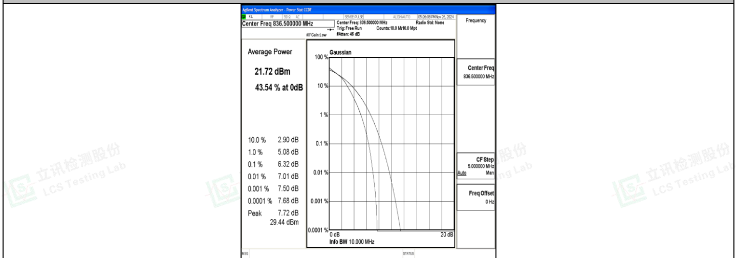
Band5-10MHz-16QAM-20525-50RB#0-PASS
