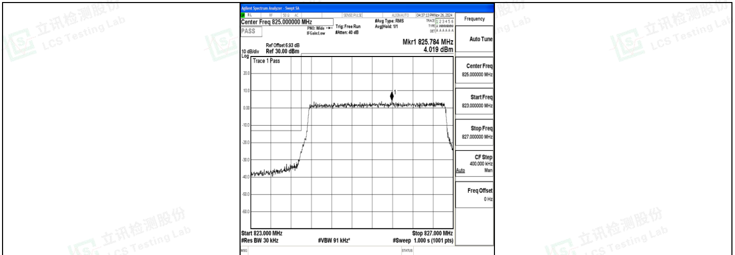
Band5_3MHz_QPSK_20415_15RB#0
