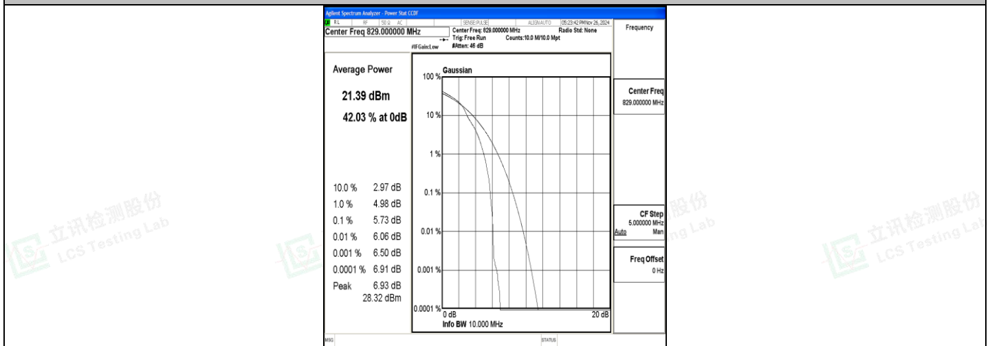
Band5-10MHz-16QAM-20450-1RB#0-PASS
