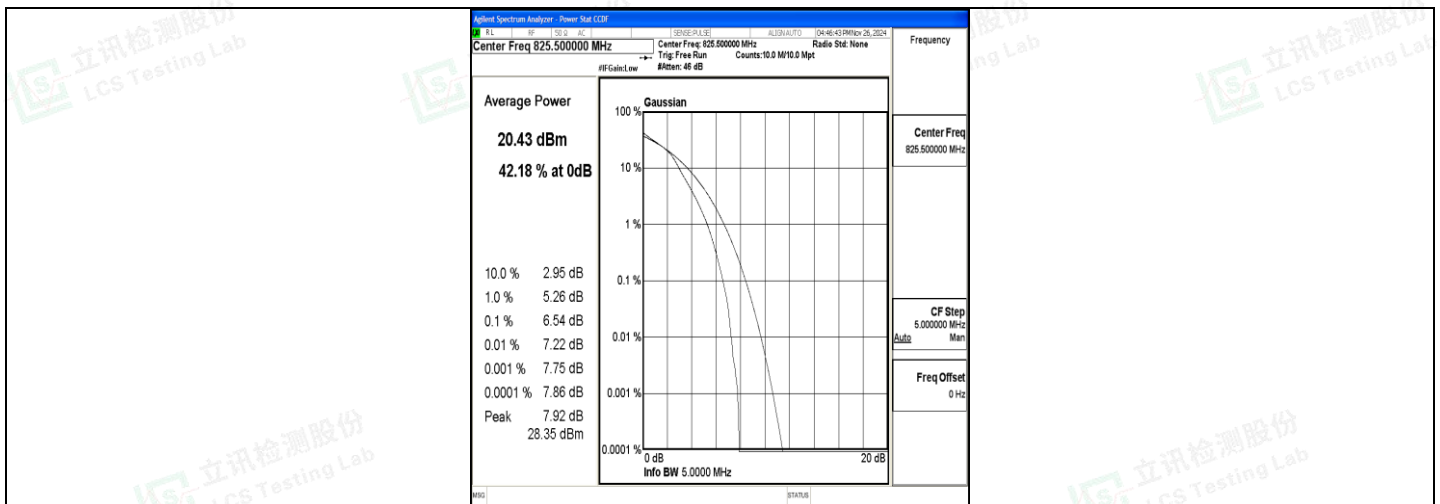
Band5-3MHz-16QAM-20415-15RB#0-PASS
