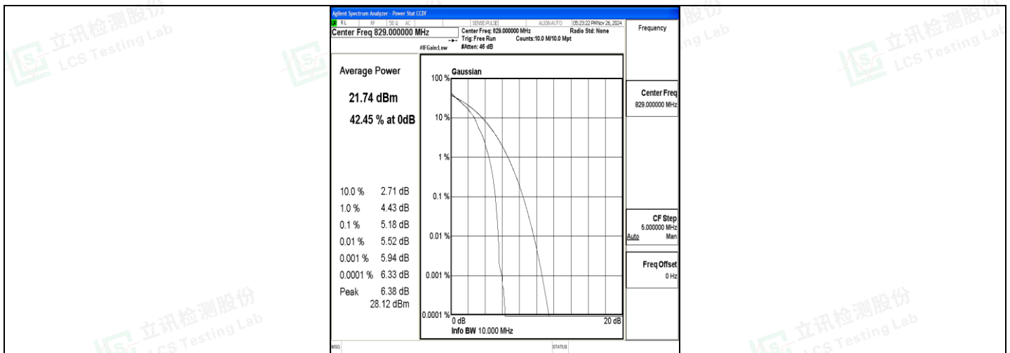
Band5-10MHz-QPSK-20450-1RB#0-PASS
