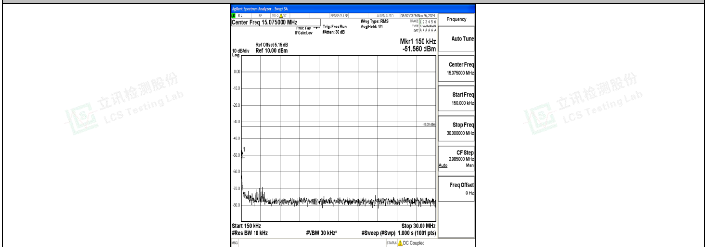
Band4_20MHz_16QAM_20050_1RB#0_0.15~30_0.15~30
