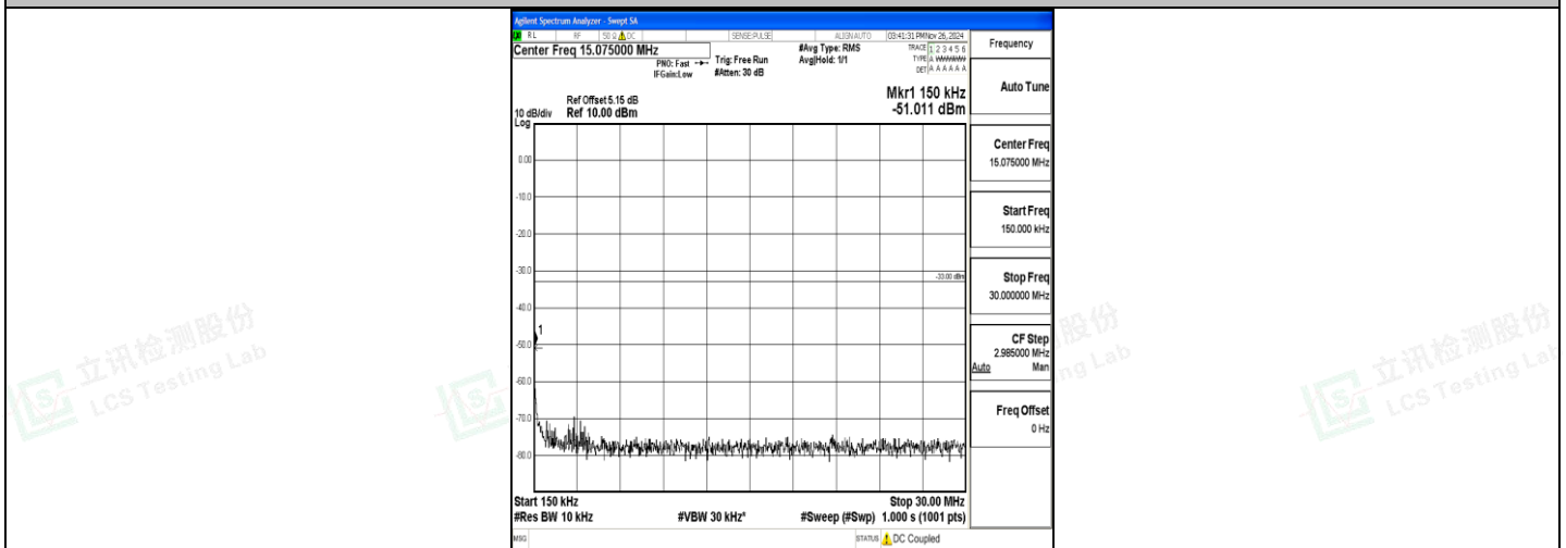
Band4_15MHz_QPSK_20175_1RB#0_0.15~30_0.15~30
