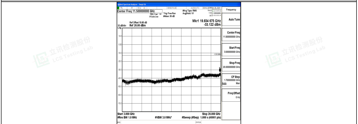
Band4_15MHz_16QAM_20025_1RB#0_3000~20000_3000~20000
