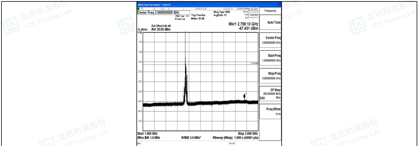
Band4_20MHz_16QAM_20300_1RB#0_1000~3000_1000~3000
