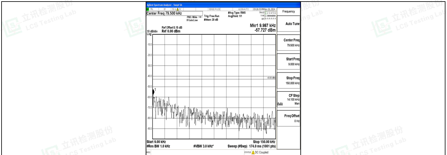
Band4_10MHz_16QAM_20350_1RB#0_0.009~0.15_0.009~0.15
