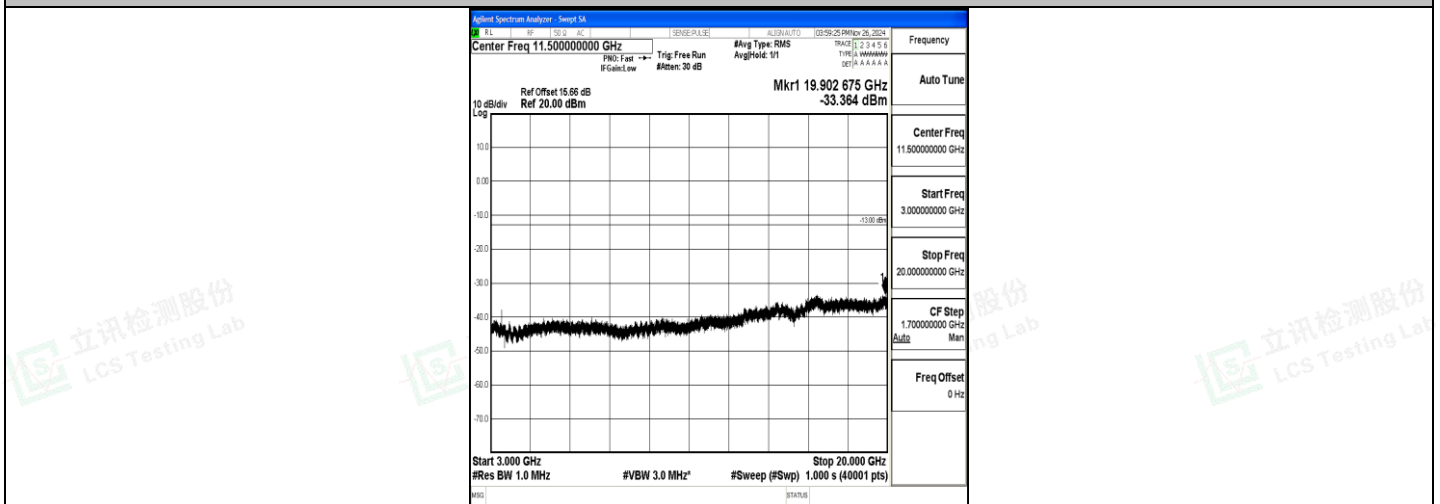
Band4_20MHz_16QAM_20300_1RB#0_3000~20000_3000~20000
