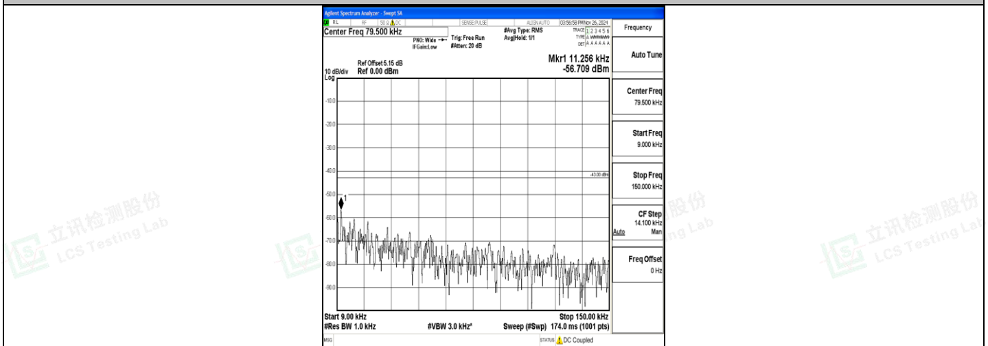
Band4_20MHz_16QAM_20050_1RB#0_0.009~0.15_0.009~0.15
