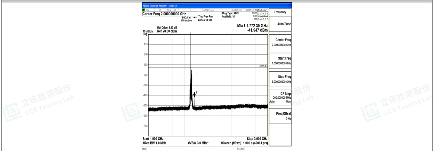
Band4_20MHz_16QAM_20050_1RB#0_1000~3000_1000~3000
