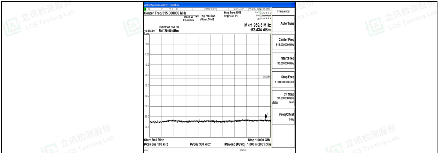
Band4_15MHz_16QAM_20025_1RB#0_30~1000_30~1000
