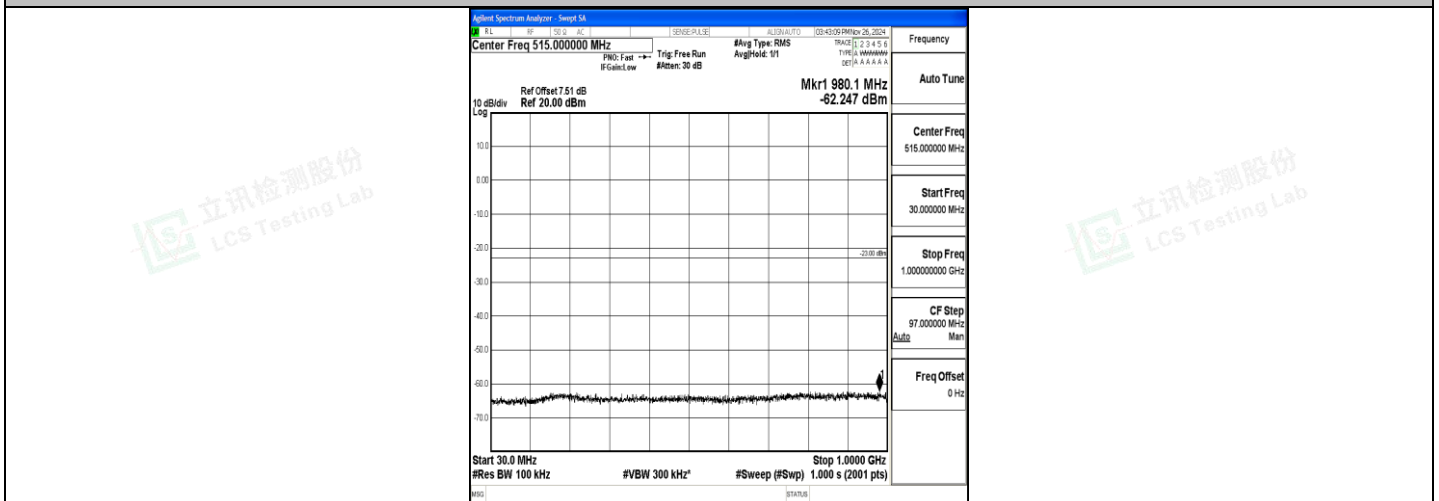
Band4_15MHz_16QAM_20325_1RB#0_30~1000_30~1000
