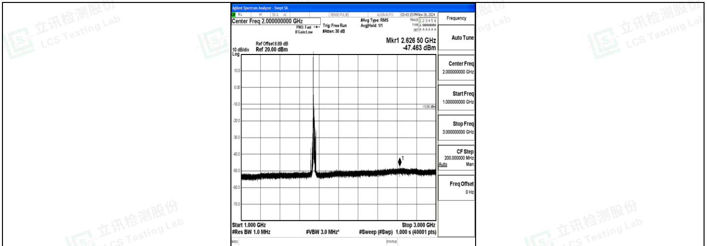
Band4_15MHz_16QAM_20325_1RB#0_1000~3000_1000~3000
