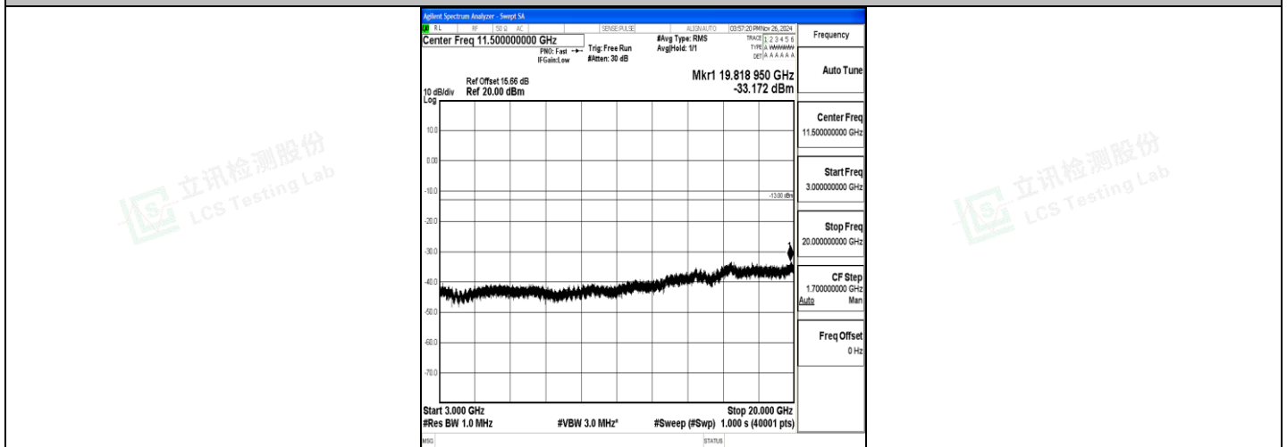
Band4_20MHz_16QAM_20050_1RB#0_3000~20000_3000~20000
