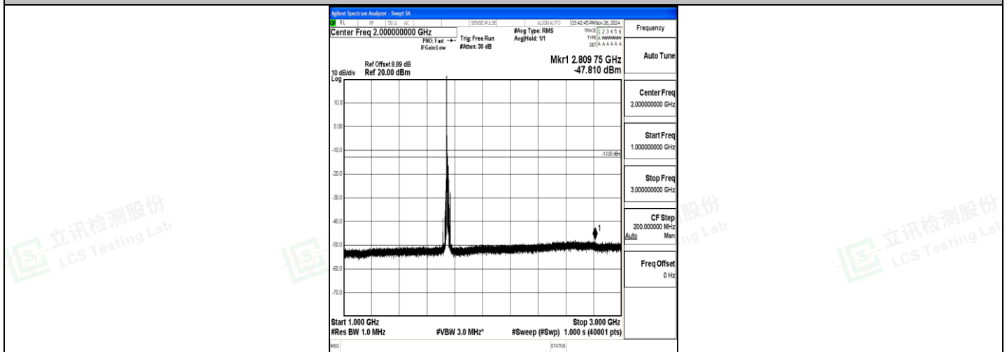
Band4_15MHz_QPSK_20325_1RB#0_1000~3000_1000~3000
