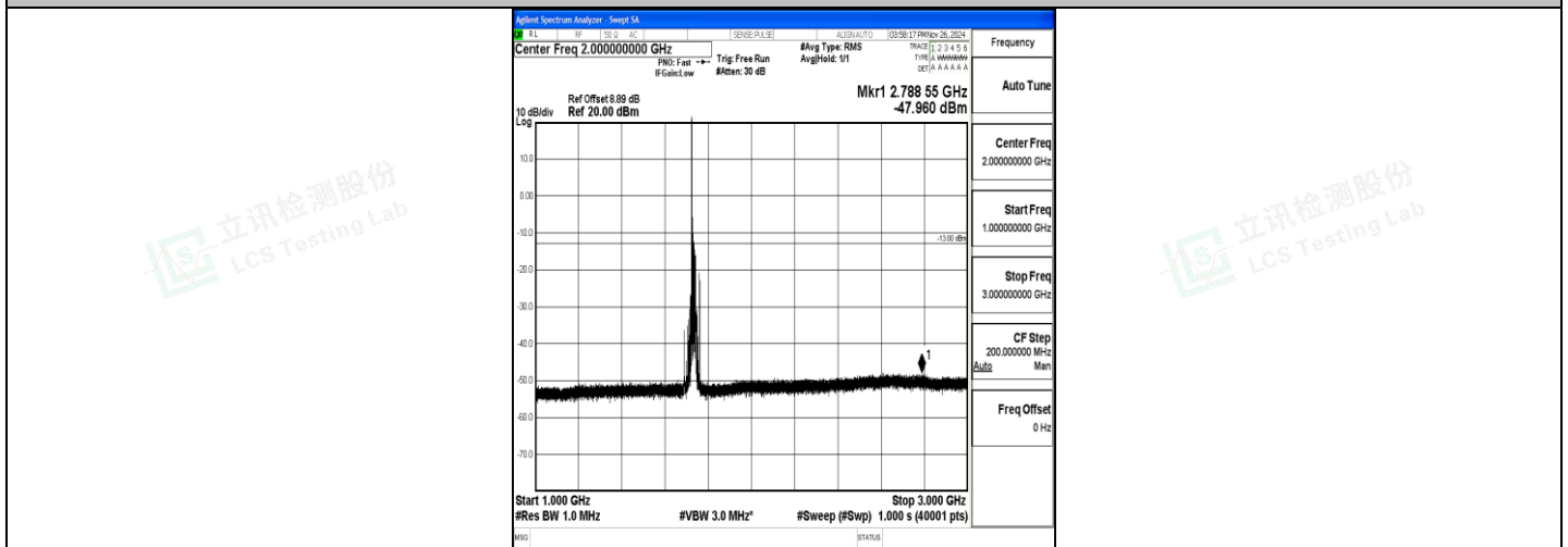
Band4_20MHz_16QAM_20175_1RB#0_1000~3000_1000~3000
