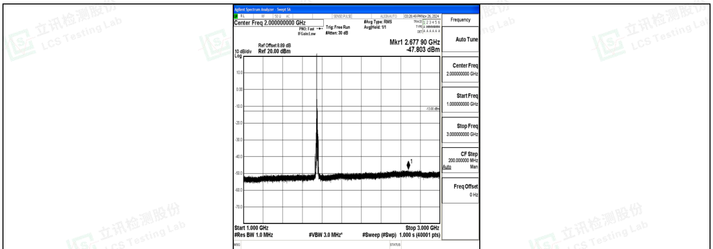
Band4_10MHz_16QAM_20350_1RB#0_1000~3000_1000~3000
