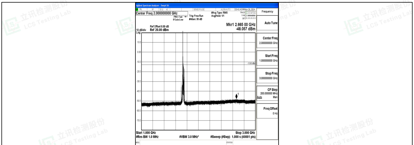
Band4_15MHz_QPSK_20175_1RB#0_1000~3000_1000~3000
