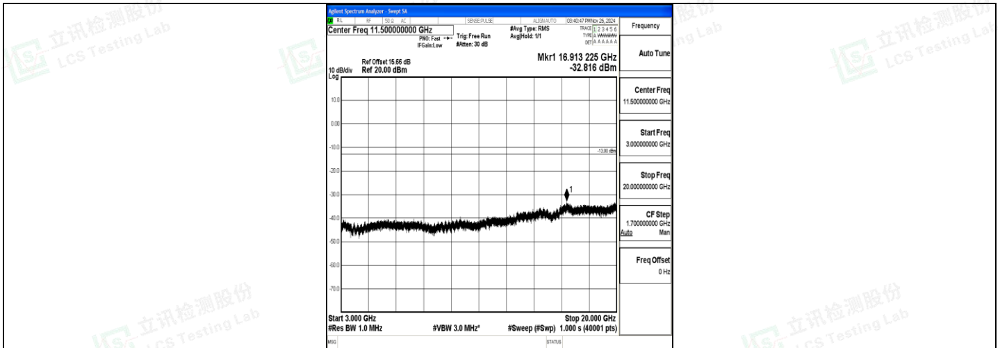
Band4_15MHz_QPSK_20025_1RB#0_3000~20000_3000~20000
