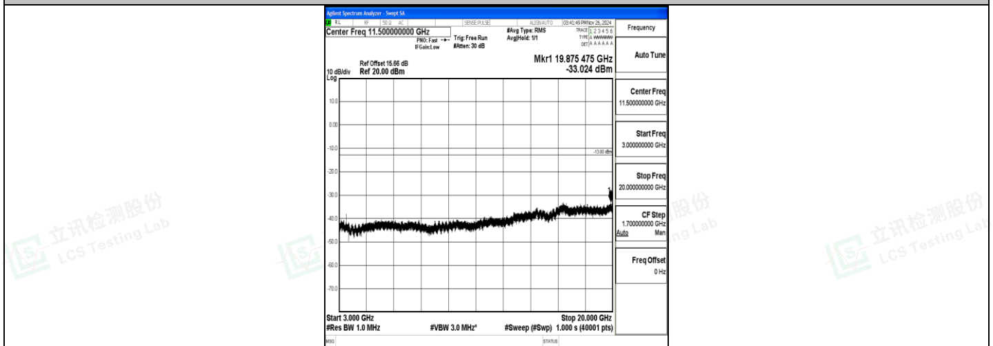
Band4_15MHz_QPSK_20175_1RB#0_3000~20000_3000~20000
