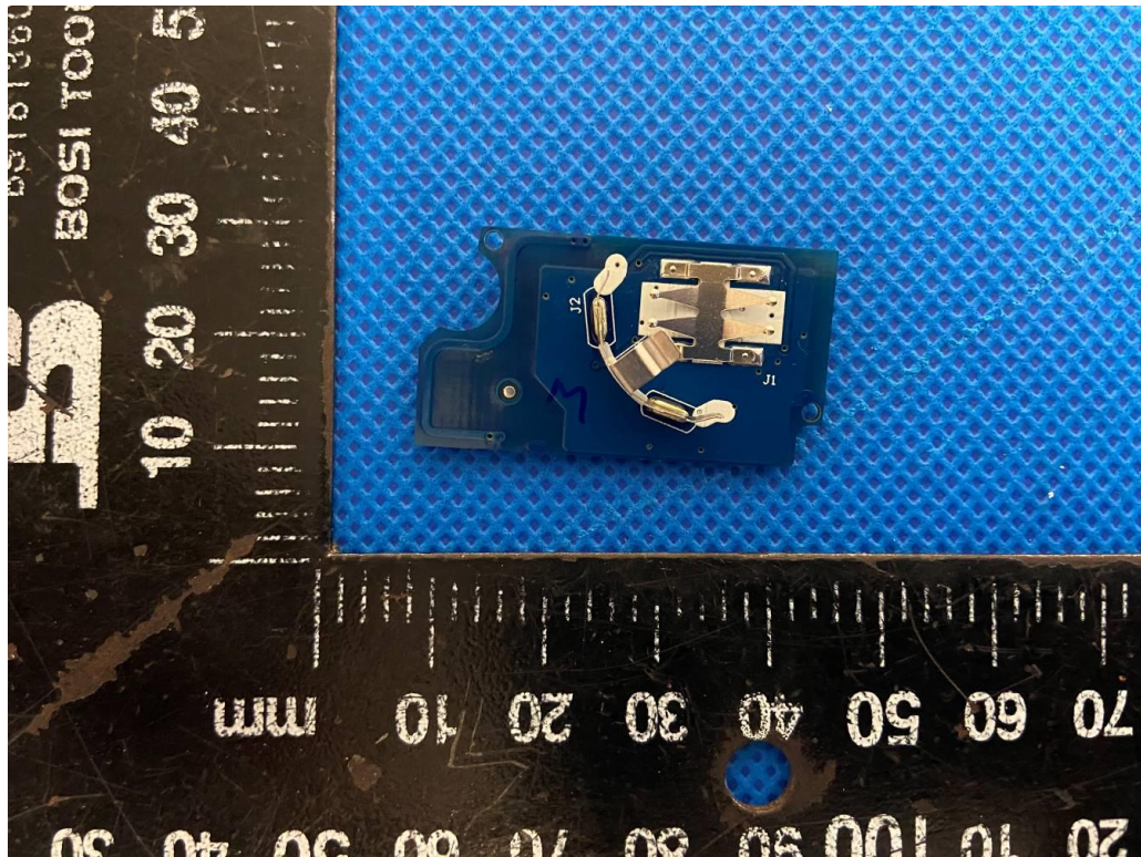
PCB view-1
