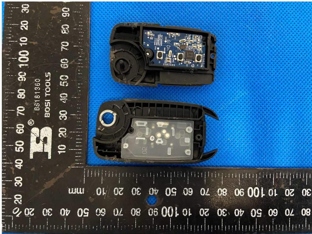
Internal view-1
