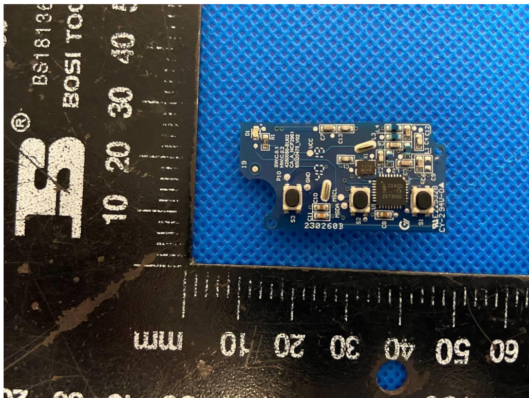
PCB view -2
