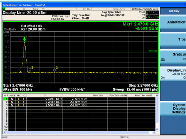
No-hopping mode
