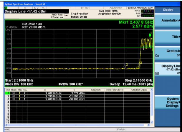
Hopping mode
