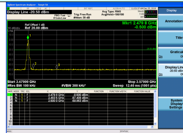
No-hopping mode
