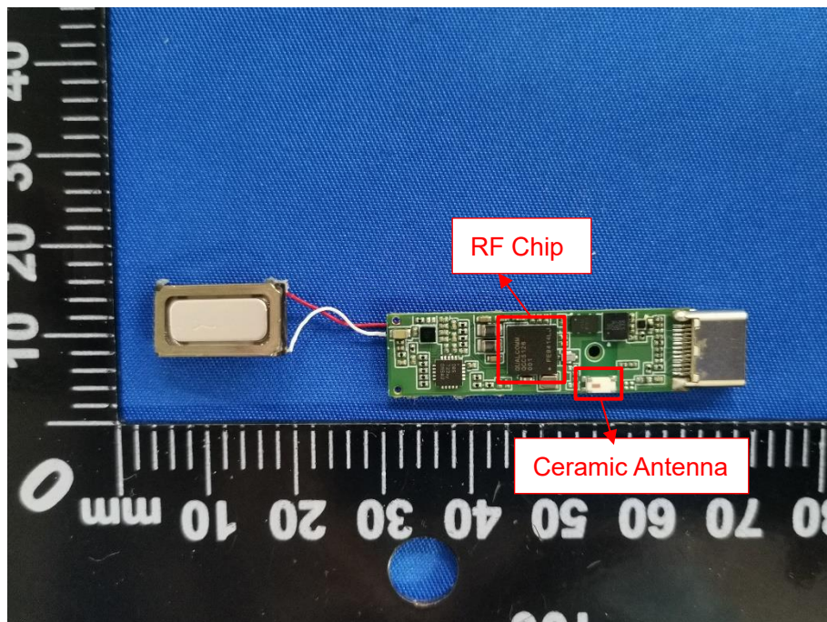
FCC ID: 2AVSDTPM-S003 BOARD TOP VIEW
