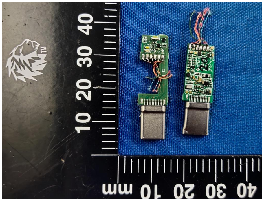
FCC ID: 2AVSDTPM-S00V BOARD REAR VIEW
