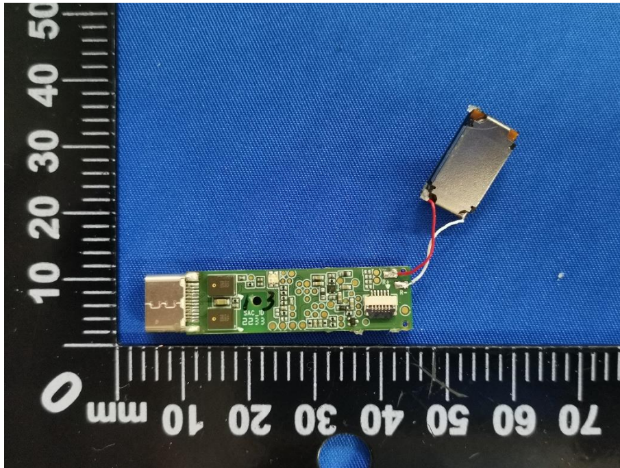
FCC ID: 2AVSDTPM-S003 BOARD REAR VIEW
