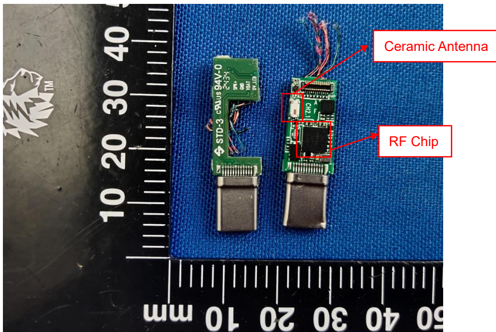
FCC ID: 2AVSDTPM-S00V BOARD TOP VIEW
