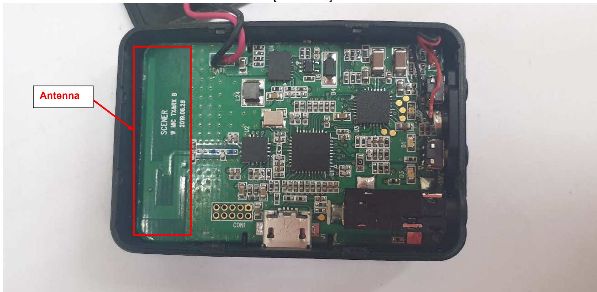
[PCB Antenna]
