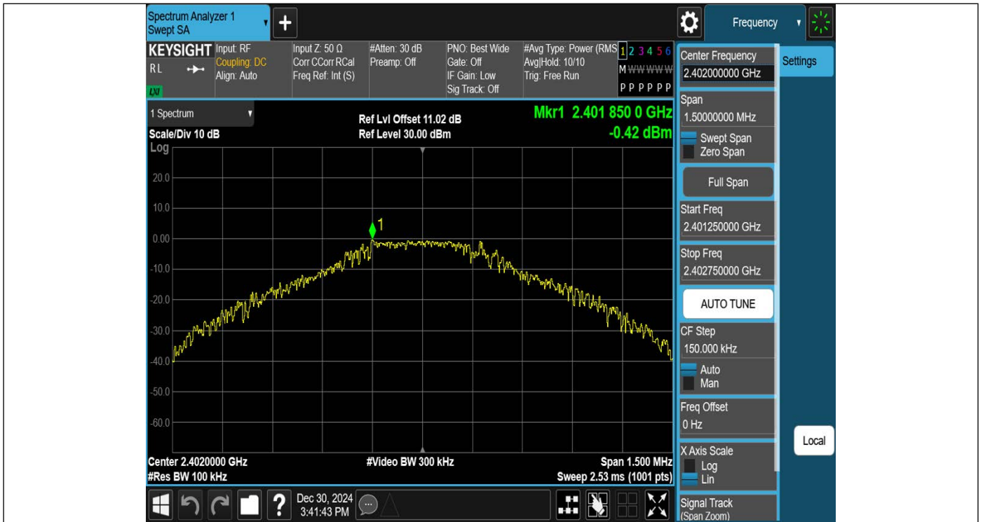
DH5-Ant1-2402-0~Reference-PASS
