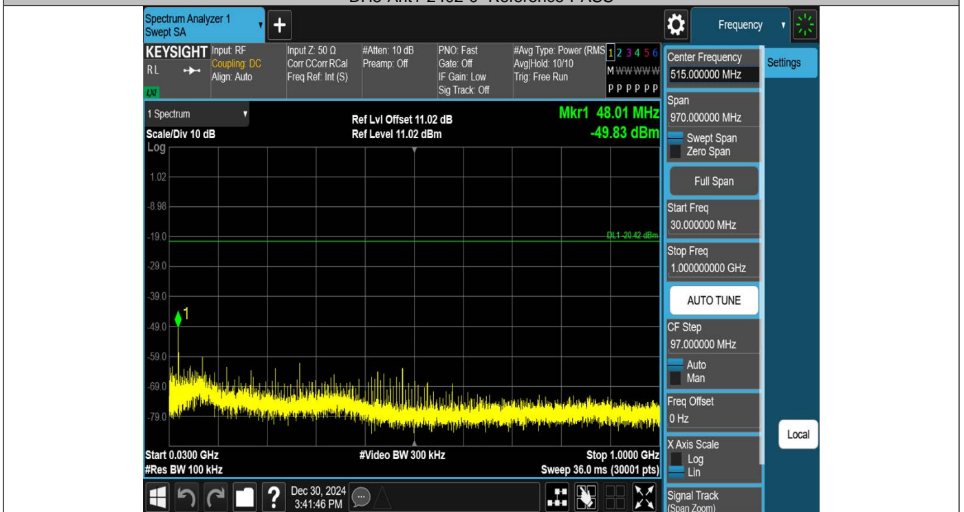
DH5-Ant1-2402-30~1000-PASS
