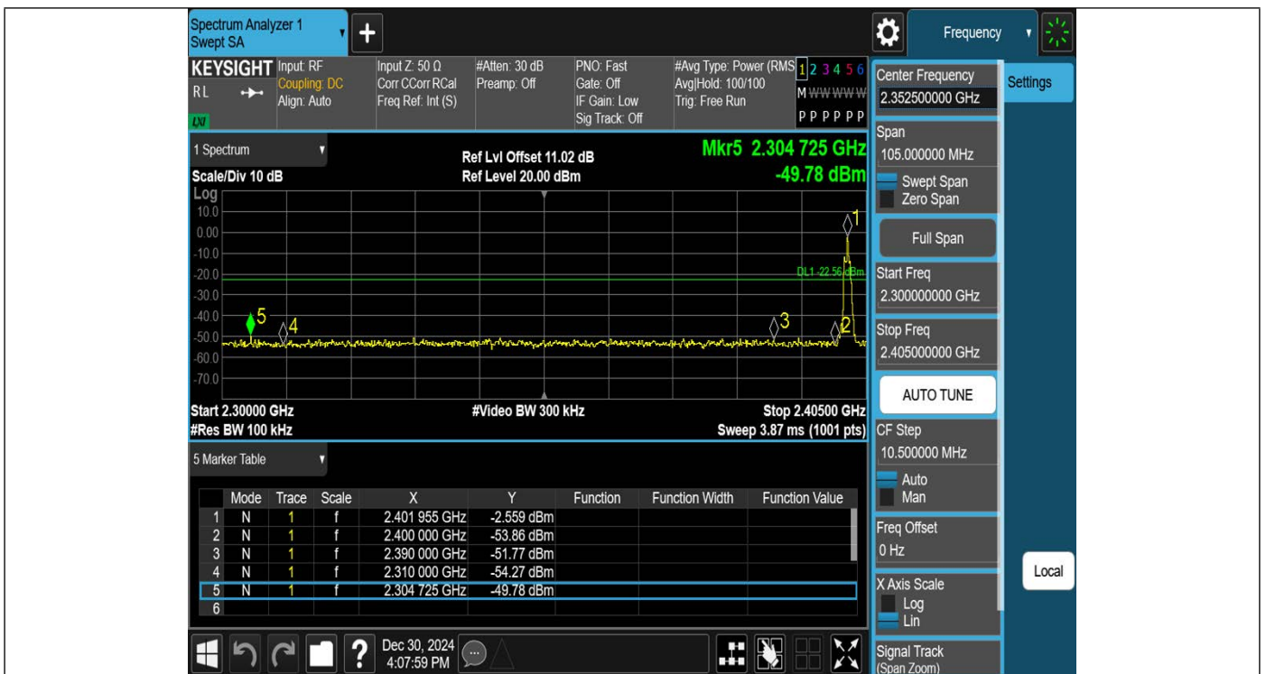
3DH5-Ant1-2402-PASS
