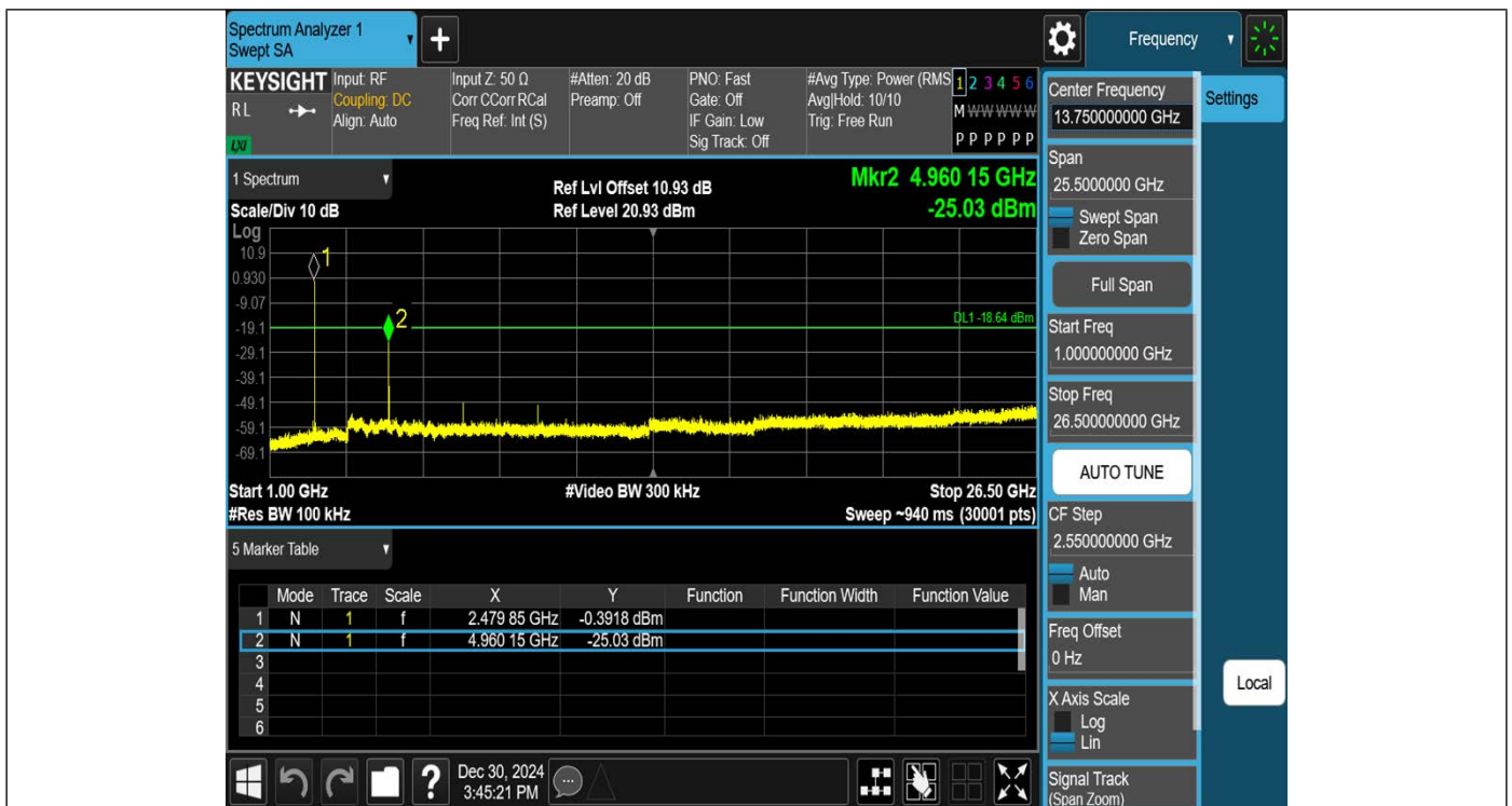
DH5-Ant1-2480-1000~26500-PASS
