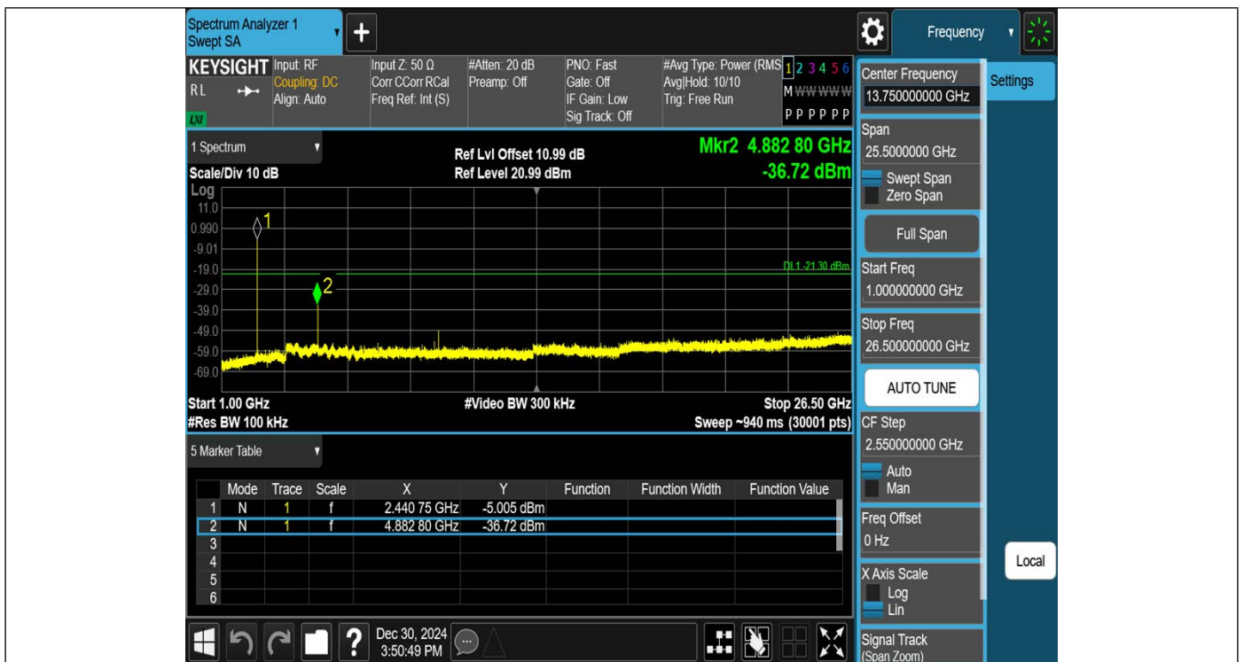
2DH5-Ant1-2441-1000~26500-PASS
