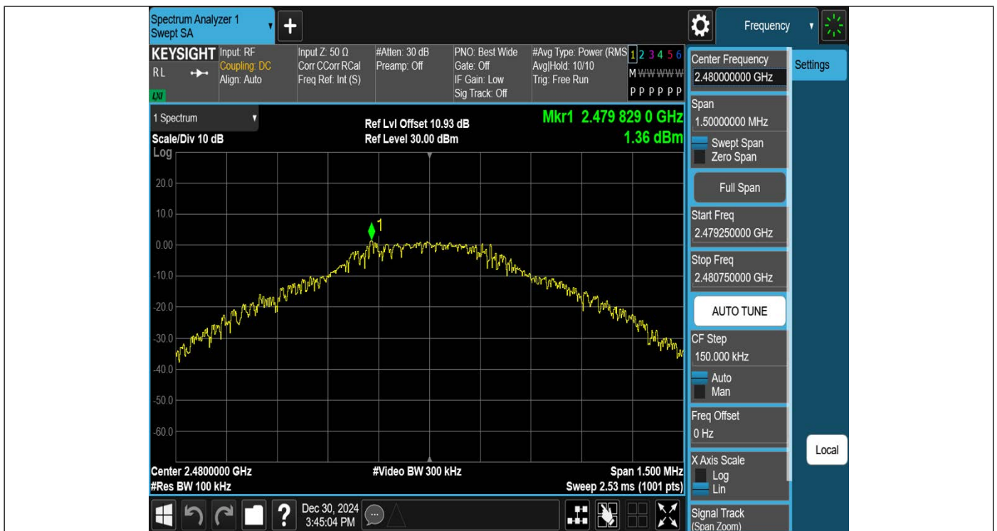
DH5-Ant1-2480-0~Reference-PASS
