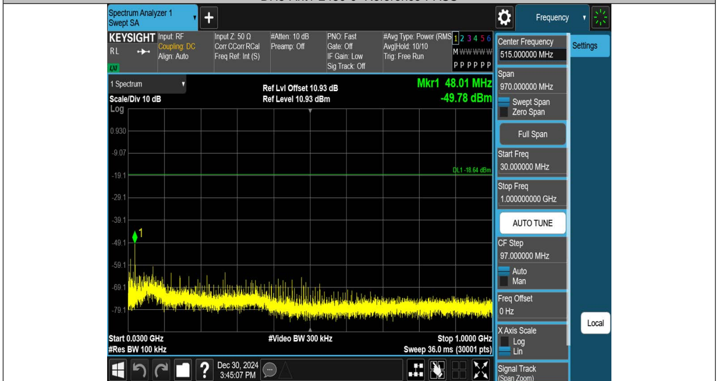
DH5-Ant1-2480-30~1000-PASS
