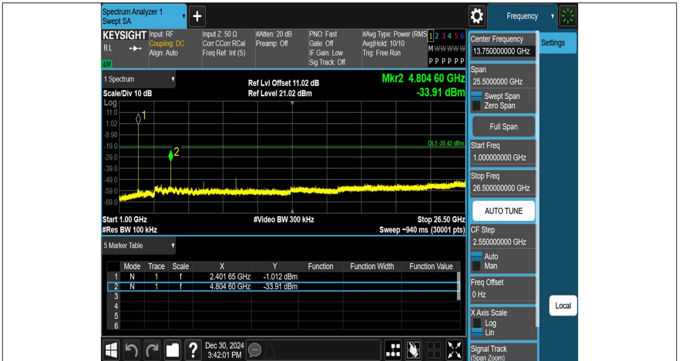
DH5-Ant1-2402-1000~26500-PASS
