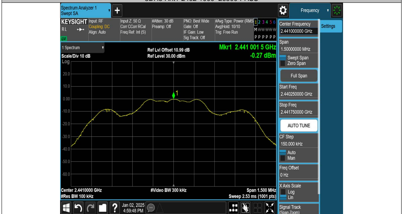
3DH5-Ant1-2441-0~Reference-PASS
