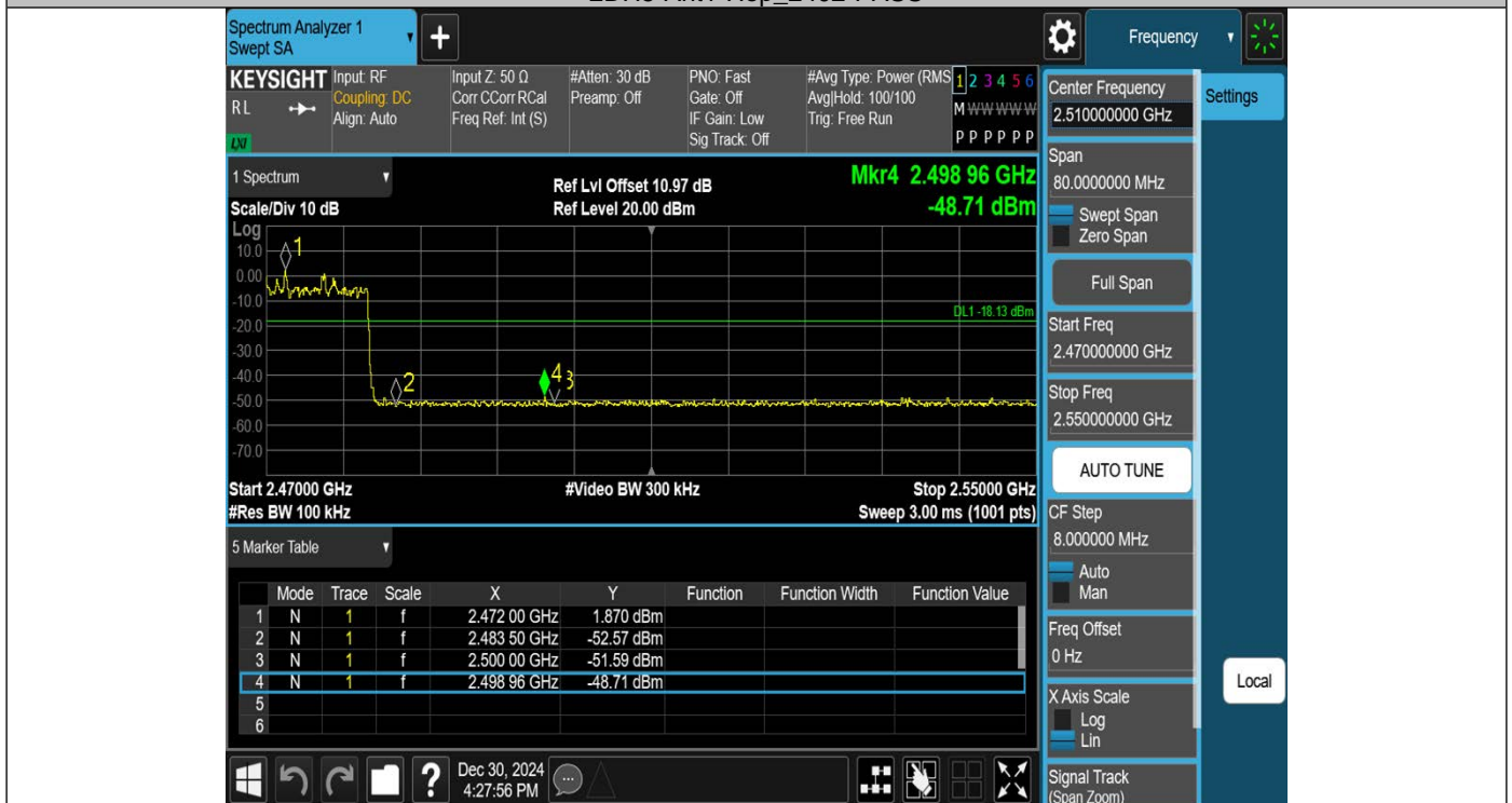
2DH5-Ant1-Hop_2480-PASS
