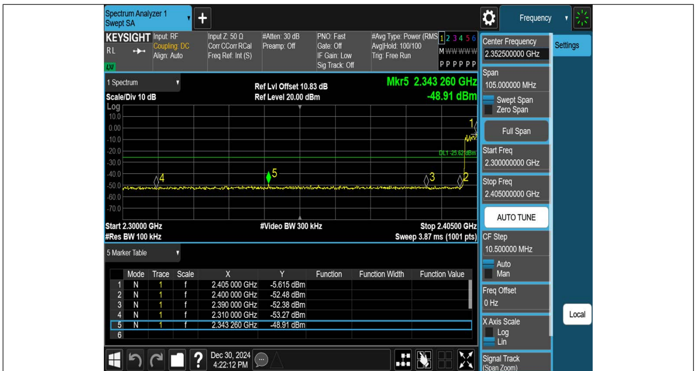
2DH5-Ant1-Hop_2402-PASS
