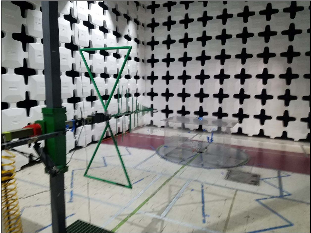
REE 30MHz - 1GHz Setup
