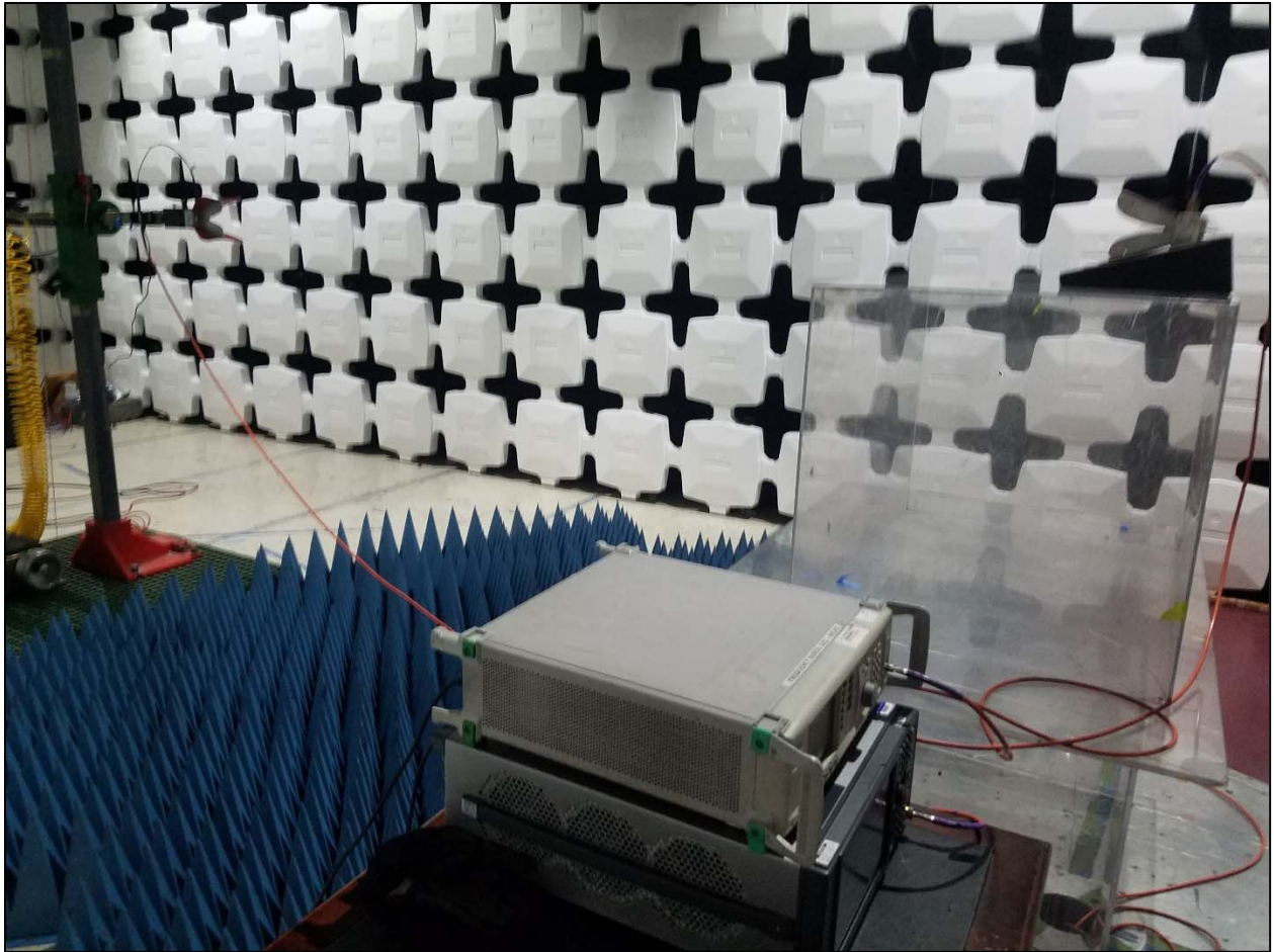
RSE Substitution Method Setup
