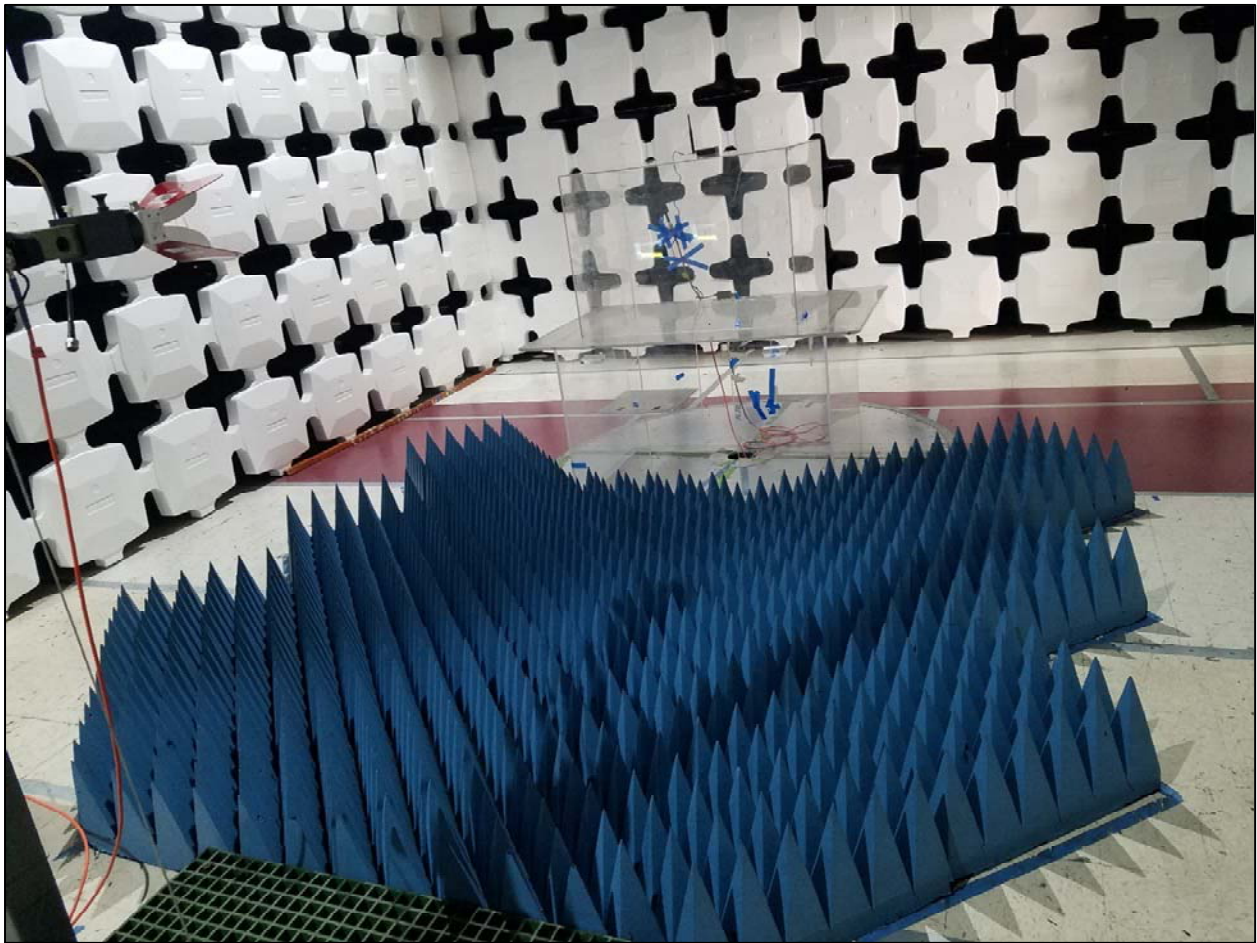
RSE Above 1GHz Setup
