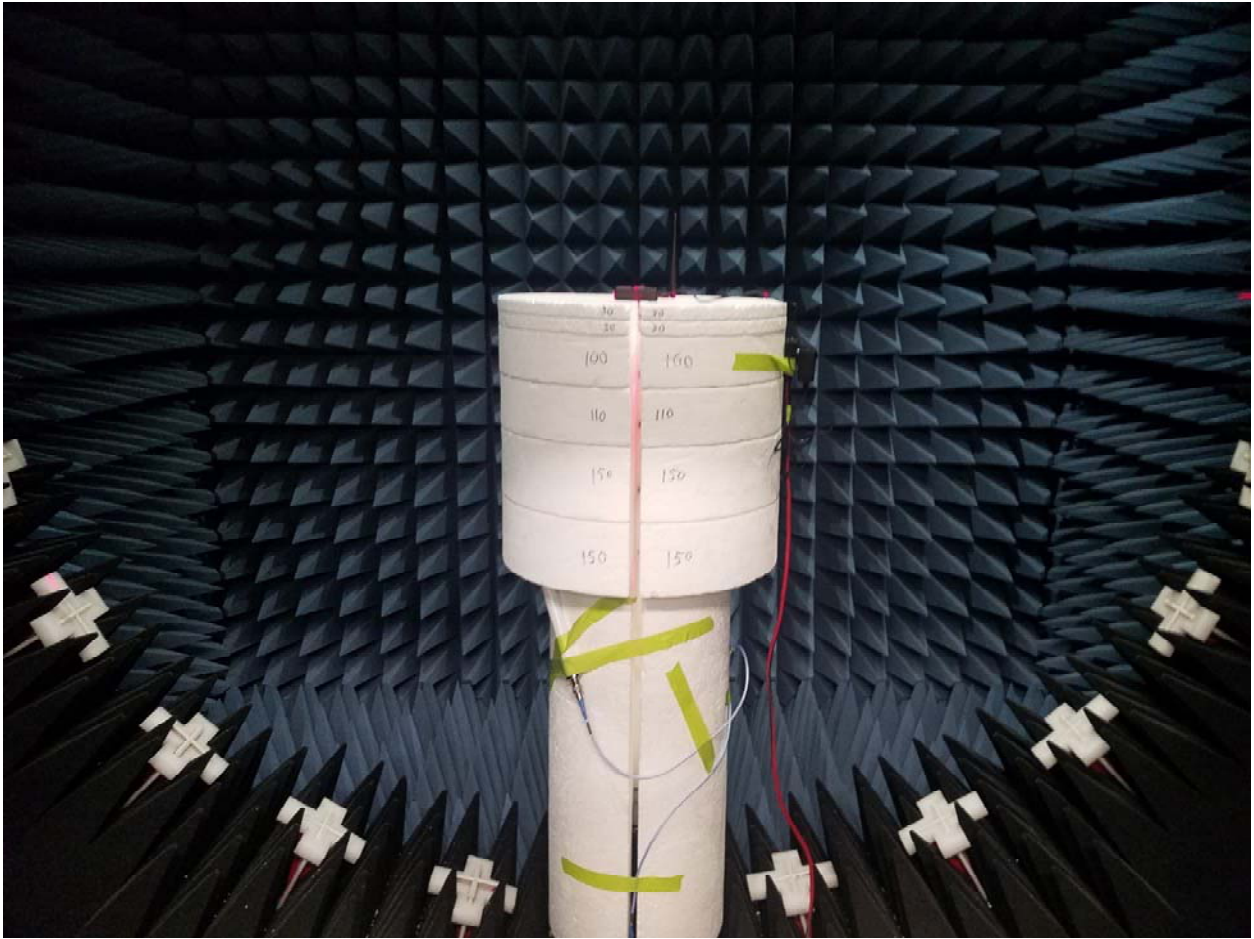
OTA Setup 1
