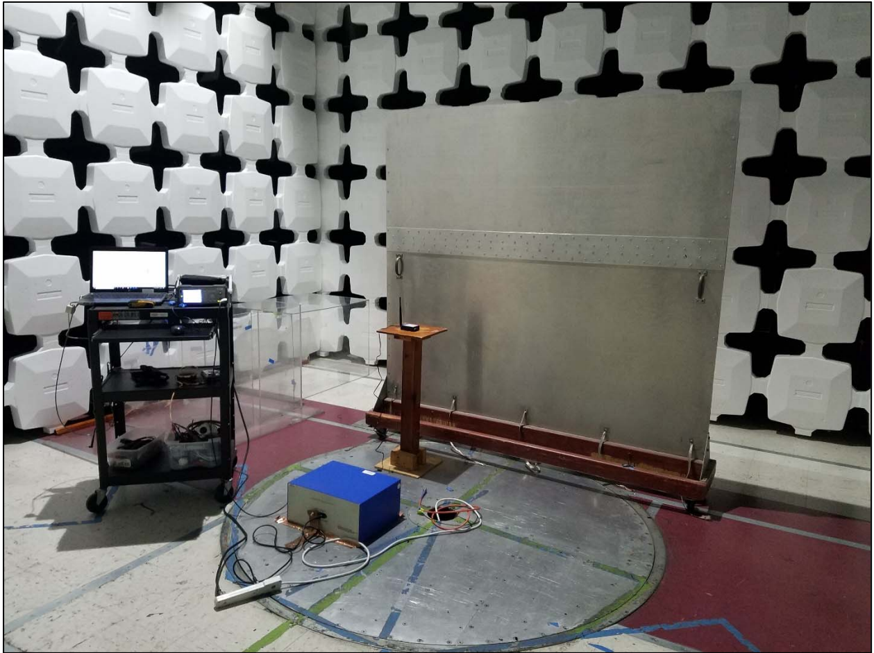
CEV Setup
