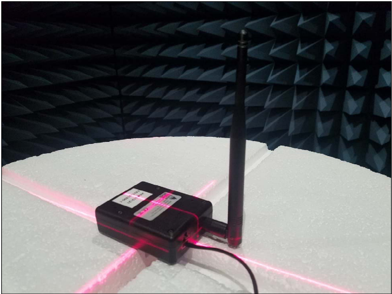
OTA Setup 2
