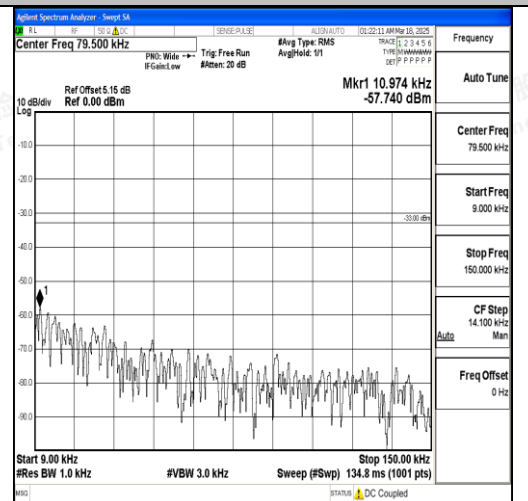
Band12_1.4MHz_16QAM_23095_1RB#0_0.009~0.15_0.009~0.15
