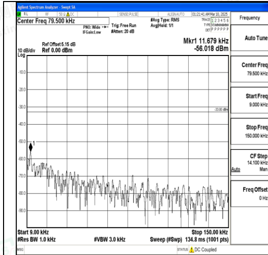
Band12_1.4MHz_QPSK_23095_1RB#0_0.009~0.15_0.009~0.15
