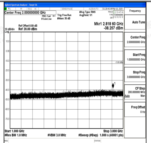
Band12_5MHz_QPSK_23035_1RB#0_1000~3000_1000~3000
