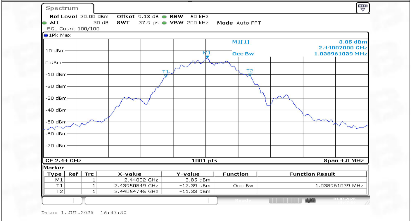
BLE_1M-Ant1-2440
