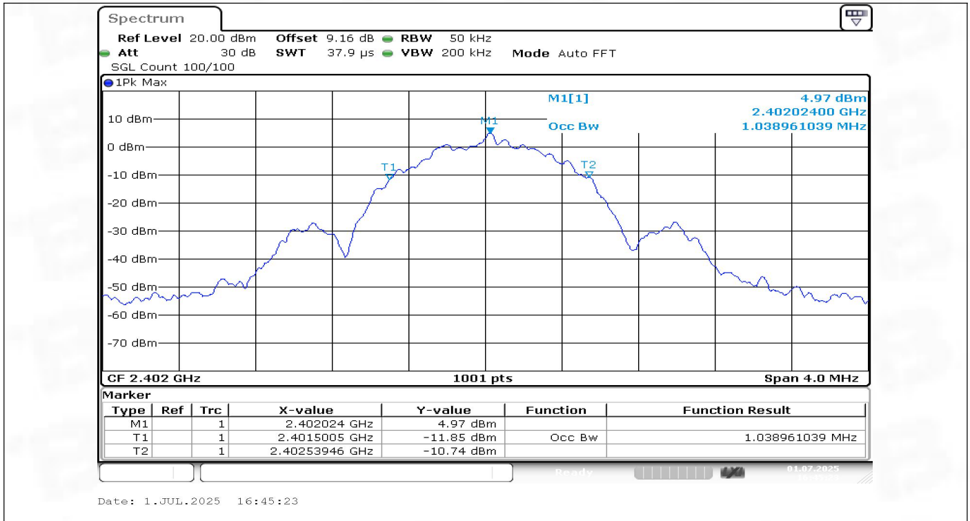
BLE_1M-Ant1-2402
