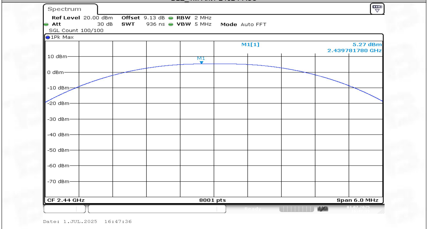
BLE_1M-Ant1-2440-PASS
