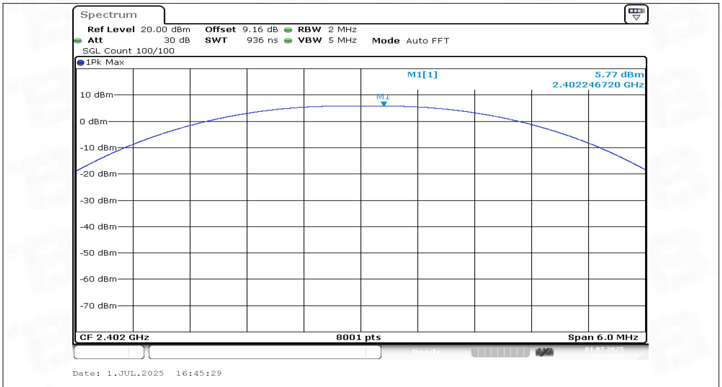
BLE_1M-Ant1-2402-PASS
