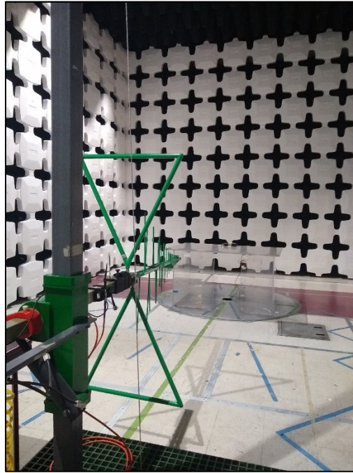
Photograph 1: Radiated Spurious Emissions, Below 1GHz, Test Setup
