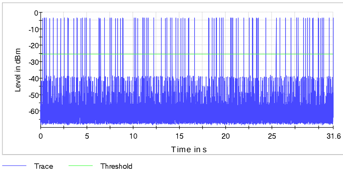
Time of Channel Occupancy(3)
