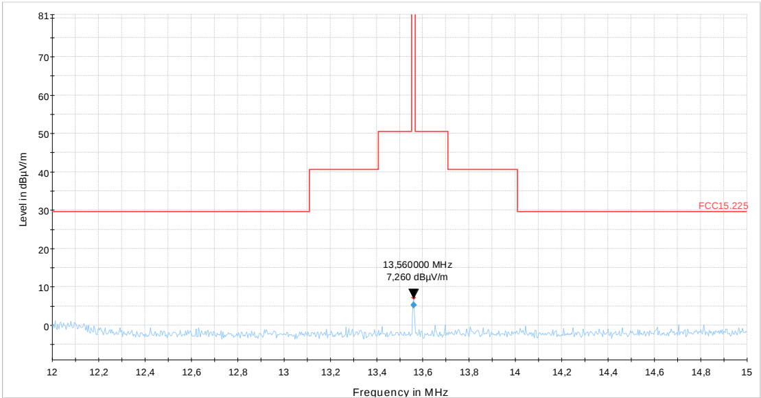
Diagram 2: EUT lying
