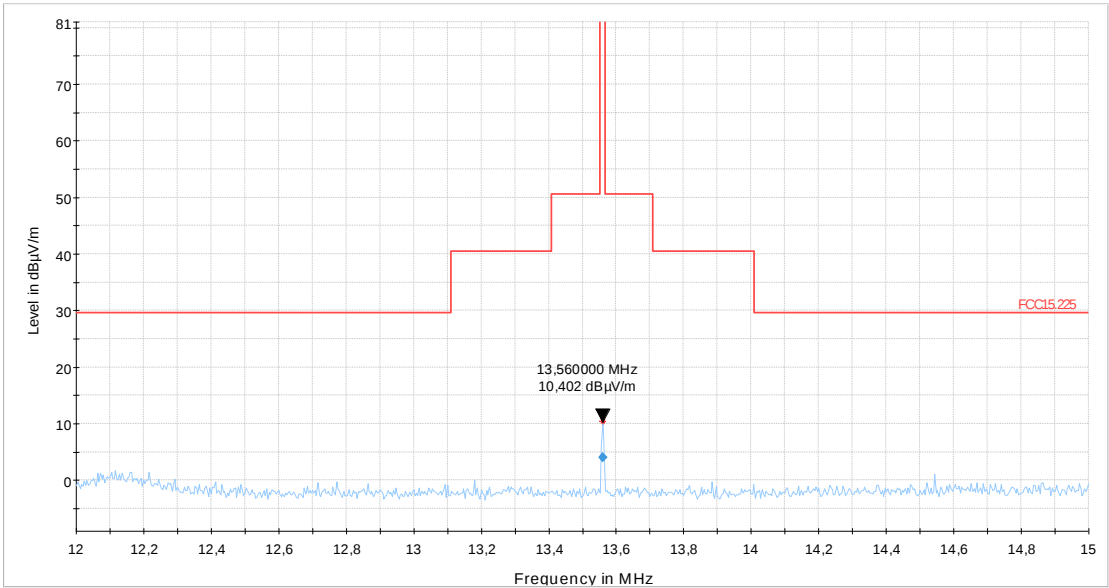
Diagram 3: EUT standing
