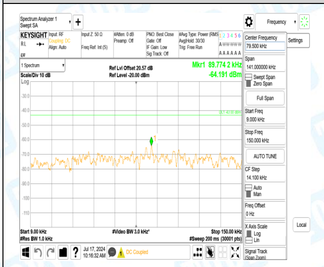
Band4-15MHz-QPSK-20325-1-0-High-0.009-0.15-0.09--64.19-21.19--43-PASS
