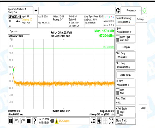
Band4-15MHz-QPSK-20325-1-0-High-0.15-30-0.16--67.2-34.2--33-PASS
