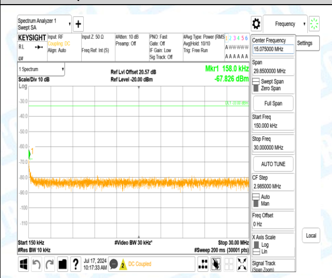
Band4-15MHz-16QAM-20325-1-0-High-0.15-30-0.16--67.83-34.83--33-PASS
