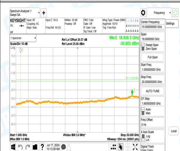
Band4-15MHz-QPSK-20025-1-0-Low-1000-20000-18938.53--30.6-17.6--13-PASS
