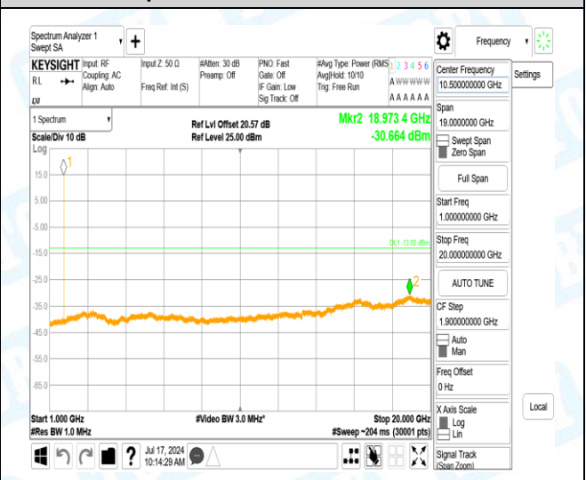
Band4-15MHz-16QAM-20025-1-0-Low-1000-20000-18973.37--30.66-17.66--13-PASS
