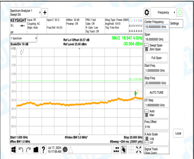
Band4-15MHz-QPSK-20325-1-0-High-1000-20000-18947.4--30.5-17.5--13-PASS
