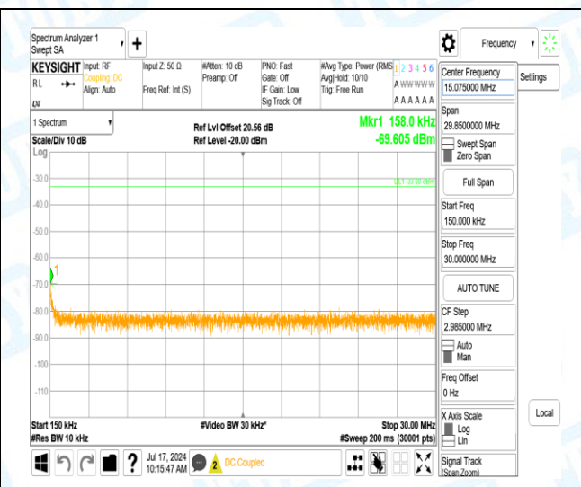
Band4:15MHz-16OAM-20175-1-0-Low-0.15-30-0.16--69.61-36.61--33-PASS
