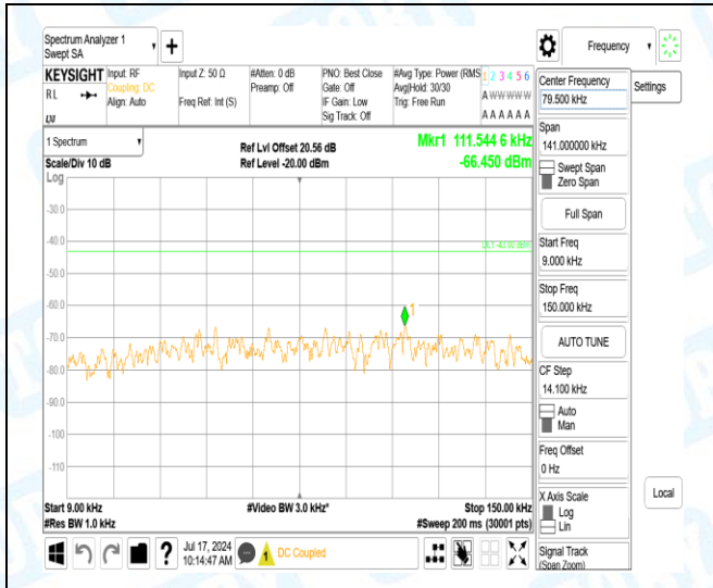
Band4-15MHz-QPSK-20175-1-0-Low-0.009-0.15-0.11--66.45-23.45--43-PASS
