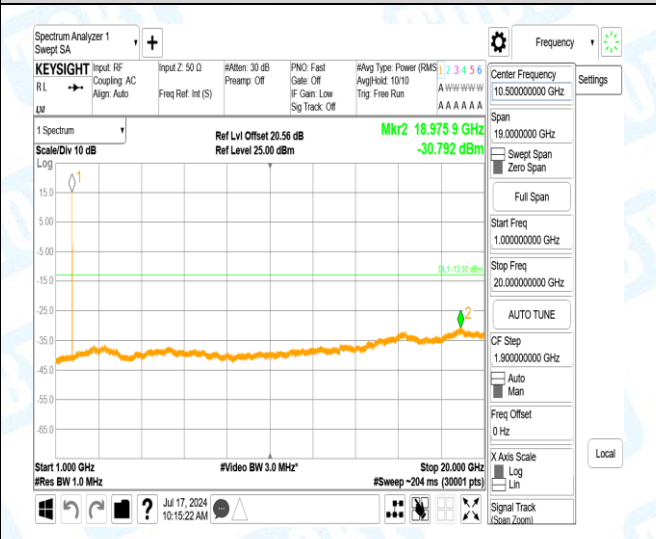
Band4-15MHz-QPSK-20175-1-0-Low-1000-20000-18975.9--30.79-17.79--13-PASS
