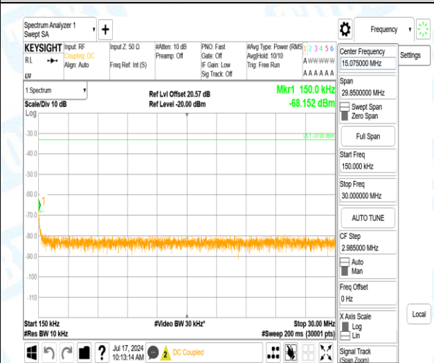
Band4-15MHz-QPSK-20025-1-0-Low-0.15-30-0.15--68.15-35.15--33-PASS
