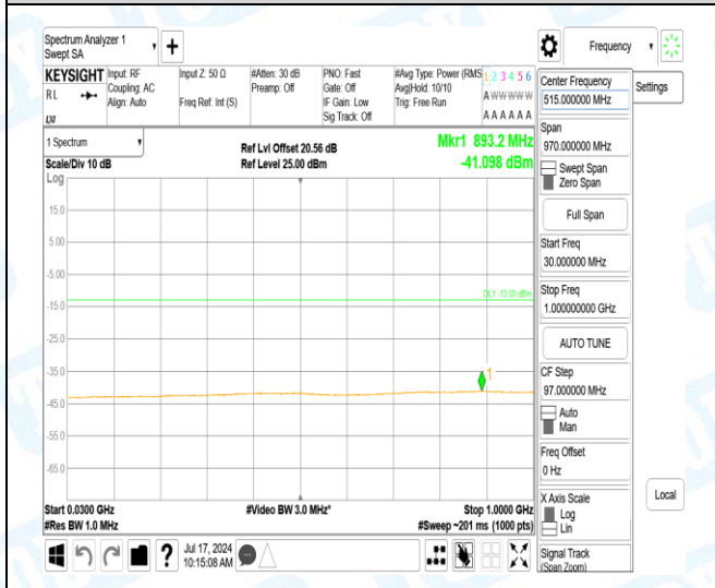
Band4-15MHz-QPSK-20175-1-0-Low-30-1000-893.19--41.1-28.1--13-PASS
