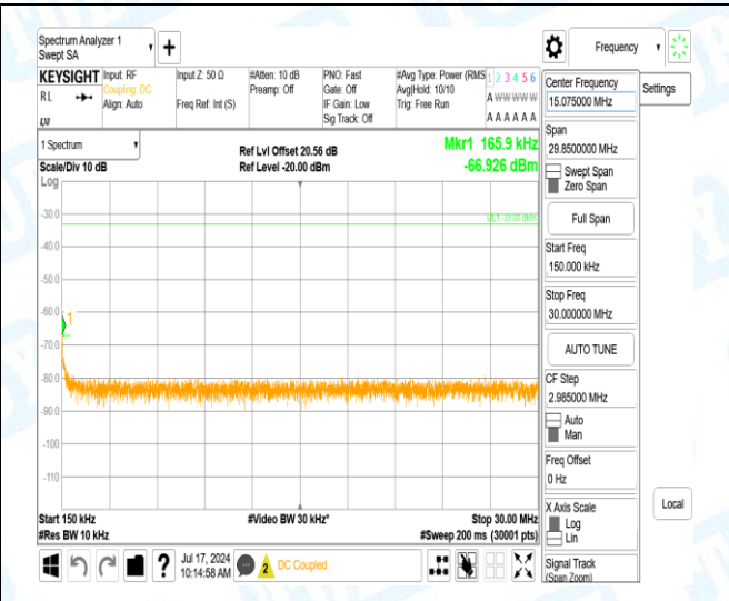
Band4-15MHz-QPSK-20175-1-0-Low-0.15-30-0.17--66.93-33.93--33-PASS
