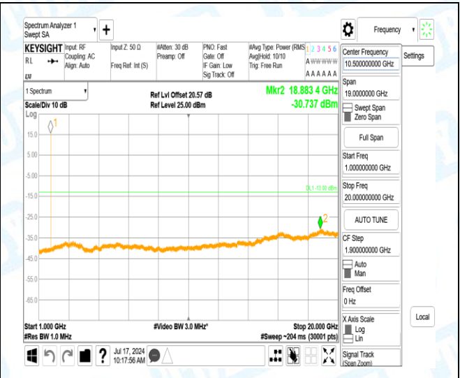
Band4-15MHz-16QAM-20325-1-0-High-1000-20000-18883.43--30.74-17.74--13-PASS
