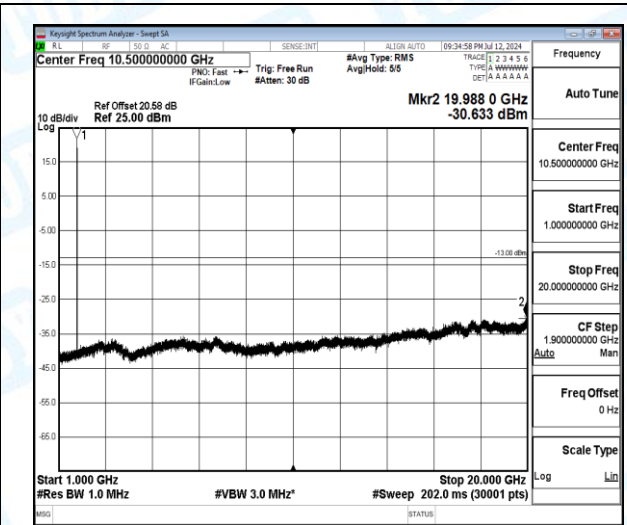
Band4-10MHz-16QAM-20350-1-0-High-1000-20000-19987.97--30.63-17.63--13-PASS
