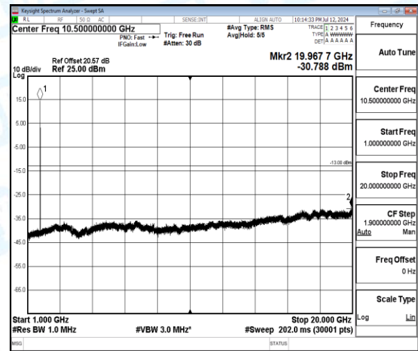
Band4-20MHz-QPSK-20300-1-0-High-1000-20000-19967.7--30.79-17.79--13-PASS
