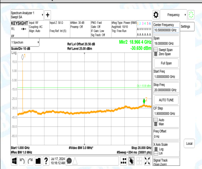
Band4-15MHz-16QAM-20175-1-0-Low-1000-20000-18966.4--30.65-17.65--13-PASS
