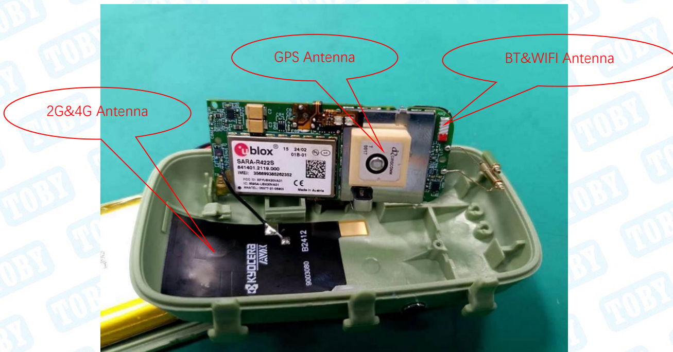
Photo 12 Internal of EUT
