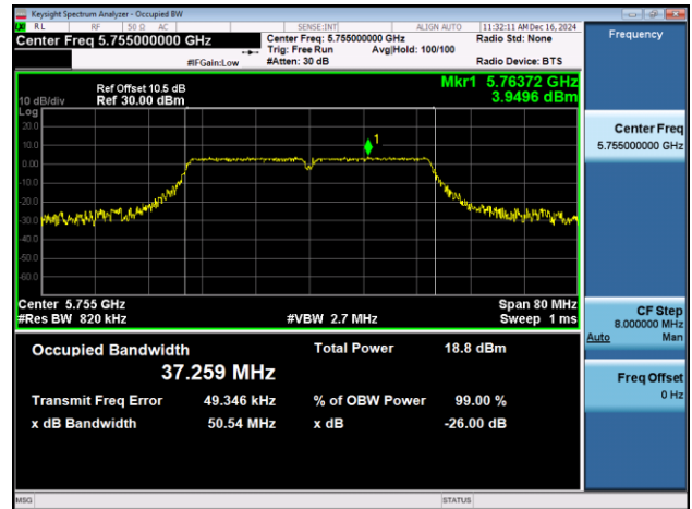
11AC40SISO-Ant1-5755
