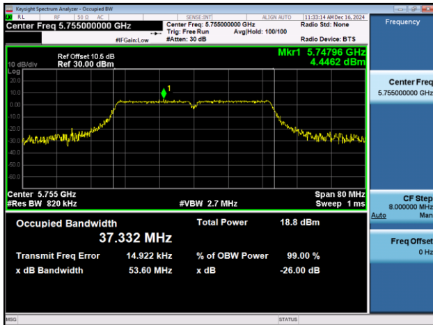
11AX40SISO-Ant1-5755
