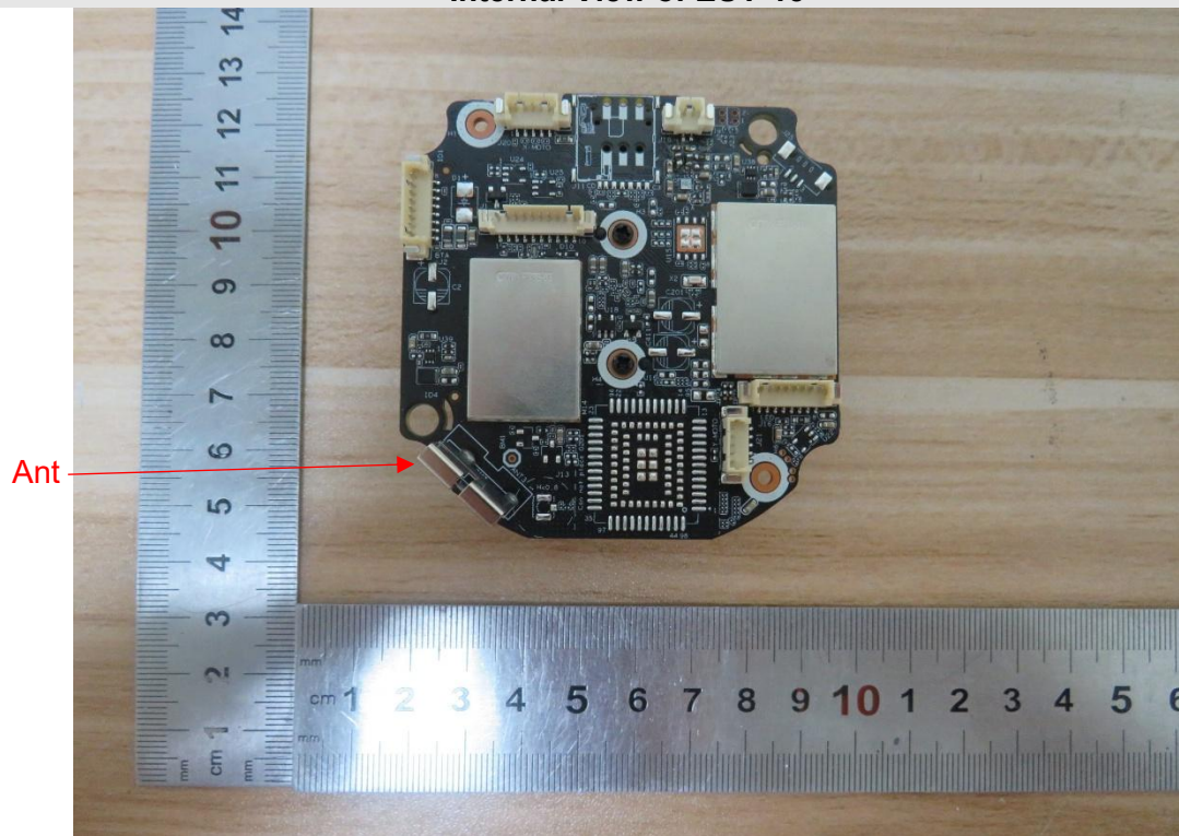
Internal View of EUT-14
