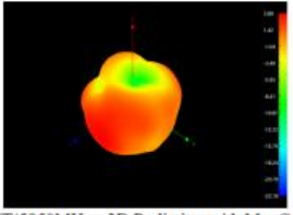
ANT(5850MHz - 3D Radiation with MaxGain)
