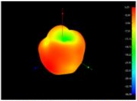
ANT(5750MHz - 3D Radiation with MaxGain)
