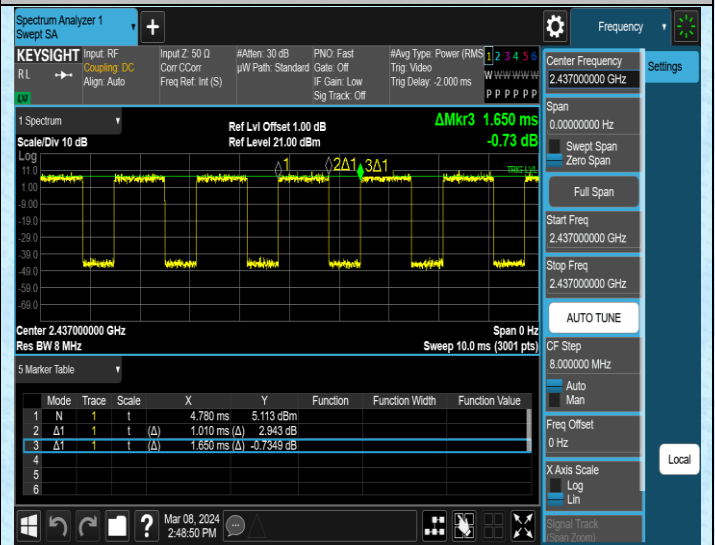
NTNV-11AX20SISO-Ant2-2437
