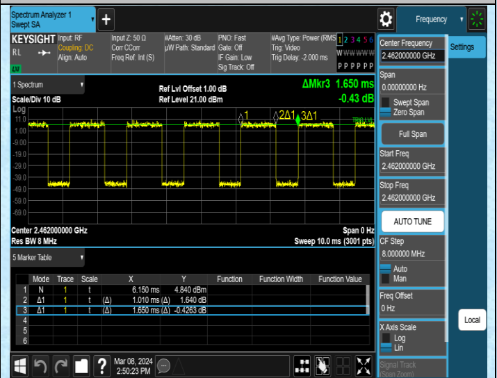
NTNV-11AX20SISO-Ant2-2462
