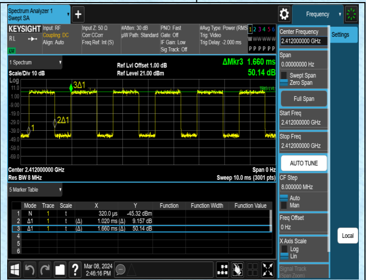
NTNV-11AX20SISO-Ant2-2412
