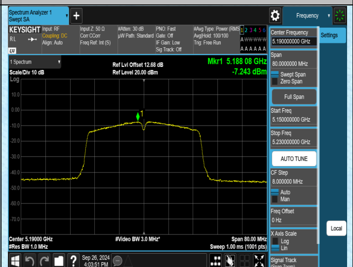
11AC40MIMO-Ant2-5190-PASS
