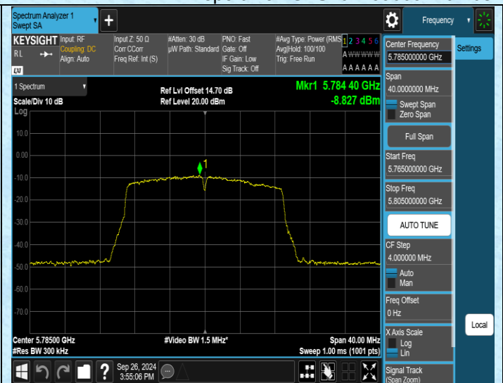
11AC20MIMO-Ant2-5785-PASS
