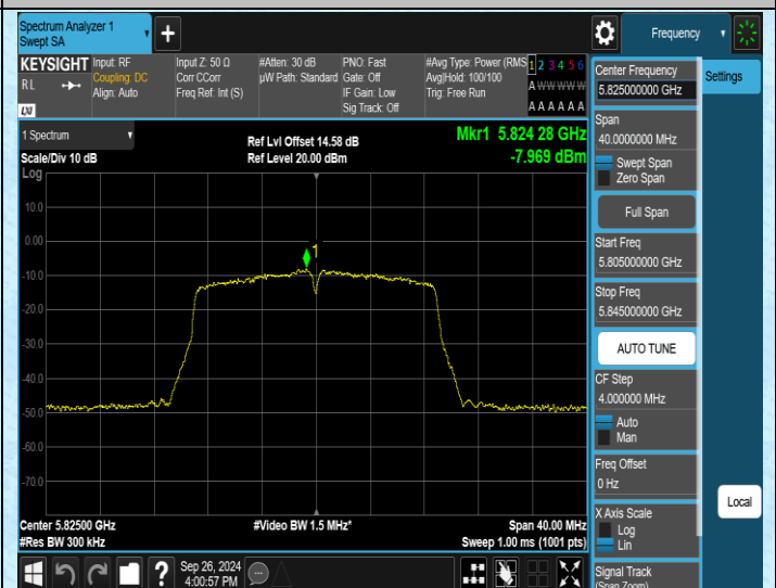
11AC20MIMO-Ant2-5825-PASS
