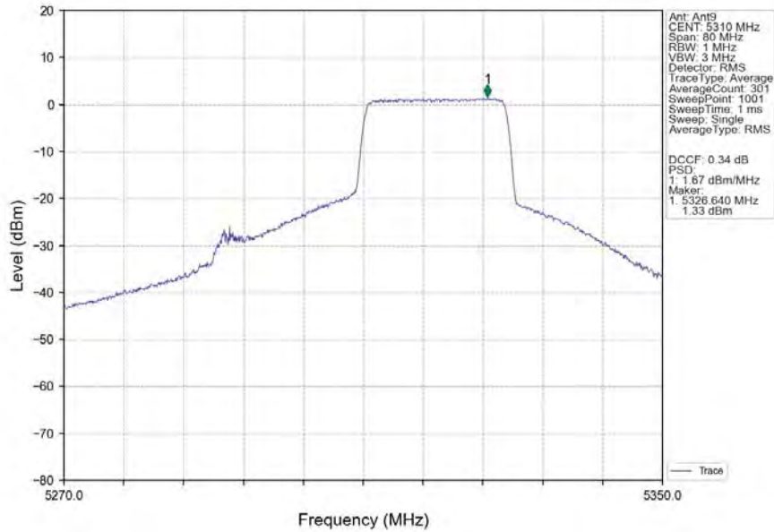
802.11ax(HEW40)_HCH_5310MHz_RU242_Right_Ant9_NTNV
