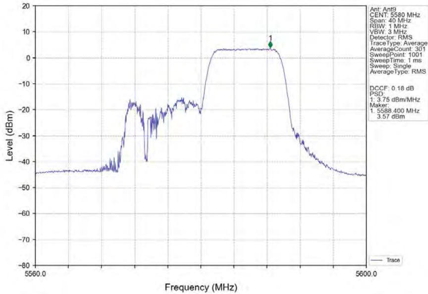
802.11ax(HEW20)_MCH_5580MHz_RU106_Right_Ant9_NTNV
