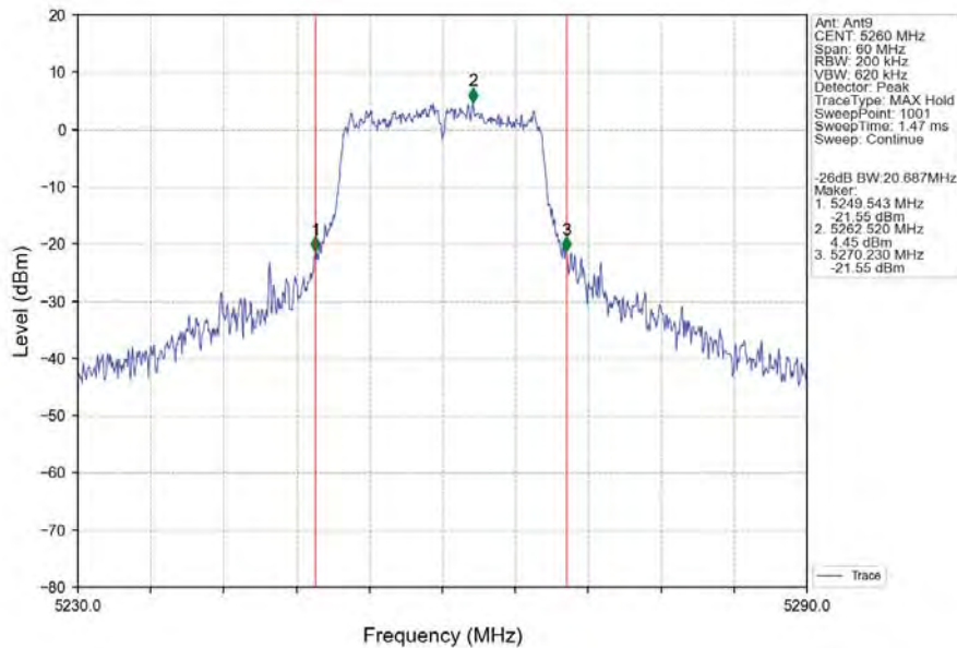
802.11a_LCH_5260MHz_Ant9_NTNV
