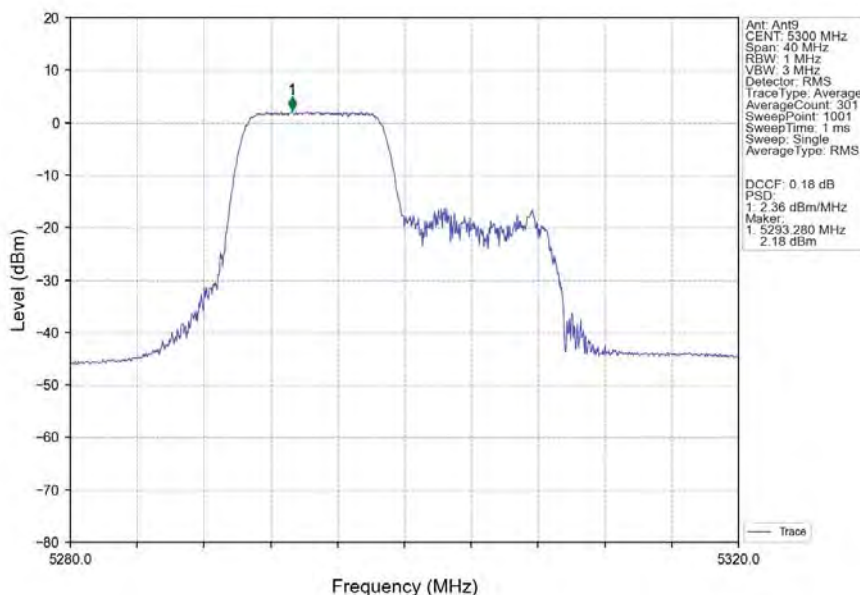
802.11ax(HEW20)_MCH_5300MHz_RU106_Left_Ant9_NTNV
