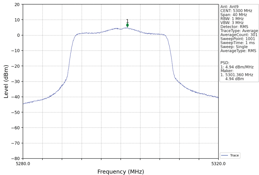
802.11ax(HEW20)_MCH_5300MHz_RU242_Left_Ant9_NTNV
