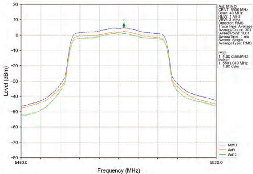
802.11ax(HEW20)_LCH_5500MHz_RU242_Left_MIMO_NTNV
