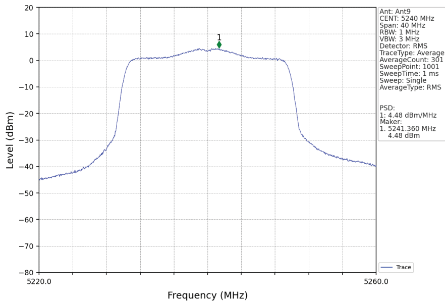
802.11ax(HEW20)_HCH_5240MHz_RU242_Left_Ant9_NTNV
