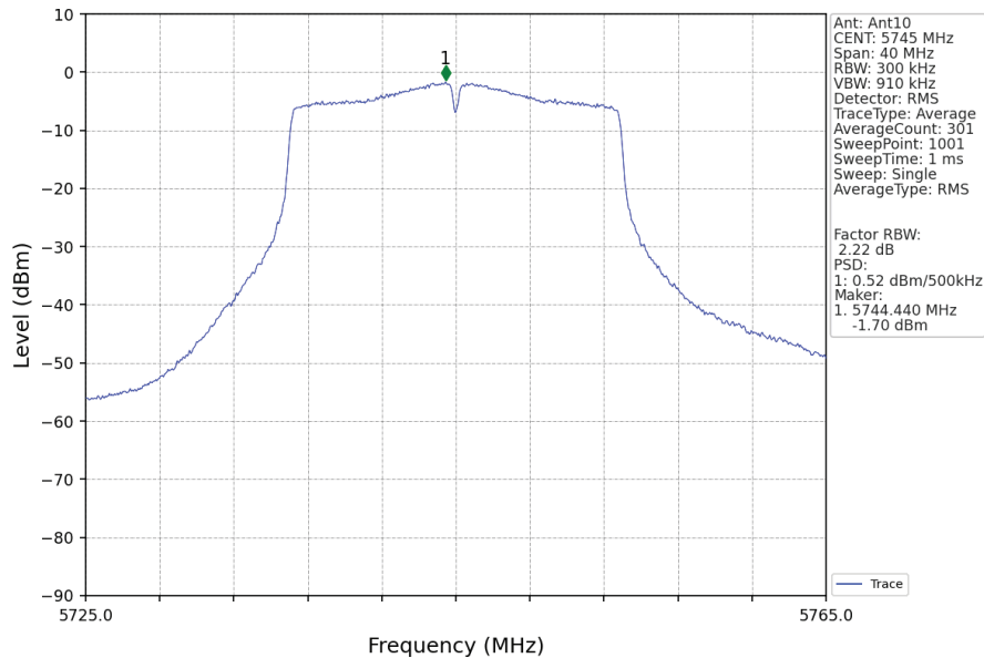
802.11ac(VHT20)_LCH_5745MHz_Ant10_NTNV
