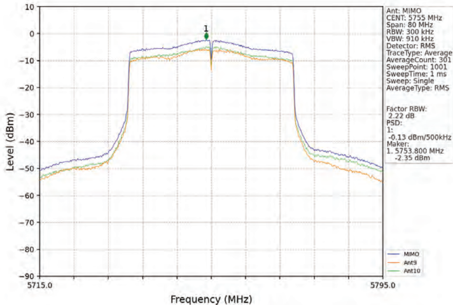
802.11ax(HEW40)_LCH_5755MHz_RU484_Left_MIMO_NTNV
