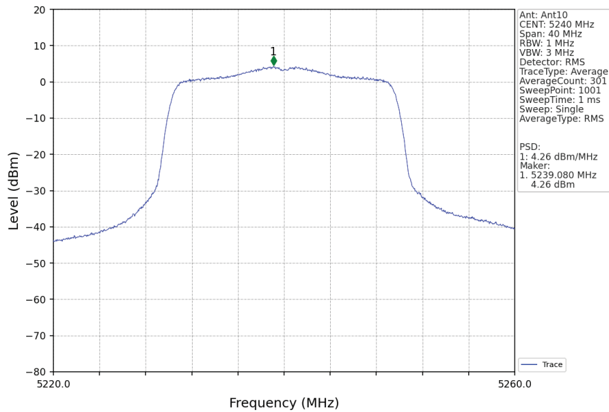
802.11ax(HEW20)_HCH_5240MHz_RU242_Left_MIMO_NTNV
