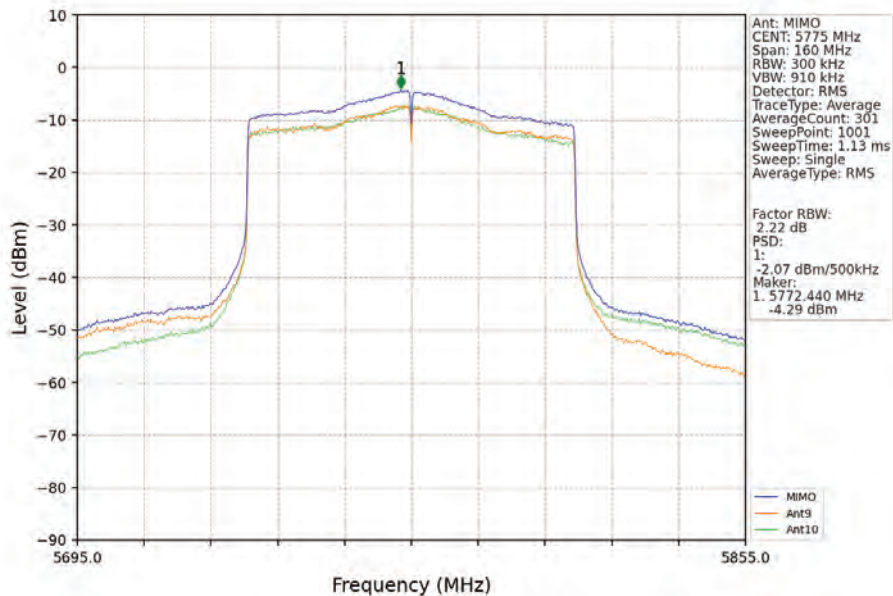
802.11ax(HEW80)_MCH_5775MHz_RU996_Left_MIMO_NTNV
