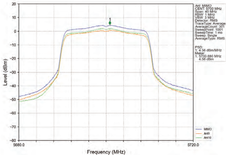
802.11ax(HEW20)_HCH_5700MHz_RU242_Left_MIMO_NTNV
