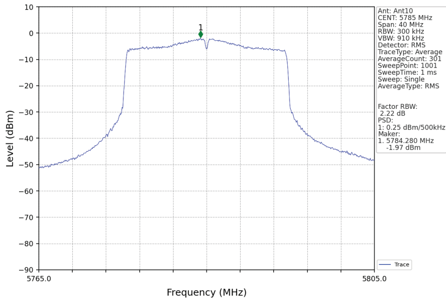
802.11ax(HEW20)_MCH_5785MHz_RU242_Left_MIMO_NTNV
