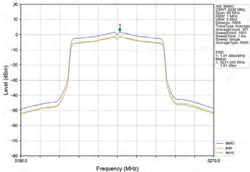
802.11ax(HEW40)_HCH_5230MHz_RU484_Left_MIMO_NTNV
