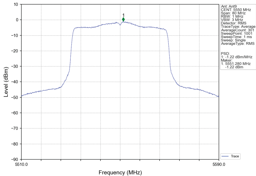
802.11ax(HEW40)_MCH_5550MHz_RU484_Left_Ant9_NTNV
