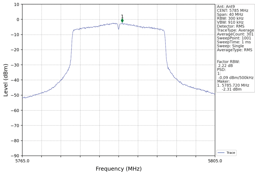
802.11ax(HEW20)_MCH_5785MHz_RU242_Left_Ant9_NTNV
