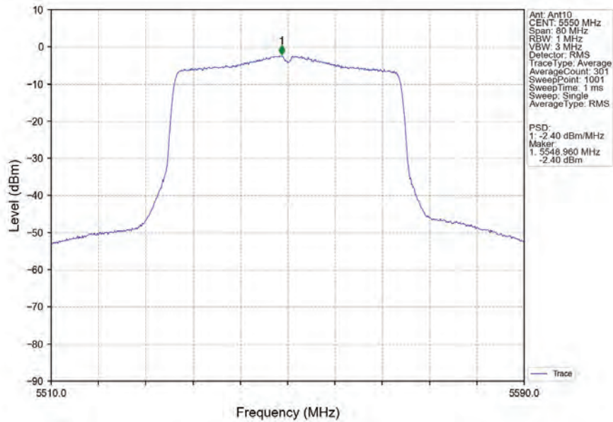
802.11ax(HEW40)_MCH_5550MHz_RU484_Left_MIMO_NTNV
