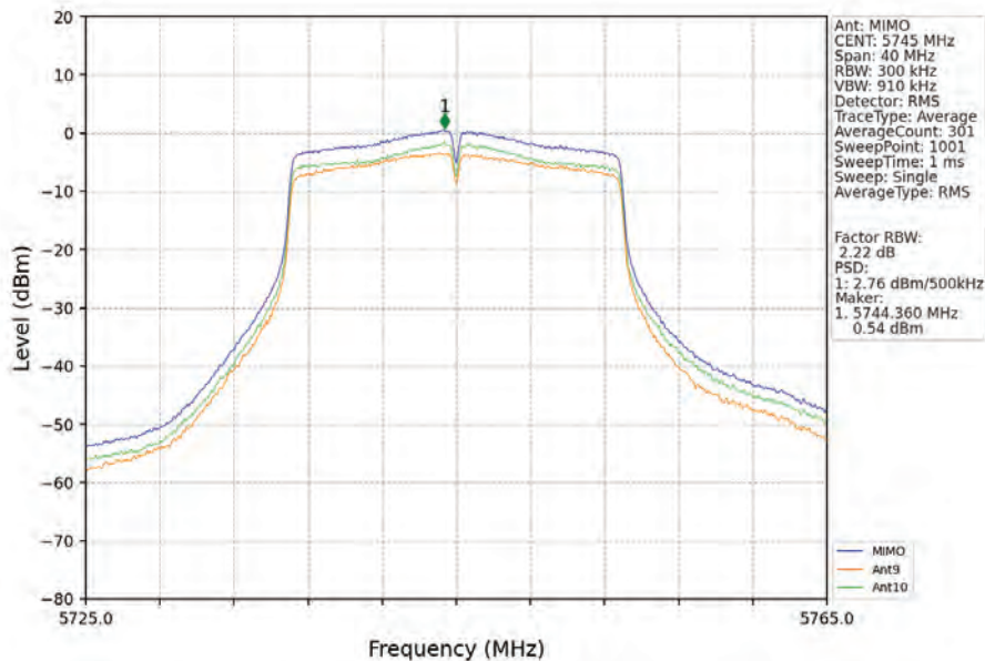
802.11n(HT20)_LCH_5745MHz_MIMO_NTNV
