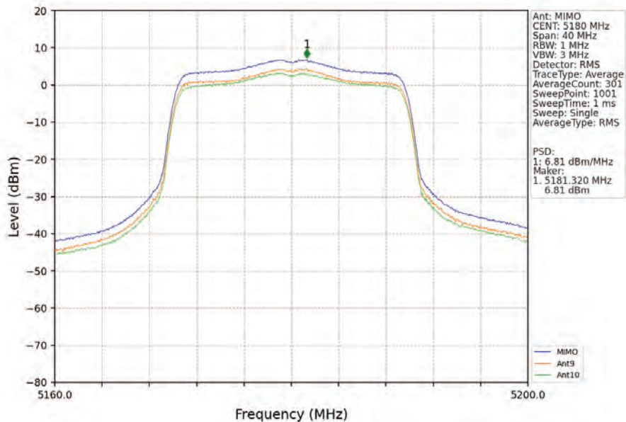
802.11ax(HEW20)_LCH_5180MHz_RU242_Left_MIMO_NTNV
