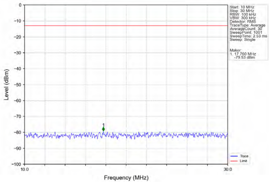
Band26b_1.4MHz_64QAM_LCH_824.7MHz_RB_1_0_NTNV
