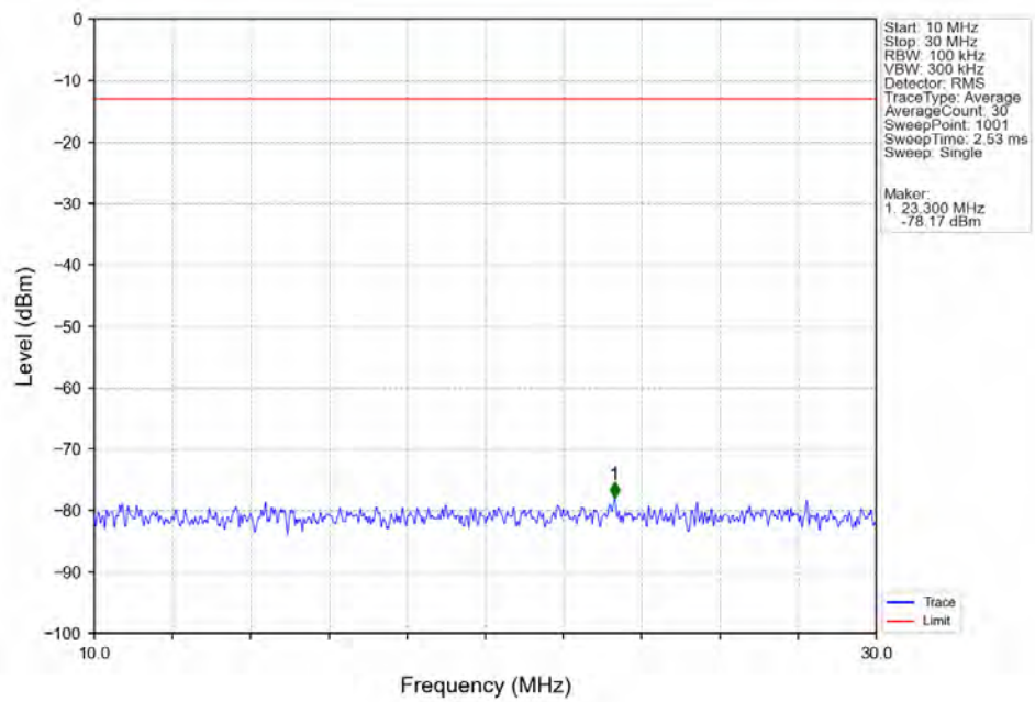
Band26b_1.4MHz_16QAM_LCH_824.7MHz_RB_1_0_NTNV
