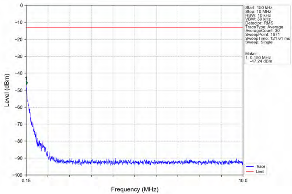
Band26b_1.4MHz_64QAM_HCH_848.3MHz_RB_1_0_NTNV
