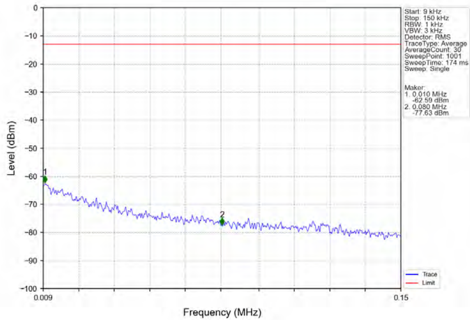
Band26b_1.4MHz_64QAM_HCH_848.3MHz_RB_1_0_NTNV
