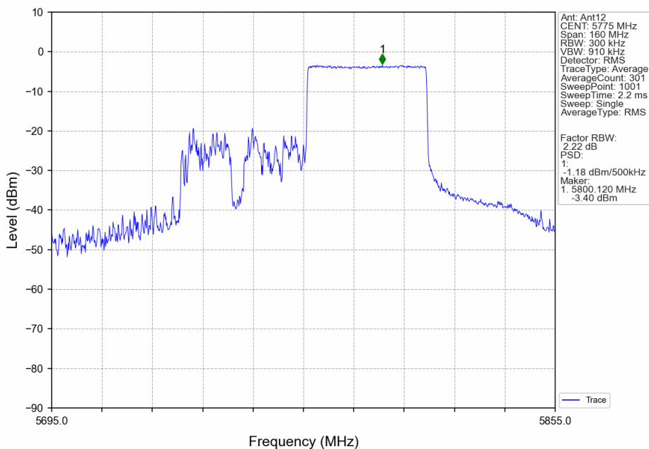
802.11ax(HEW80)_MCH_5775MHz_RU484_Right_Ant12_NTNV
