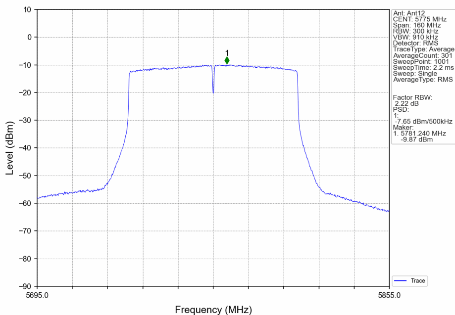
802.11ac(VHT80)_MCH_5775MHz_Ant12_NTNV
