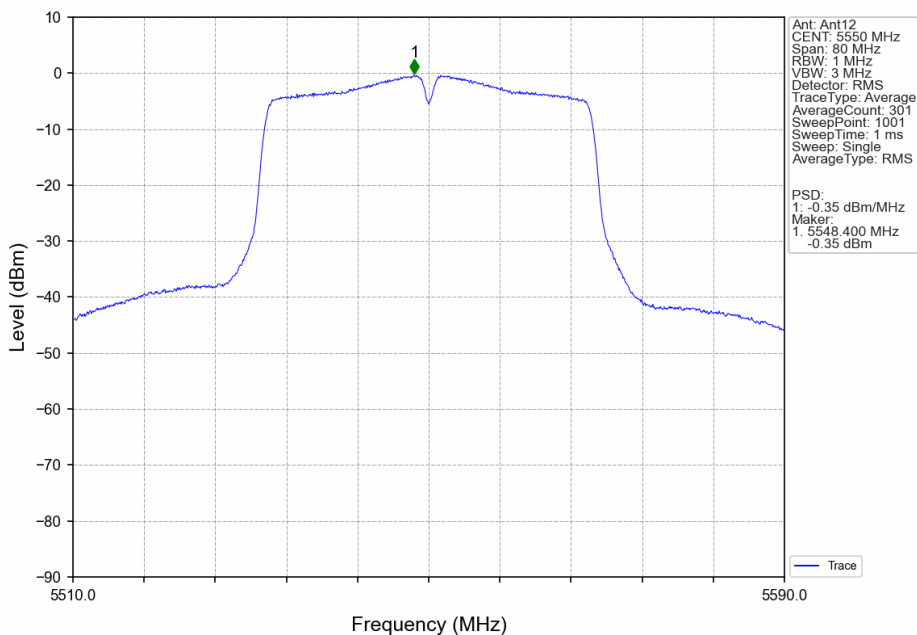
802.11ac(VHT40)_MCH_5550MHz_Ant12_NTNV
