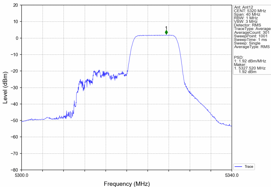
802.11ax(HEW20)_HCH_5320MHz_RU106_Right_Ant12_NTNV
