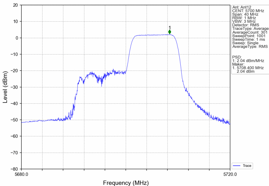
802.11ax(HEW20)_HCH_5700MHz_RU106_Right_Ant12_NTNV
