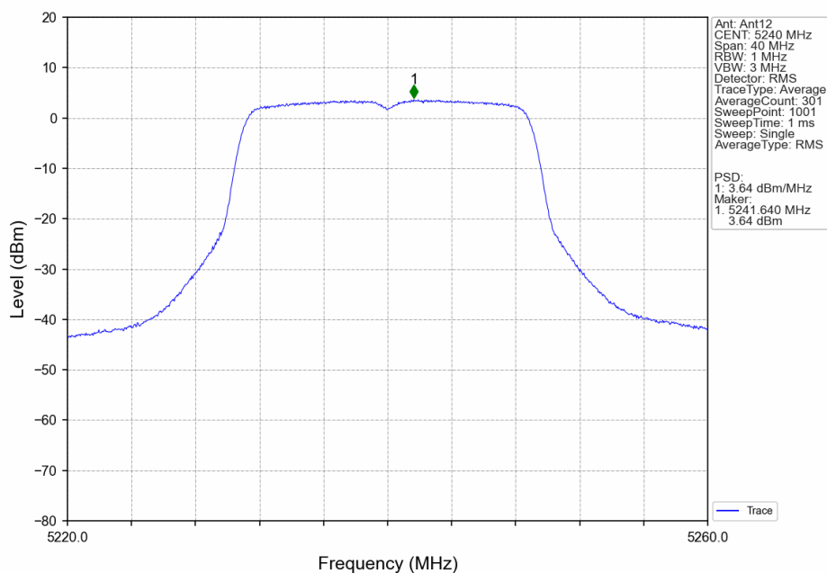
802.11ac(VHT20)_HCH_5240MHz_Ant12_NTNV
