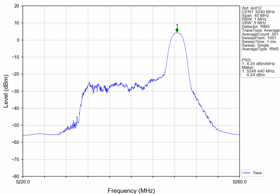
802.11ax(HEW20)_HCH_5240MHz_RU26_Right_Ant12_NTNV
