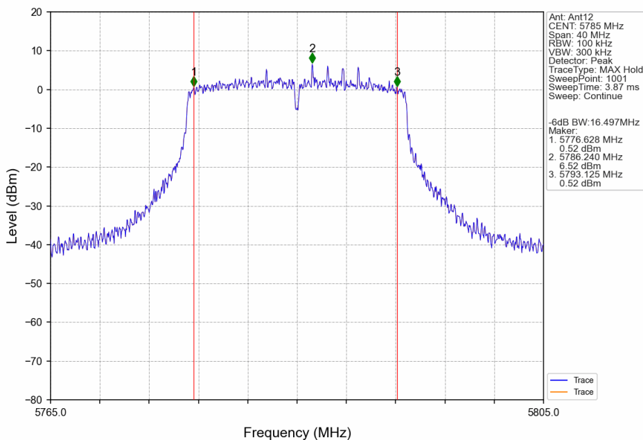
802.11ac(VHT20)_MCH_5785MHz_Ant12_NTNV
