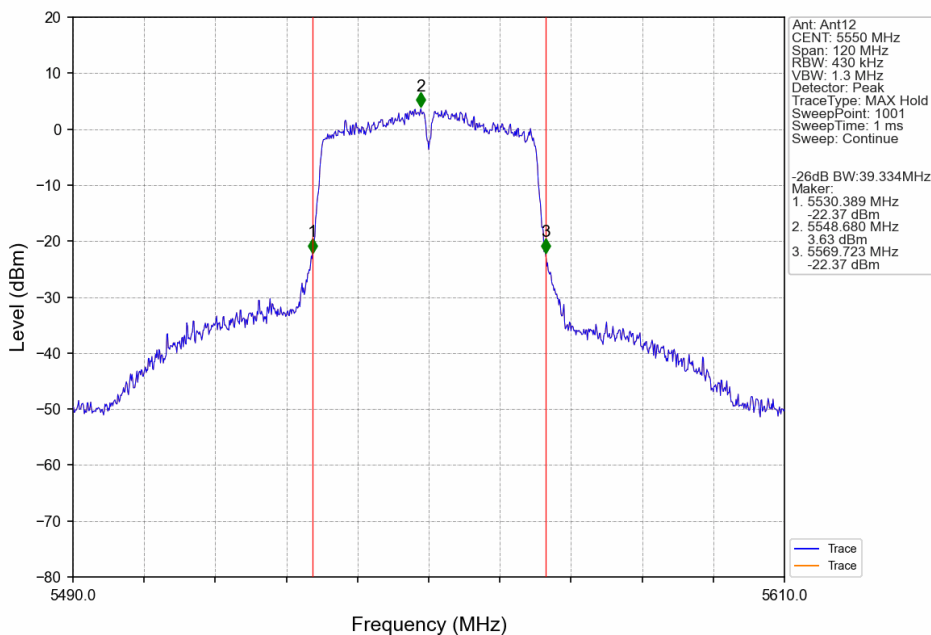
802.11ac(VHT40)_MCH_5550MHz_Ant12_NTNV
