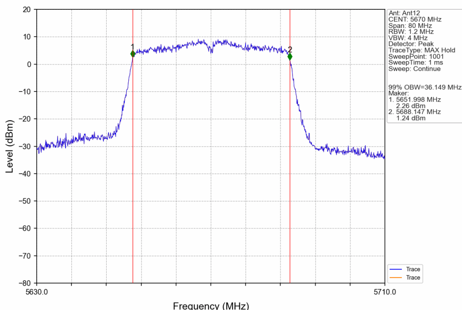
802.11ac(VHT40)_HCH_5670MHz_Ant12_NTNV
