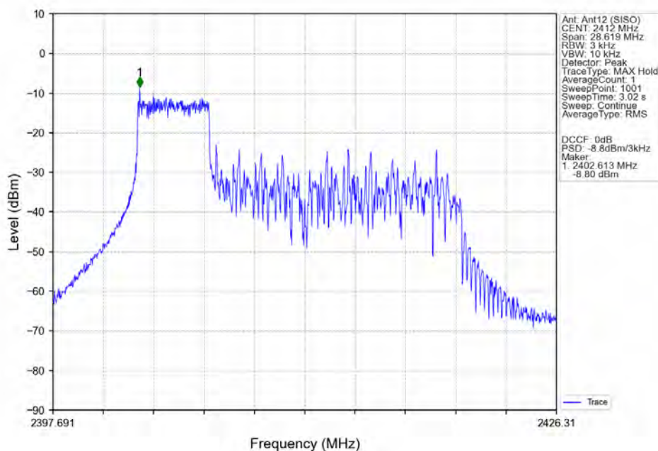
802.11ax(HEW20)_LCH_2412MHz_RU52_Left_Ant12 (SISO)_NTNV
