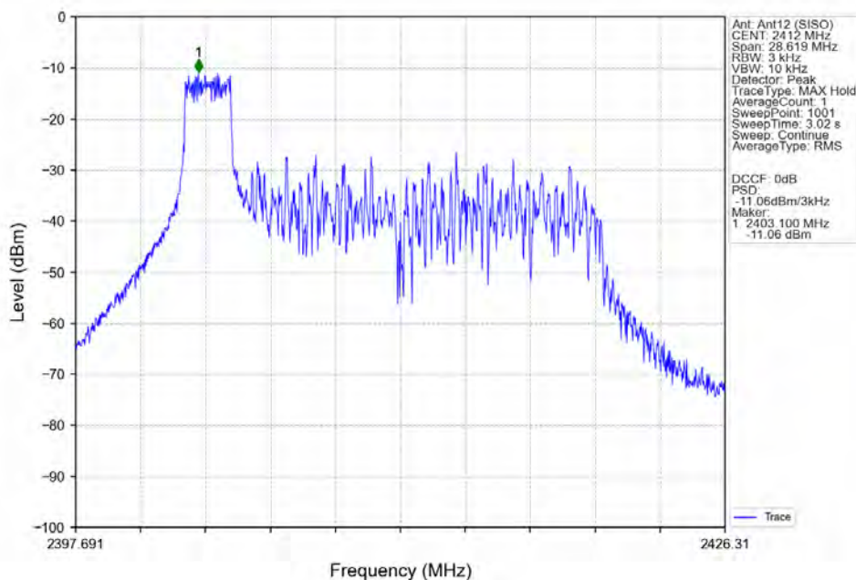
802.11ax(HEW20)_LCH_2412MHz_RU52_Left_Ant12 (SISO)_NTNV
