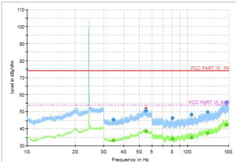
Fig.34 Radiated Spurious Emission (802.11b, CH6, 1GHz-18GHz)
