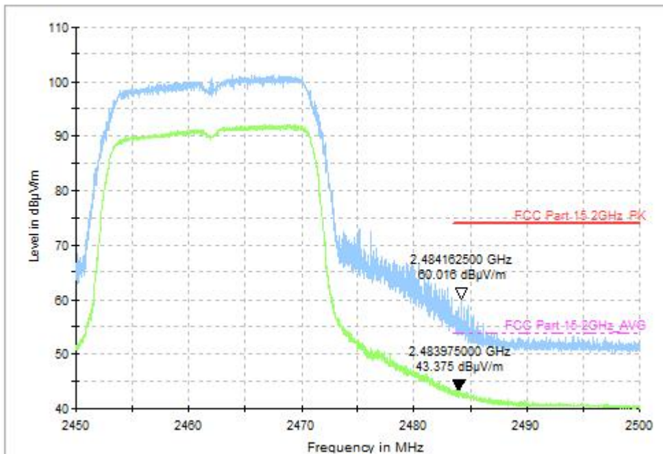
Fig.52 Radiated Restricted Band (802.11-VHT20, CH11, 2.45GHz~2.50GHz)
