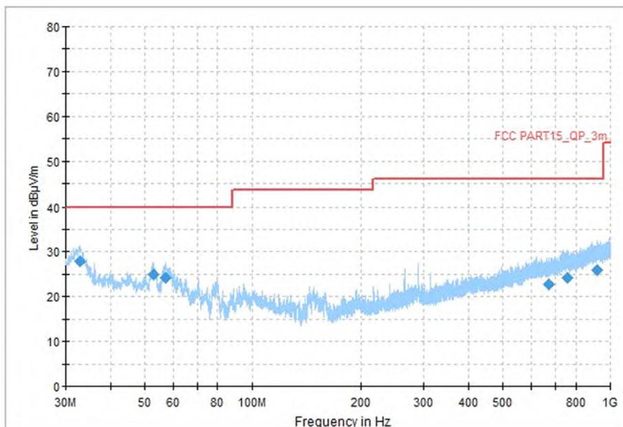
Fig.64 Radiated Spurious Emission (All Channels, 30MHz-1GHz)
