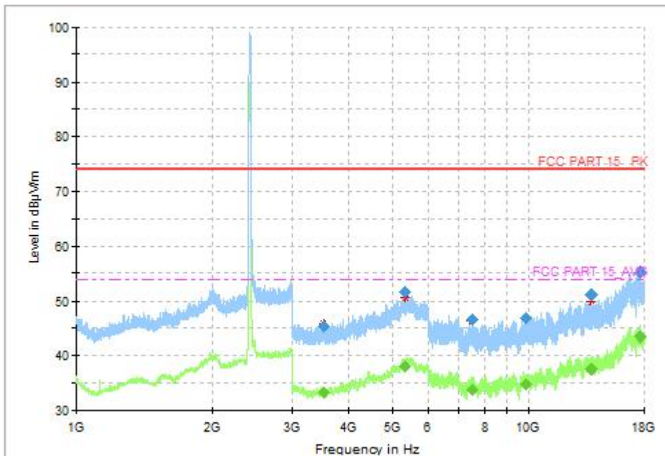
Fig.58 Radiated Spurious Emission (802.11-VHT40, CH3, 1GHz-18GHz)
