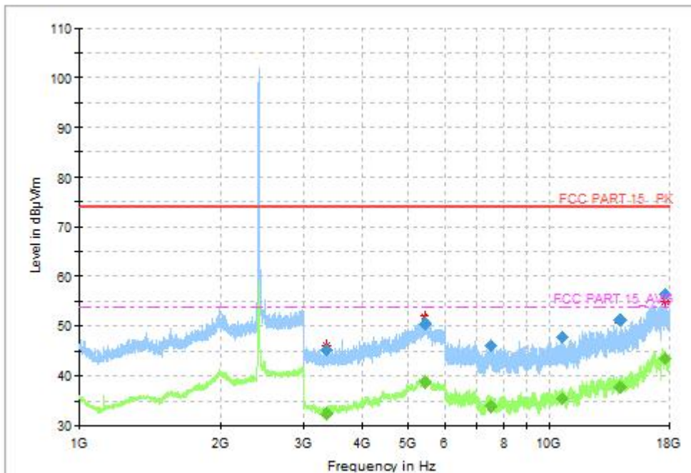
Fig.38 Radiated Spurious Emission (802.11g, CH1, 1GHz-18GHz)
