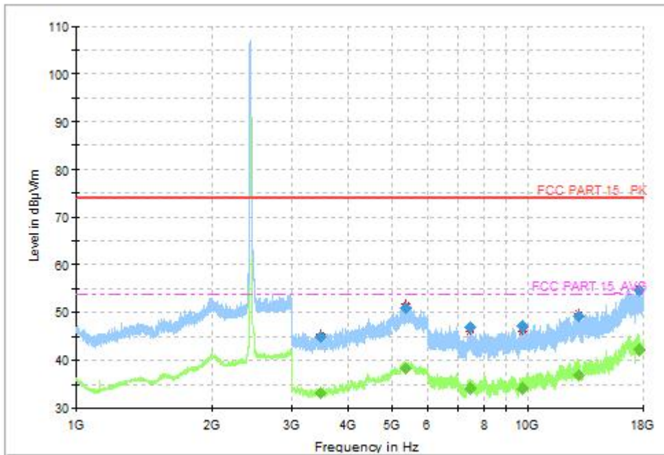
Fig.49 Radiated Spurious Emission (802.11-VHT20, CH6, 1GHz-18GHz)
