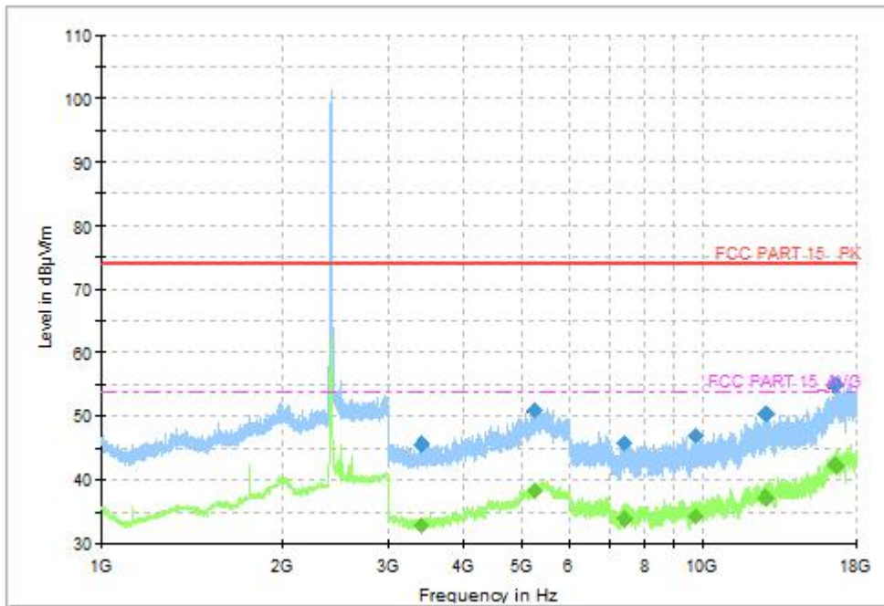
Fig.43 Radiated Spurious Emission (802.11n-HT20, CH1, 1GHz-18GHz)
