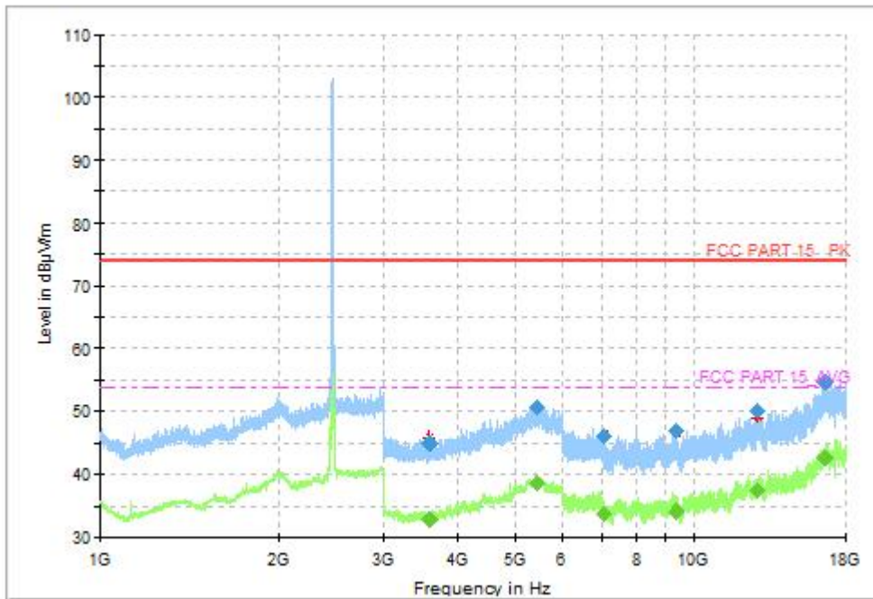
Fig.35 Radiated Spurious Emission (802.11b, CH11, 1GHz-18GHz)
