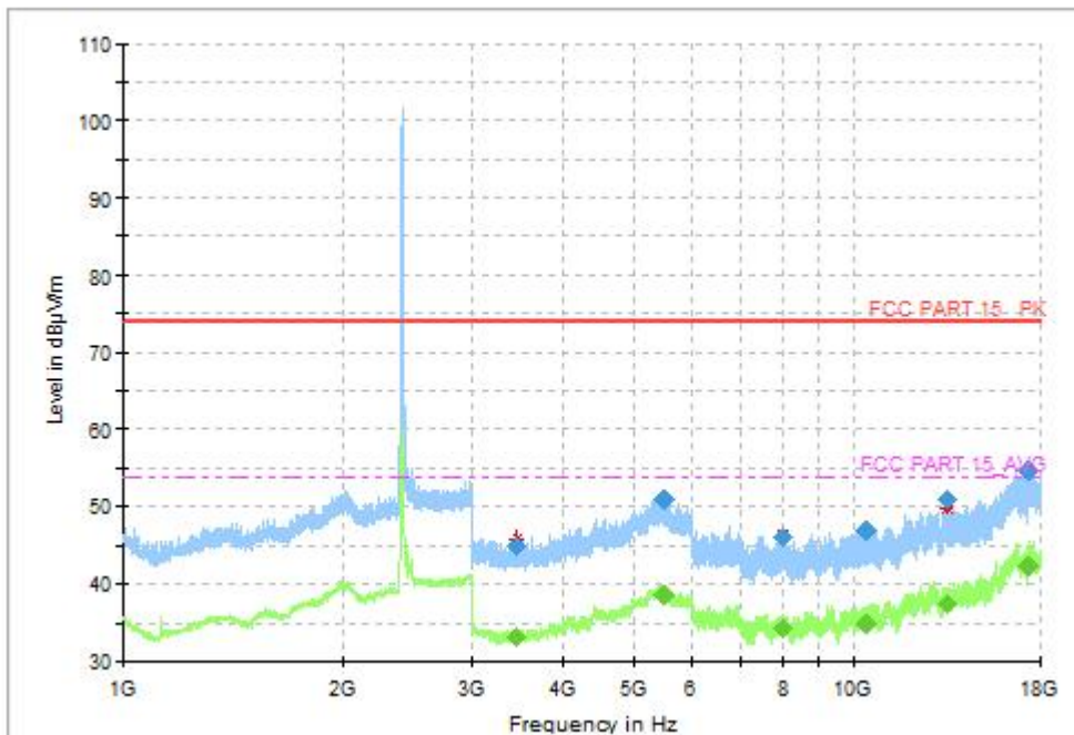
Fig.48 Radiated Spurious Emission (802.11-VHT20, CH1, 1GHz-18GHz)
