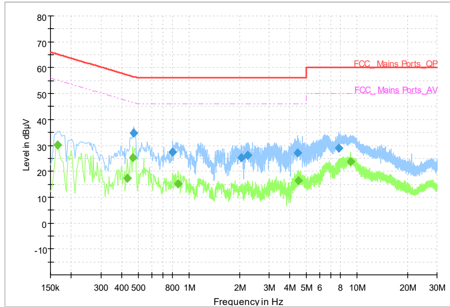
Fig.66 AC Power line Conducted Emission (Traffic)
