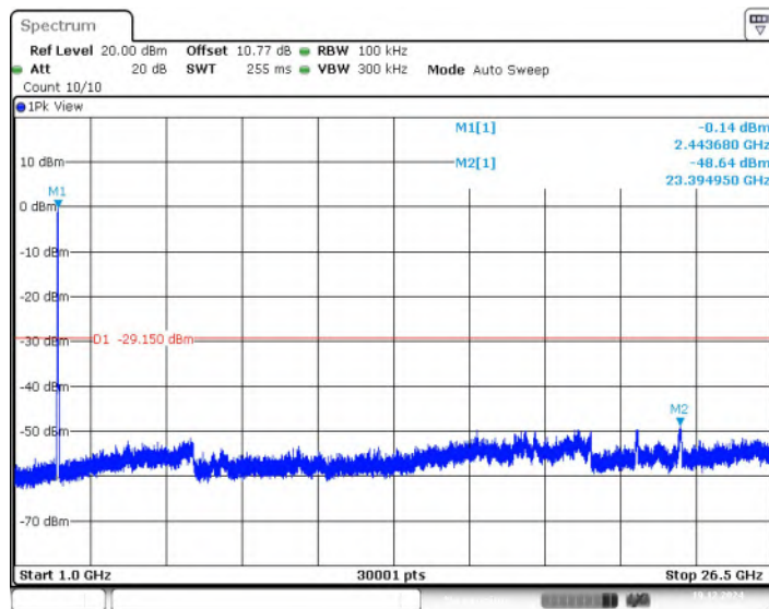
Fig.27 Conducted Spurious Emission (1GHz-26.5GHz, 802.11n-HT40, CH6)
