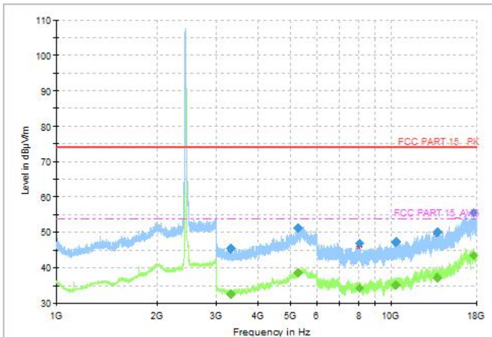
Fig.44 Radiated Spurious Emission (802.11n-HT20, CH6, 1GHz-18GHz)
