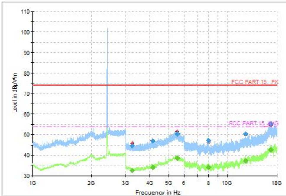
Fig.33 Radiated Spurious Emission (802.11b, CH1, 1GHz-18GHz)
