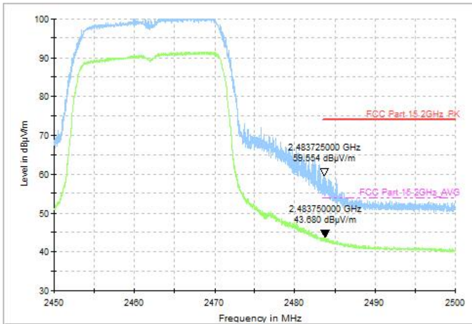
Fig.47 Radiated Restricted Band (802.11n-HT20, CH11, 2.45GHz~2.50GHz)
