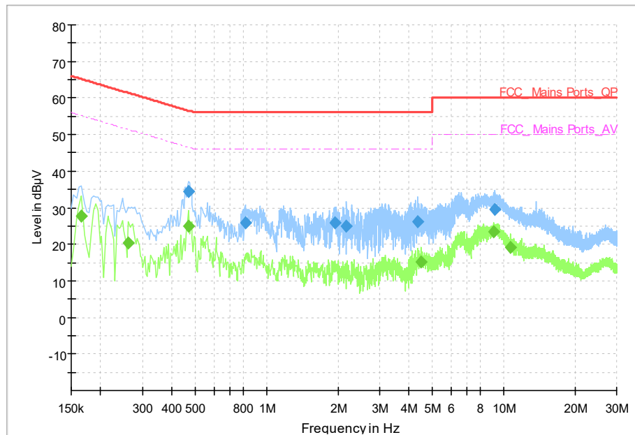
Fig.67 AC Power line Conducted Emission (Idle)
