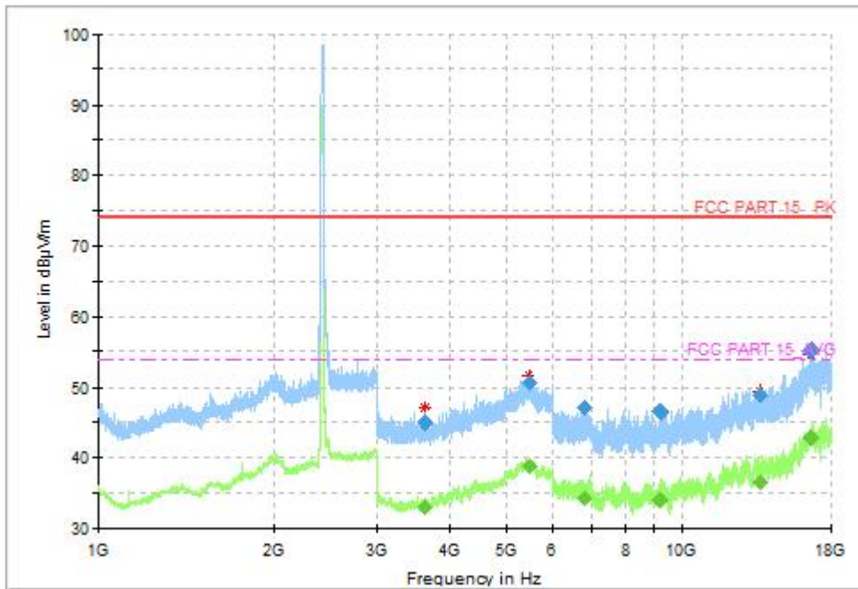
Fig.53 Radiated Spurious Emission (802.11n-HT40, CH3, 1GHz-18GHz,)
