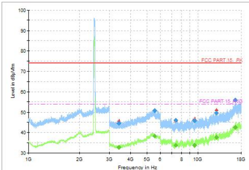
Fig.60 Radiated Spurious Emission (802.11-VHT40, CH9, 1GHz-18GHz)
