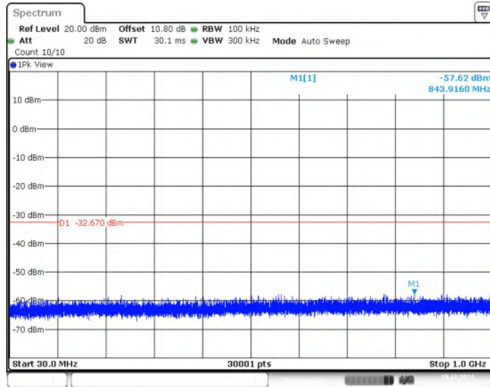
Fig.32 Conducted Spurious Emission (All Channels, 30MHz -1GHz)
