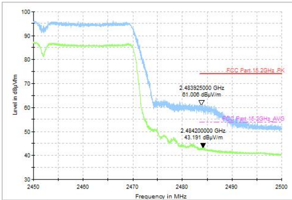
Fig.57 Radiated Restricted Band (802.11n-HT40, CH9, 2.45GHz~2.50GHz)
