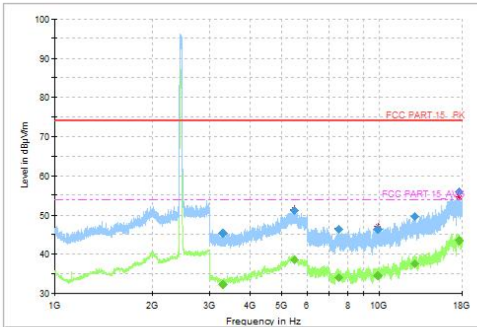
Fig.55 Radiated Spurious Emission (802.11n-HT40, CH9, 1GHz-18GHz)
