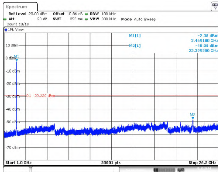
Fig.25 Conducted Spurious Emission (1GHz-26.5GHz, 802.11-VHT20, CH11)
