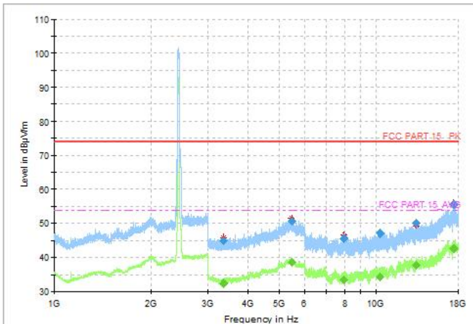
Fig.54 Radiated Spurious Emission (802.11n-HT40, CH6, 1GHz-18GHz)
