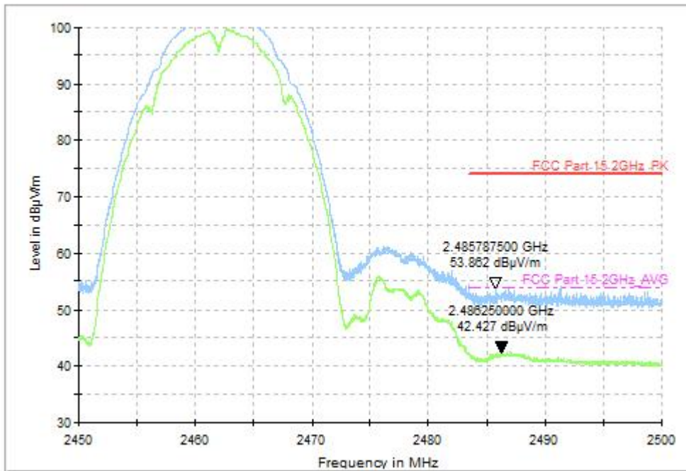
Fig.37 Radiated Restricted Band (802.11b, CH11, 2.45GHz~2.50GHz)
