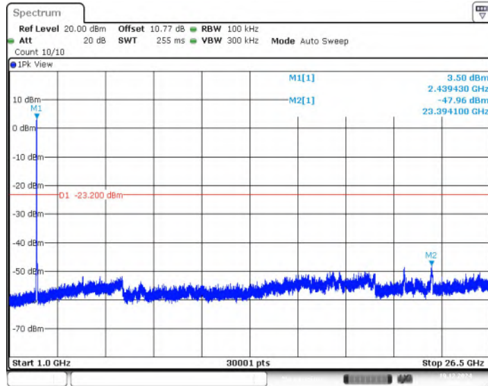
Fig.24 Conducted Spurious Emission (1GHz-26.5GHz, 802.11-VHT20, CH6)
