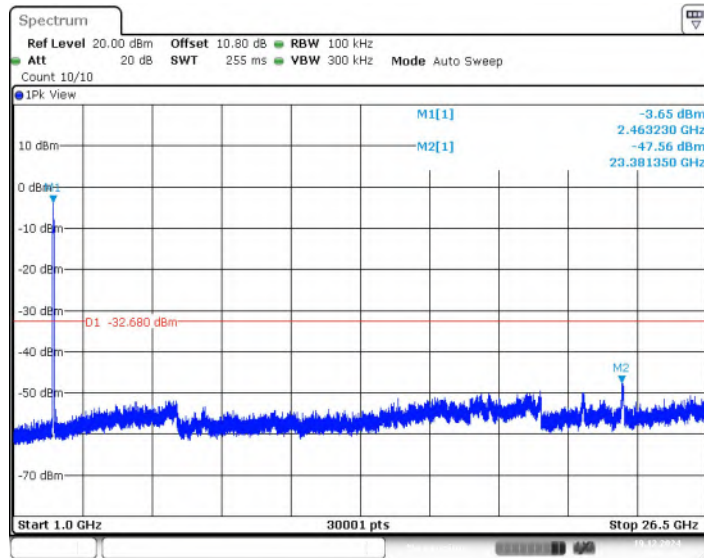
Fig.28 Conducted Spurious Emission (1GHz-26.5GHz, 802.11n-HT40, CH9)
