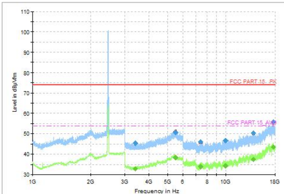
Fig.50 Radiated Spurious Emission (802.11-VHT20, CH11, 1GHz-18GHz)
