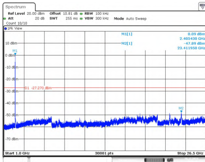
Fig.23 Conducted Spurious Emission (1GHz-26.5GHz, 802.11-VHT20, CH1)
