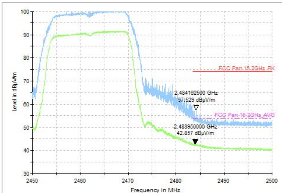
Fig.42 Radiated Restricted Band (802.11g, CH11, 2.45GHz~2.50GHz)
