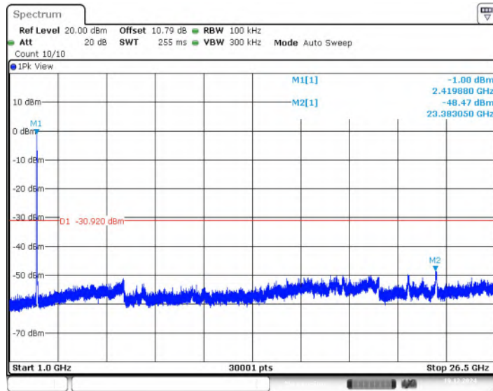
Fig.26 Conducted Spurious Emission (1GHz-26.5GHz, 802.11n-HT40, CH3)
