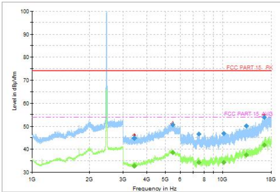
Fig.45 Radiated Spurious Emission (802.11n-HT20, CH11, 1GHz-18GHz)
