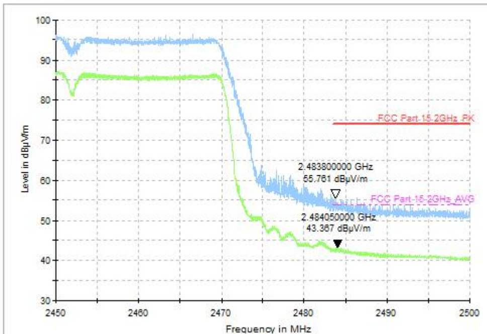
Fig.62 Radiated Restricted Band (802.11-VHT40, CH9, 2.45GHz~2.50GHz)
