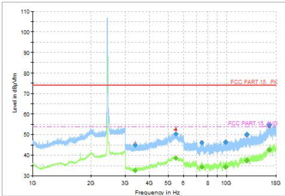
Fig.39 Radiated Spurious Emission (802.11g, CH6, 1GHz-18GHz)
