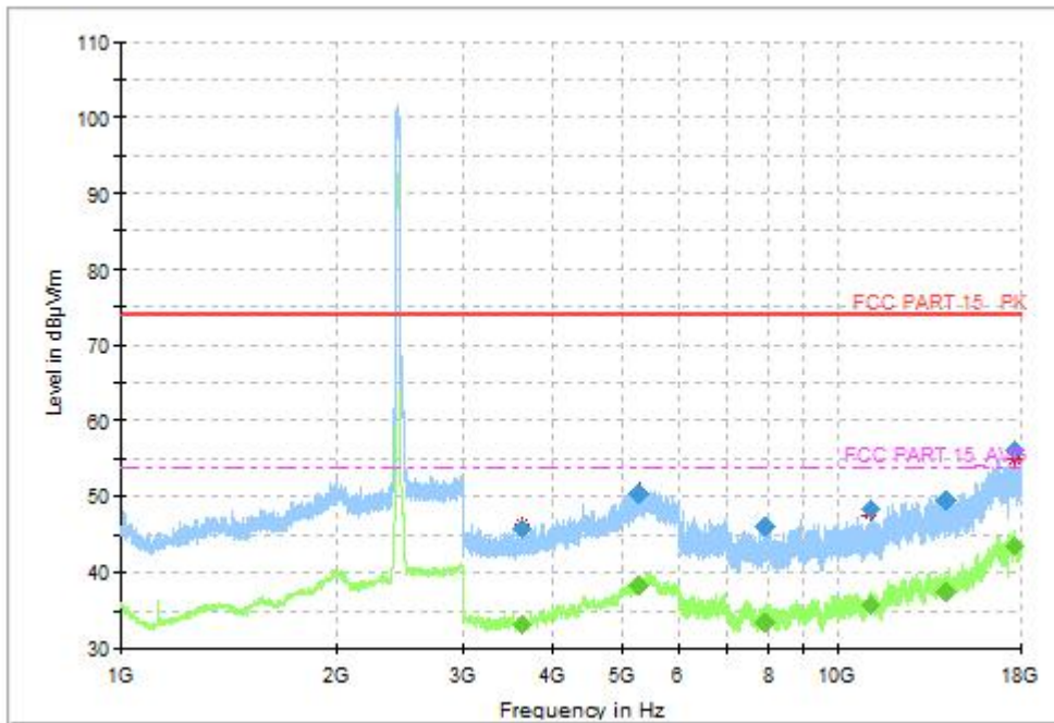
Fig.59 Radiated Spurious Emission (802.11-VHT40, CH6, 1GHz-18GHz)
