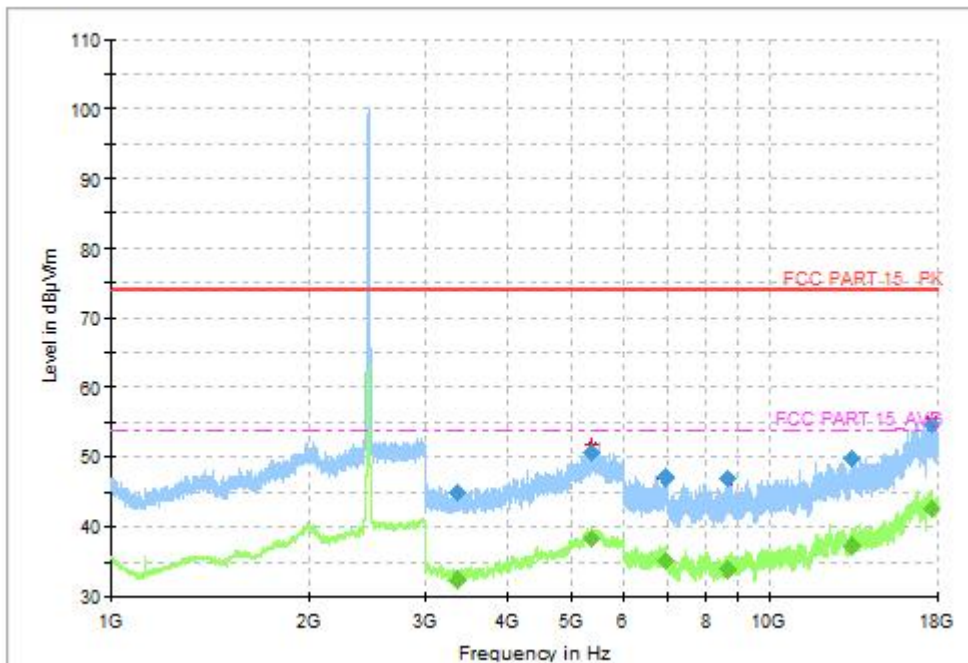
Fig.40 Radiated Spurious Emission (802.11g, CH11, 1GHz-18GHz)
