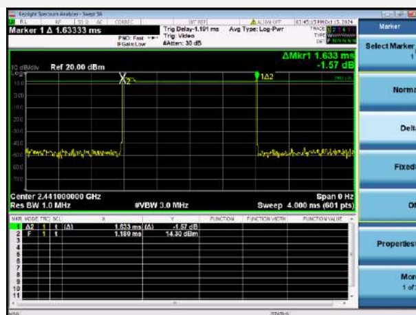
8-DPSK 3DH3
