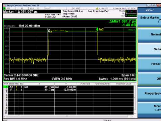
8-DPSK 3DH1
