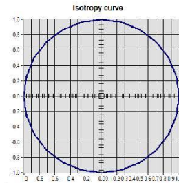
Isotropy: +/-0.12% (+/-0.01dB)
