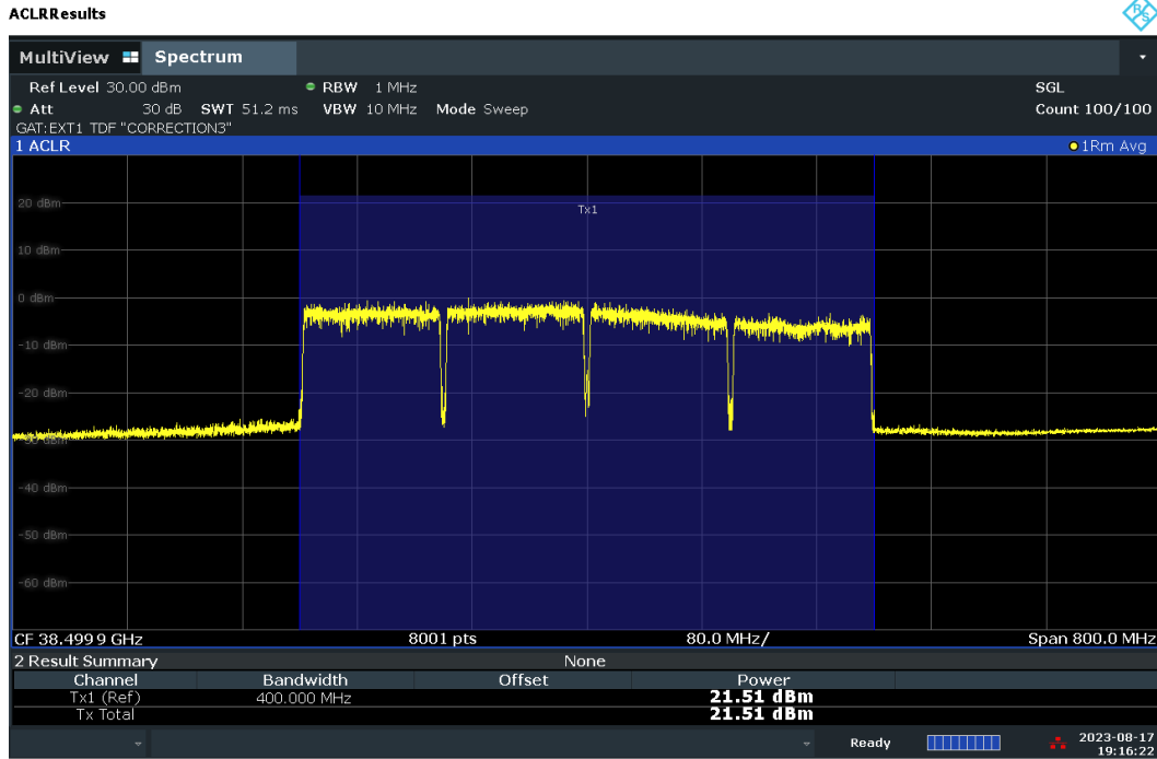
Plot 7-122. Conducted Power Plot – CP – H-DL Polarization (100MHz-4CC – QPSK – Mid Ch. – Full RB)
