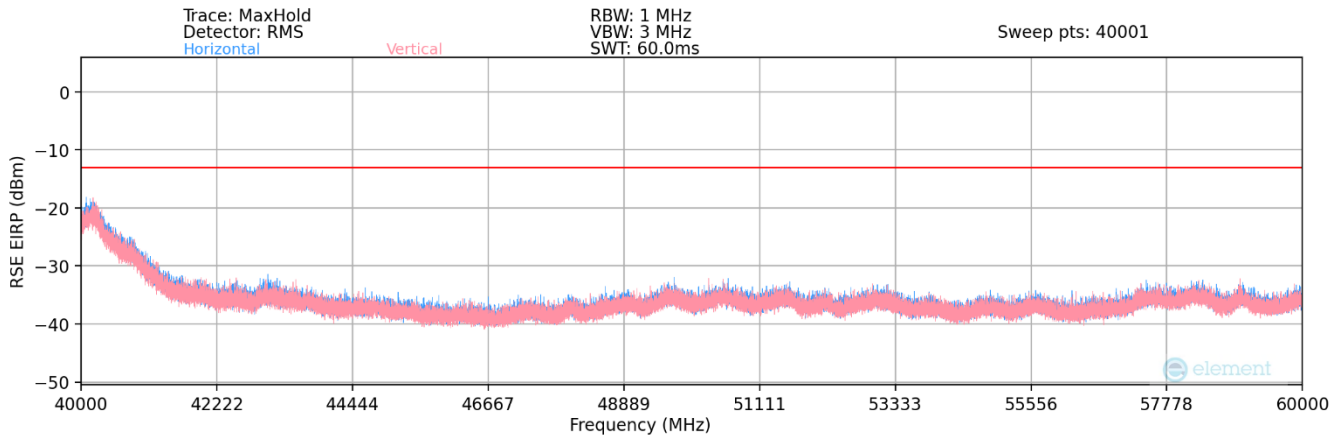
Plot 7-131. n260 Radiated Spurious Plot (1CC QPSK High Channel) - SU
