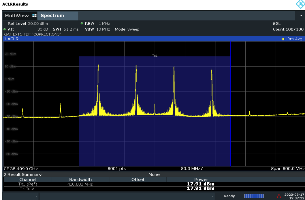
Plot 7-123. Conducted Power Plot – CP – H-DL Polarization (100MHz-4CC – QPSK – Mid Ch. – 1 RB)
