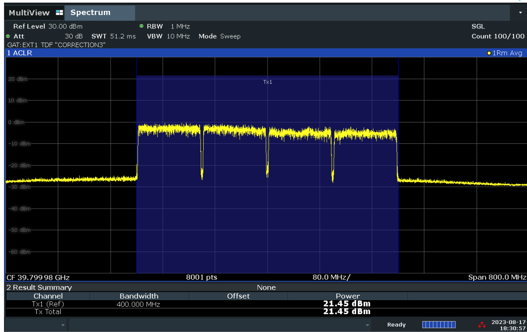
Plot 7-126. Conducted Power Plot – CP – H-DL Polarization (100MHz-4CC – 16QAM – High Ch. – Full RB)
