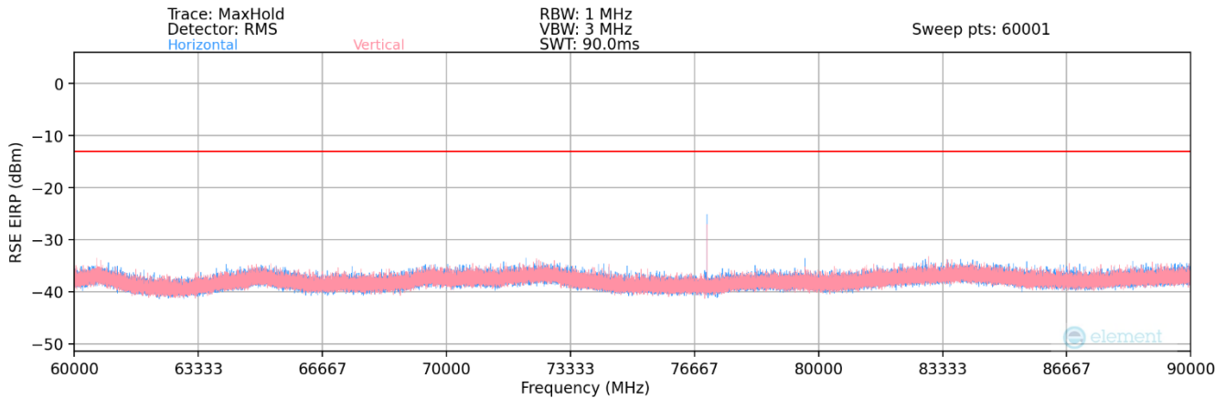
Plot 7-132. n260 Radiated Spurious Plot (1CC QPSK Mid Channel) - SU
