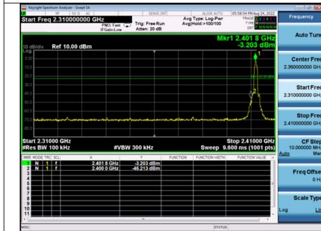
8DPSK No-Hopping Band edge-Left side
