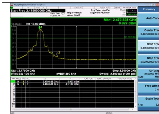
8DPSK No-Hopping Band edge-Right side
