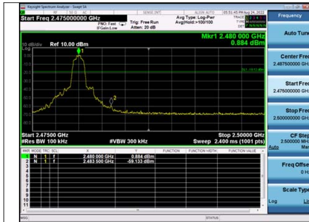
\pi/4 -DQPSK No-Hopping Band edge-Right side
