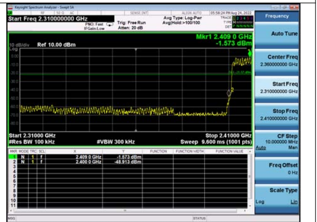
8DPSK Hopping Band edge-Left side
