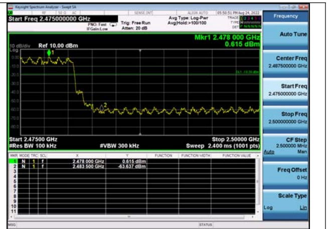
\pi/4 -DQPSK Hopping Band edge-Right side
