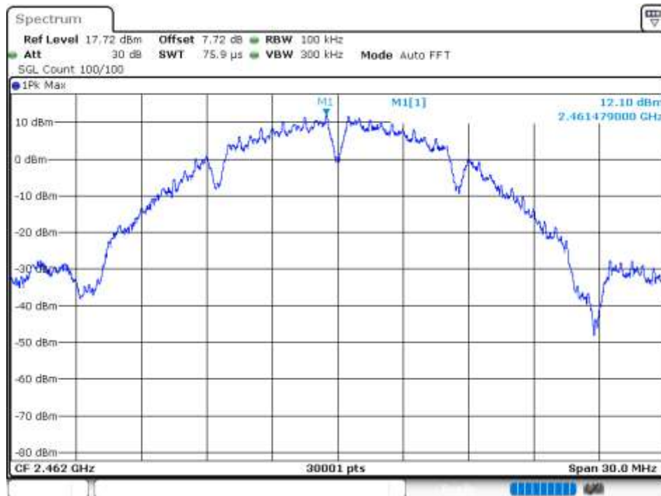
Tx. Spurious NVNT 802.11b 2462MHz Ant 0 Emission
