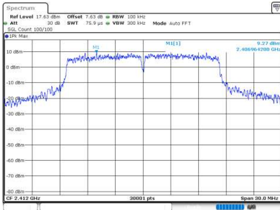
Tx. Spurious NVNT 802.11g 2412MHz Ant 0 Emission
