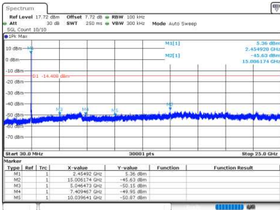
Tx. Spurious NVNT 802.11ax20 2462MHz Ant 3 Emission
