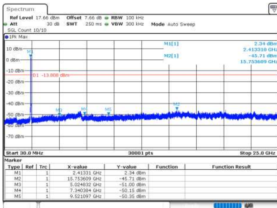
Tx. Spurious NVNT 802.11ax40 2422MHz Ant 0 Emission
