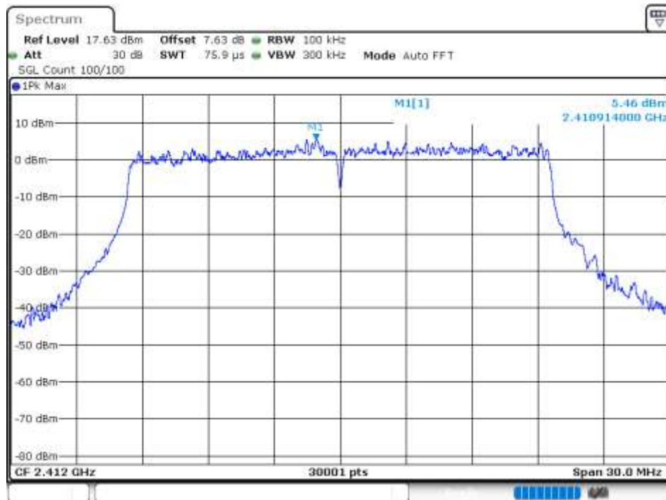
Tx. Spurious NVNT 802.11ax20 2412MHz Ant 0 Emission
