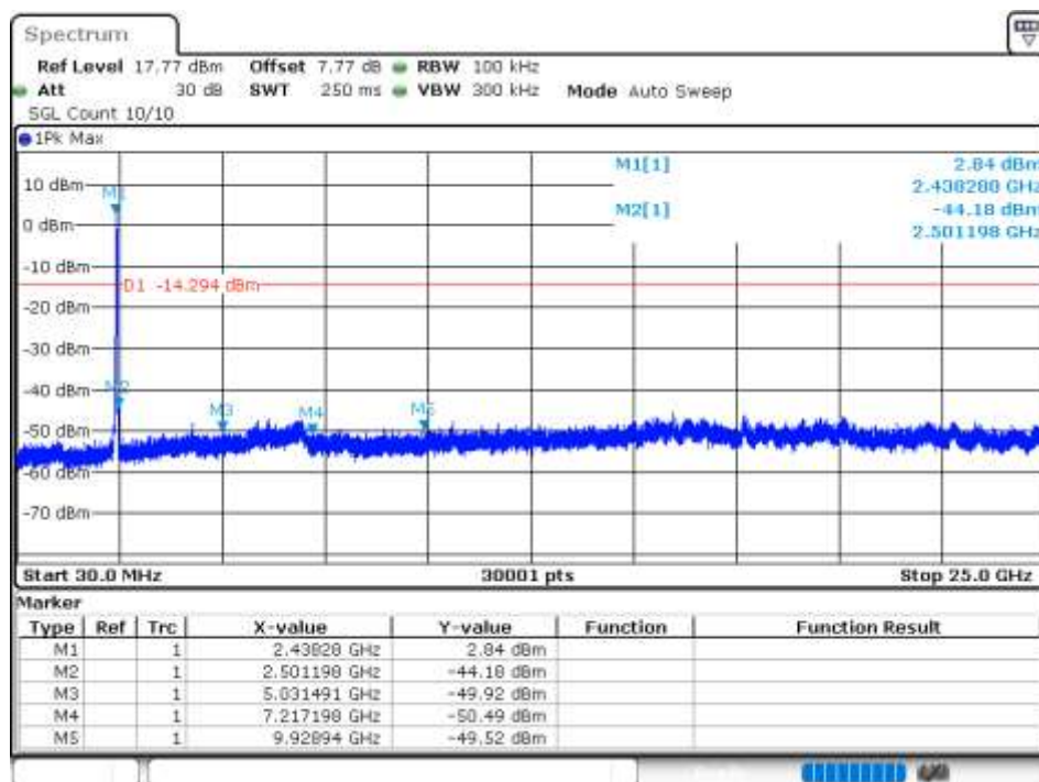
Tx. Spurious NVNT 802.11ax40 2437MHz Ant 3 Emission
