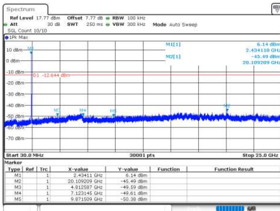
Tx. Spurious NVNT 802.11ax20 2437MHz Ant 2 Emission
