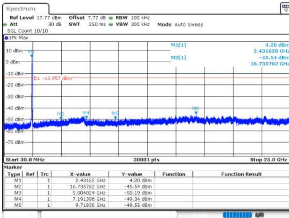
Tx. Spurious NVNT 802.11ax40 2437MHz Ant 0 Emission
