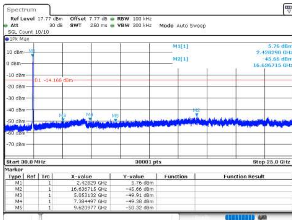
Tx. Spurious NVNT 802.11ax40 2437MHz Ant 1 Emission
