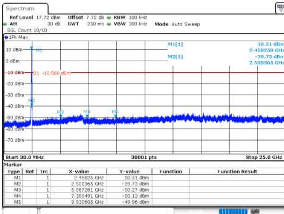
Tx. Spurious NVNT 802.11g 2462MHz Ant 0 Emission
