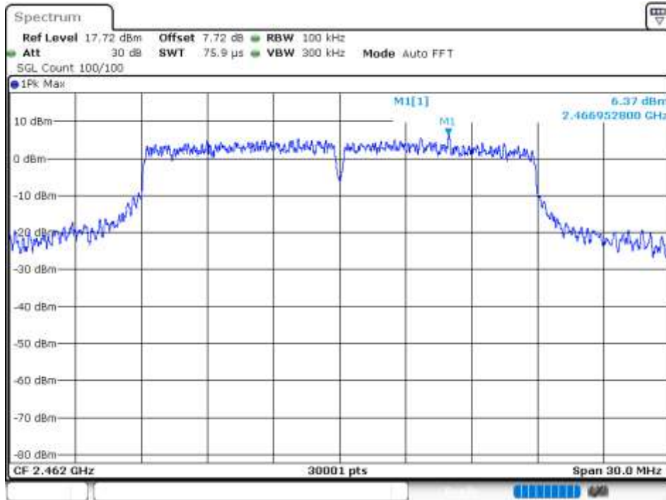
Tx. Spurious NVNT 802.11n(HT20) 2462MHz Ant 0 Emission
