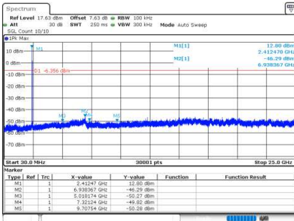
Tx. Spurious NVNT 802.11b 2412MHz Ant 3 Emission
