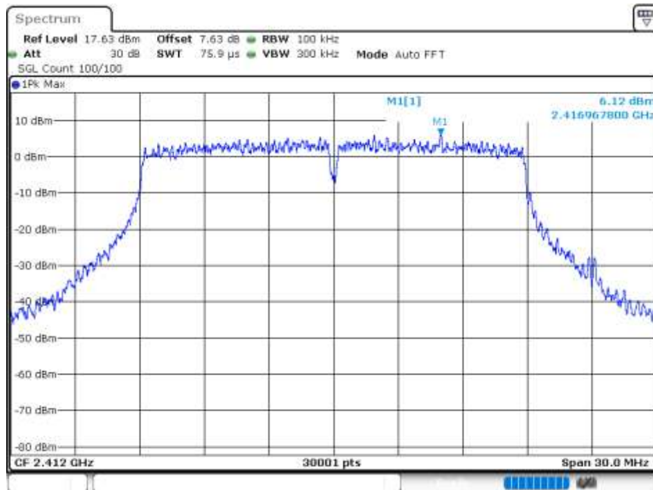
Tx. Spurious NVNT 802.11n(HT20) 2412MHz Ant 3 Emission
