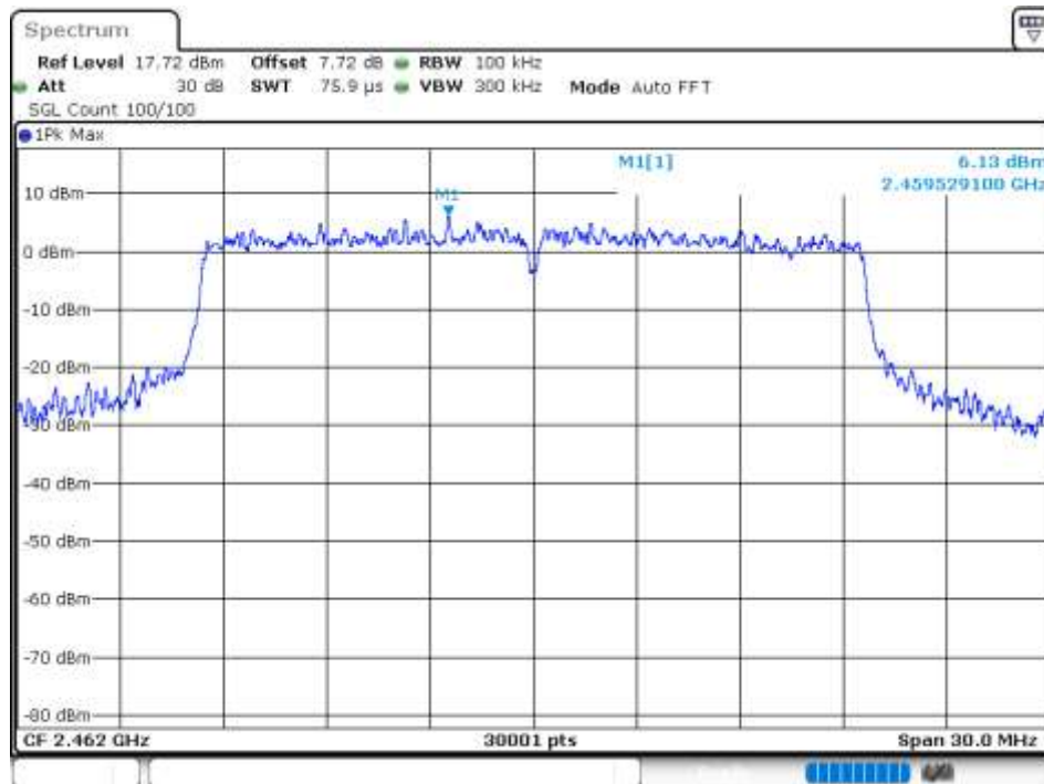
Tx. Spurious NVNT 802.11ax20 2462MHz Ant 1 Emission
