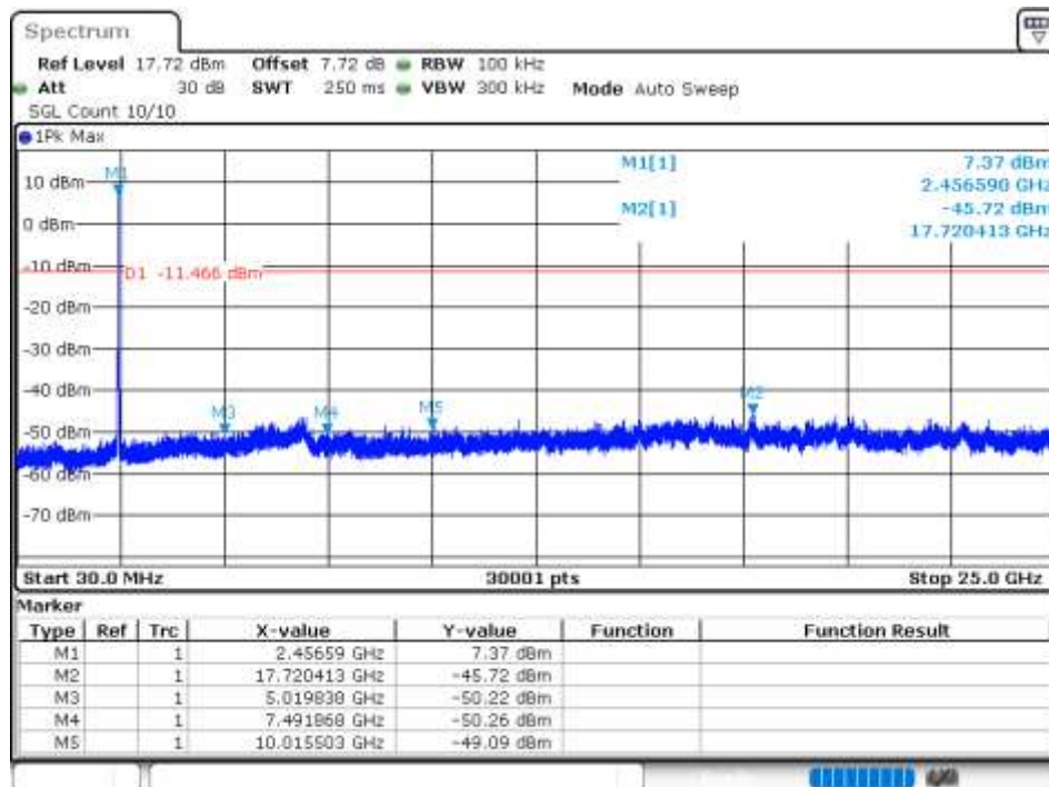
Tx. Spurious NVNT 802.11g 2462MHz Ant 3 Emission
