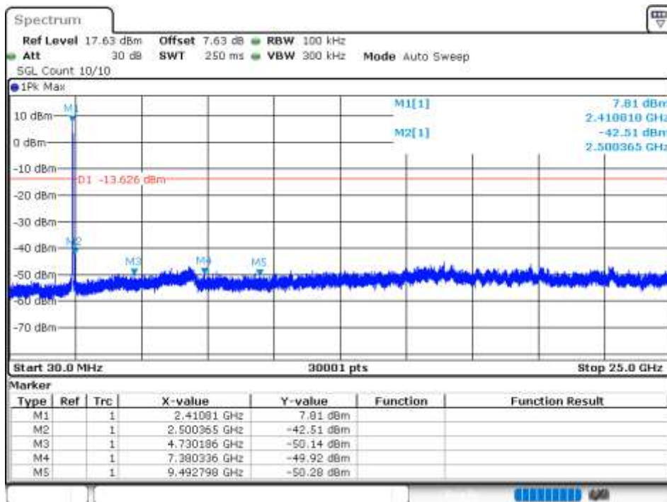
Tx. Spurious NVNT 802.11ax20 2412MHz Ant 3 Emission
