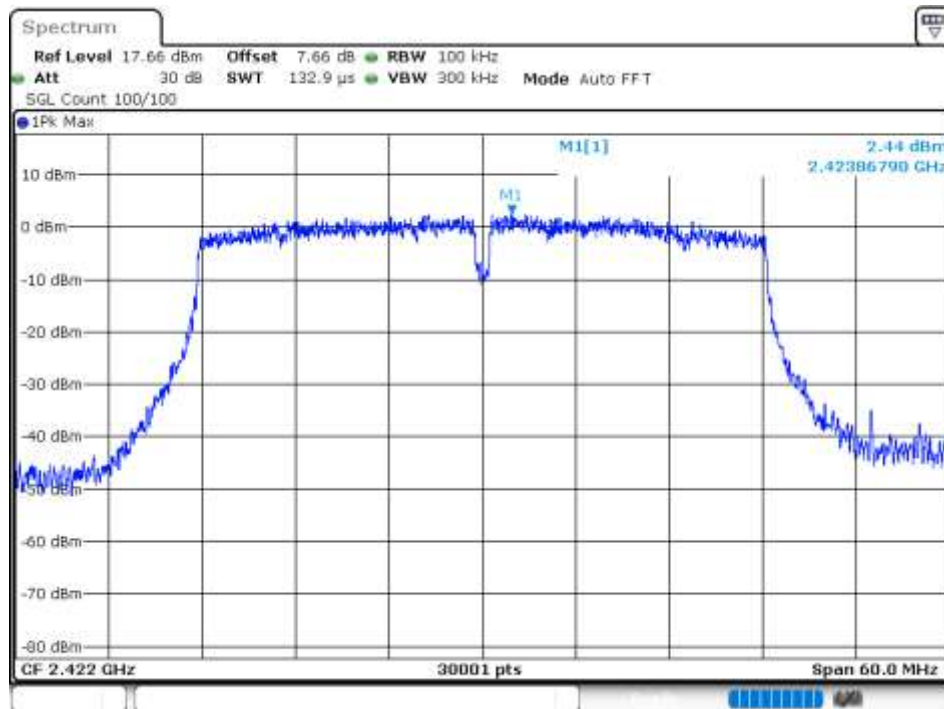
Tx. Spurious NVNT 802.11n(HT40) 2422MHz Ant 0 Emission
