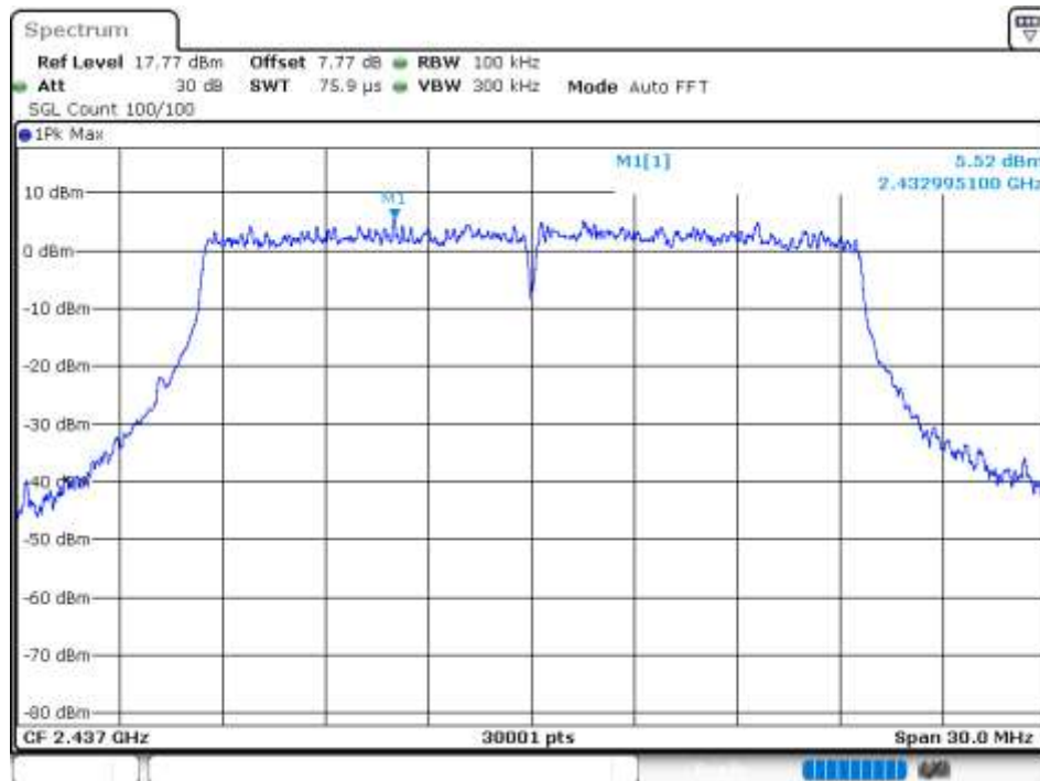
Tx. Spurious NVNT 802.11ax20 2437MHz Ant 3 Emission
