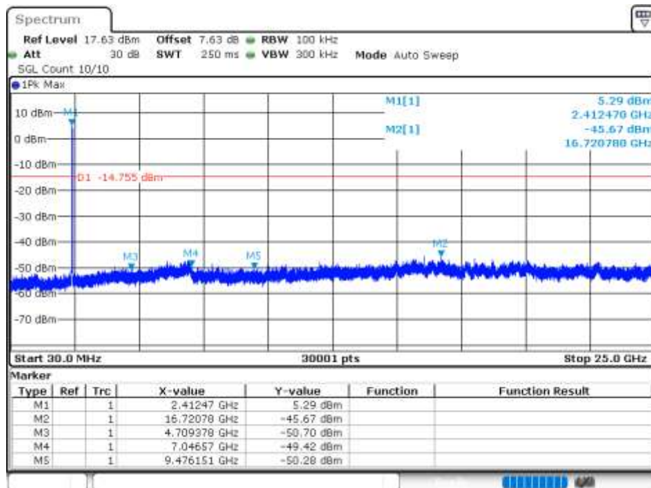
Tx. Spurious NVNT 802.11n(HT20) 2412MHz Ant 0 Emission
