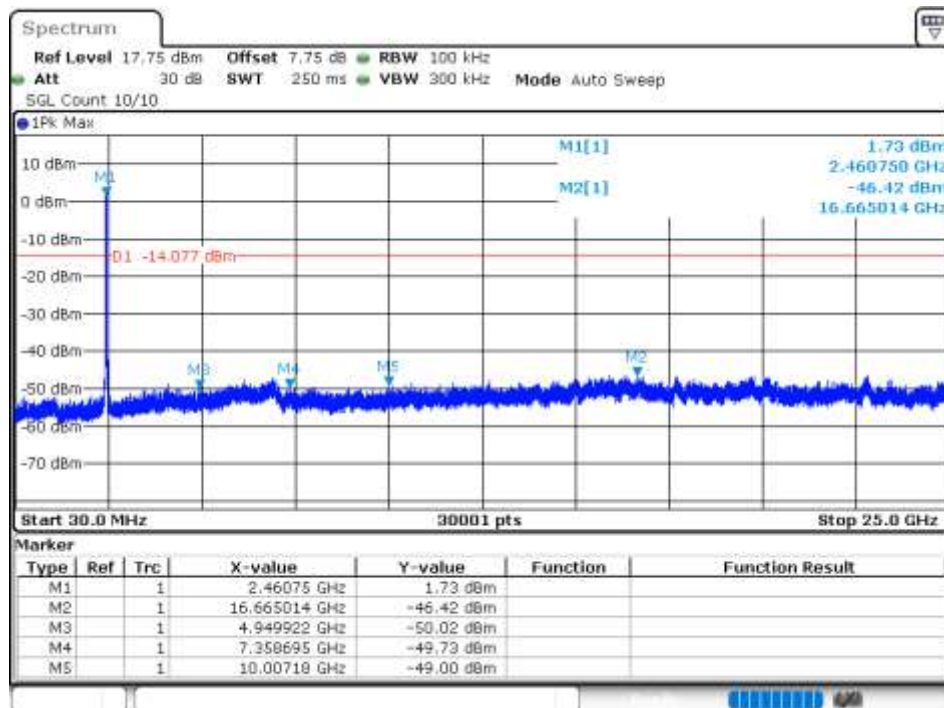
Tx. Spurious NVNT 802.11n(HT40) 2452MHz Ant 3 Emission
