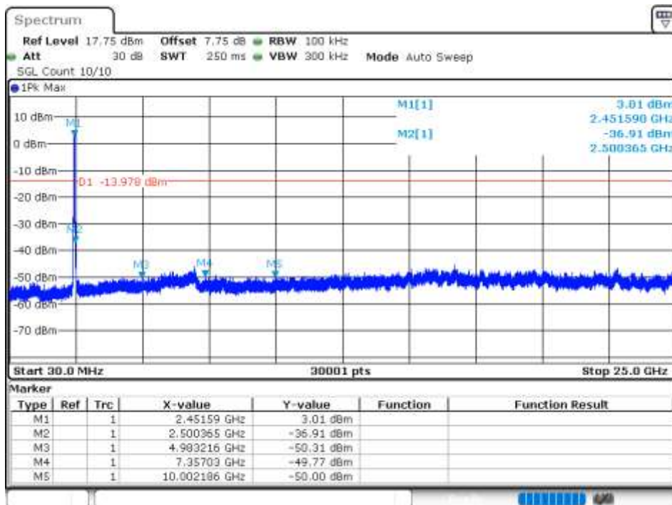
Tx. Spurious NVNT 802.11ax40 2452MHz Ant 1 Emission
