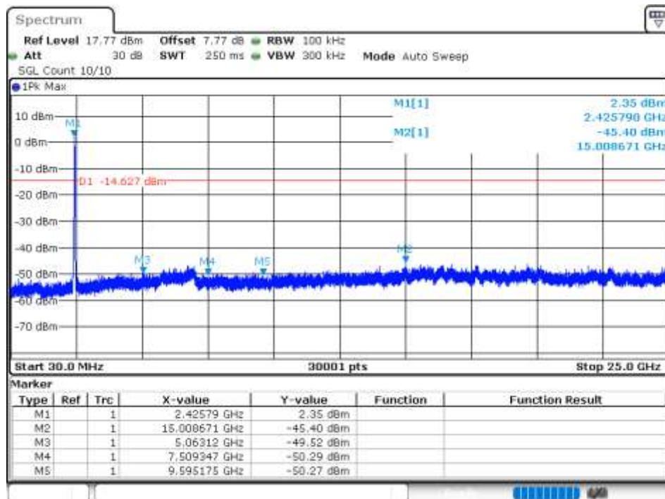
Tx. Spurious NVNT 802.11n(HT40) 2437MHz Ant 0 Emission
