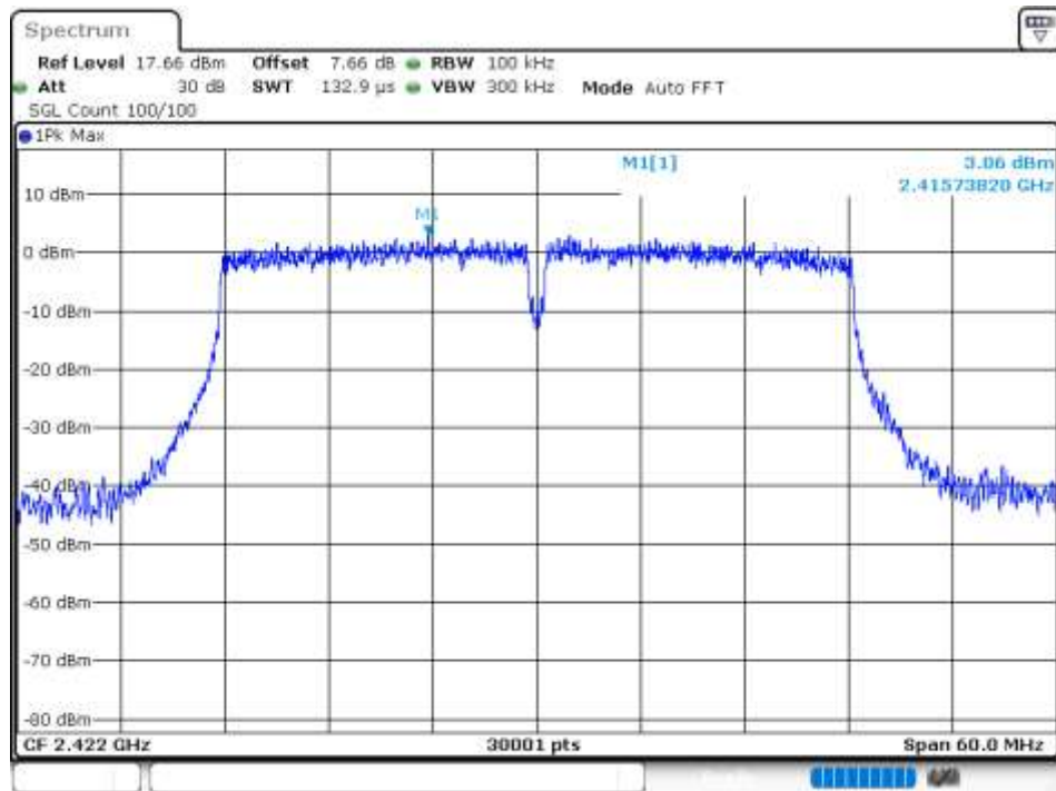
Tx. Spurious NVNT 802.11n(HT40) 2422MHz Ant 3 Ref
