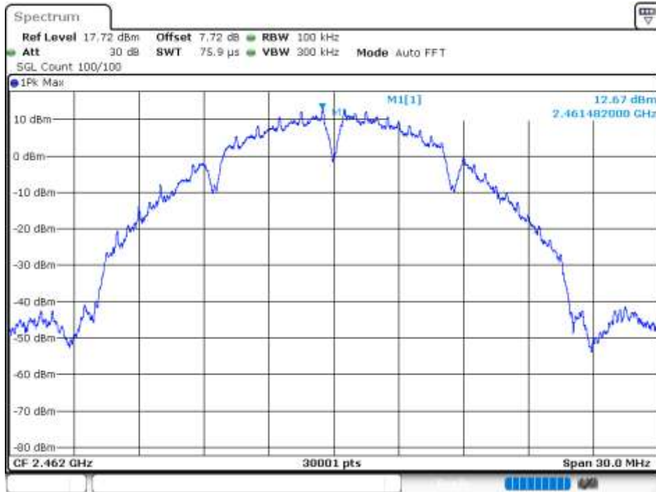
Tx. Spurious NVNT 802.11b 2462MHz Ant 3 Emission
