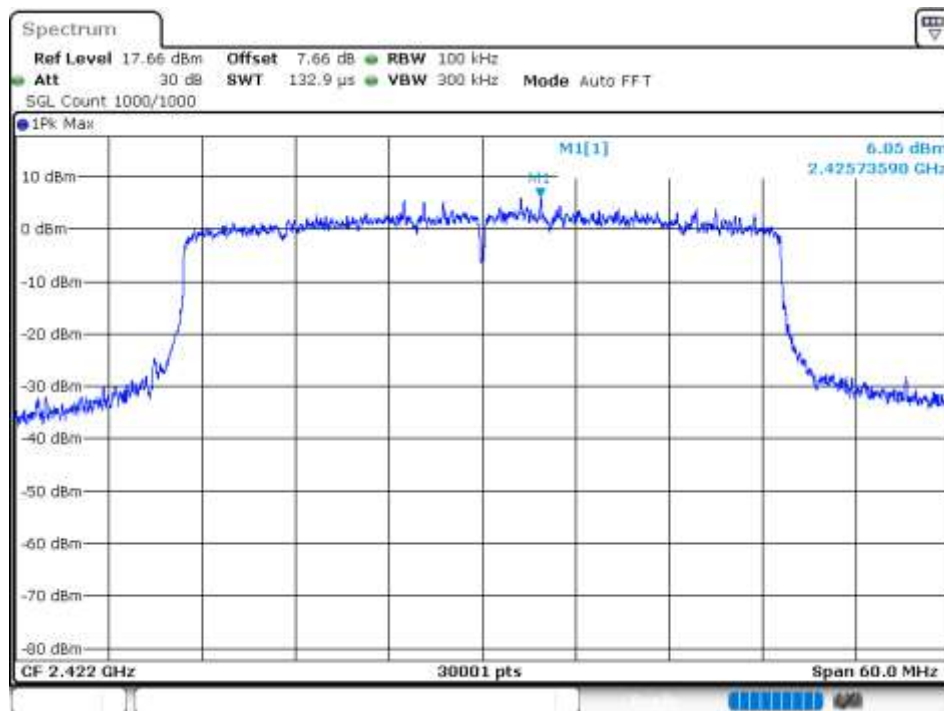
Tx. Spurious NVNT 802.11ax40 2422MHz Ant 1 Emission
