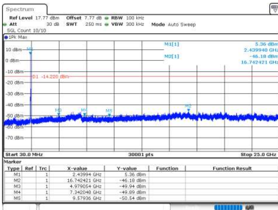
Tx. Spurious NVNT 802.11ax20 2437MHz Ant 1 Emission
