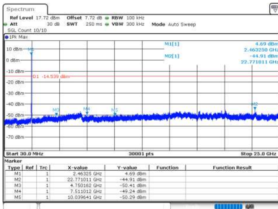
Tx. Spurious NVNT 802.11n(HT20) 2462MHz Ant 3 Emission
