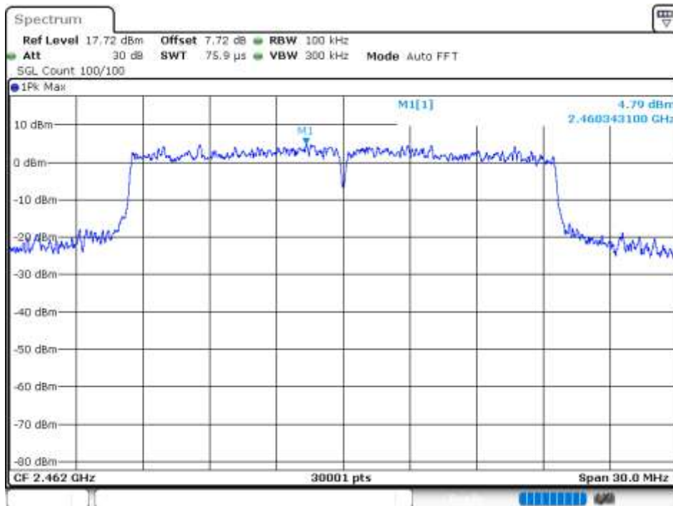
Tx. Spurious NVNT 802.11ax20 2462MHz Ant 0 Emission
