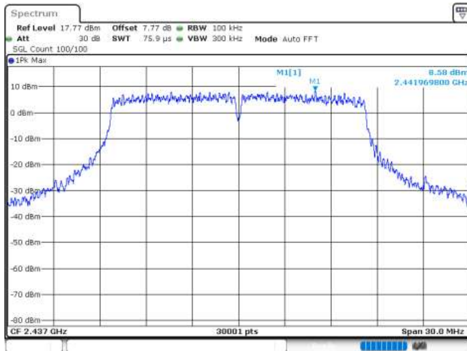
Tx. Spurious NVNT 802.11g 2437MHz Ant 3 Emission
