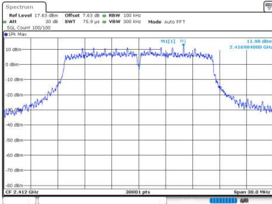
Tx. Spurious NVNT 802.11g 2412MHz Ant 3 Emission
