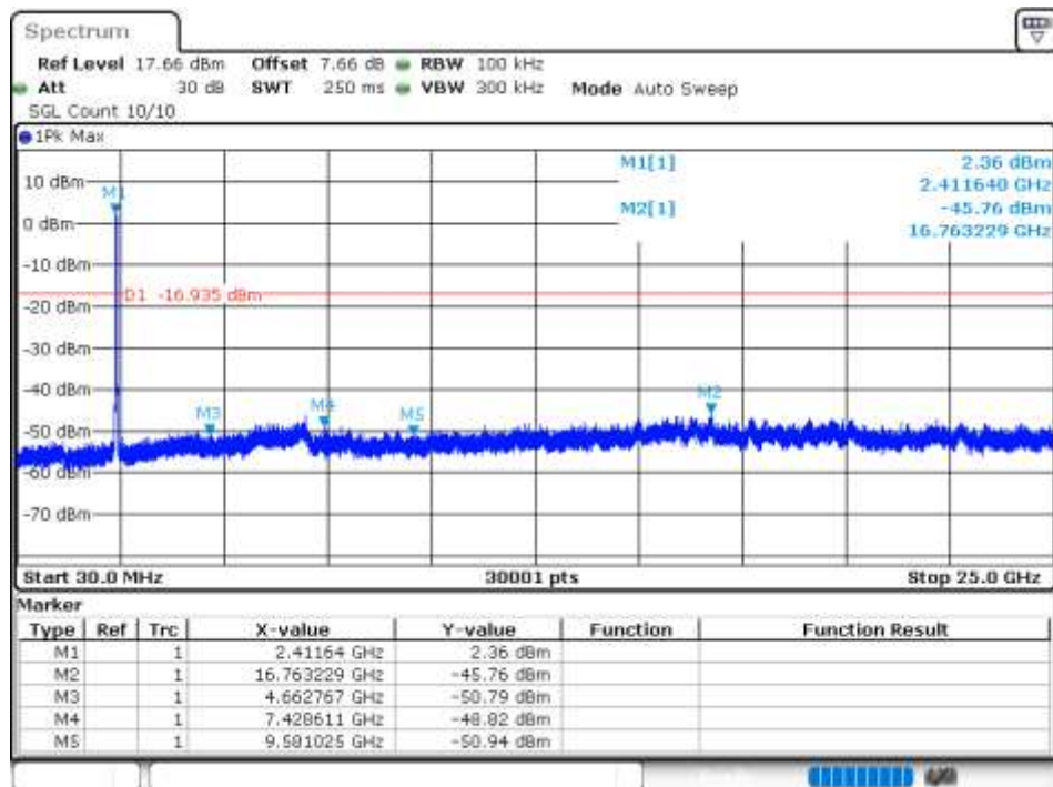
Tx. Spurious NVNT 802.11n(HT40) 2422MHz Ant 3 Emission
