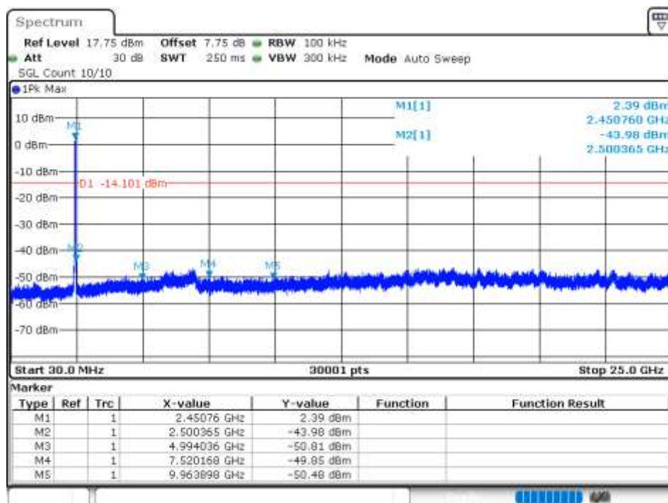
Tx. Spurious NVNT 802.11ax40 2452MHz Ant 3 Emission
