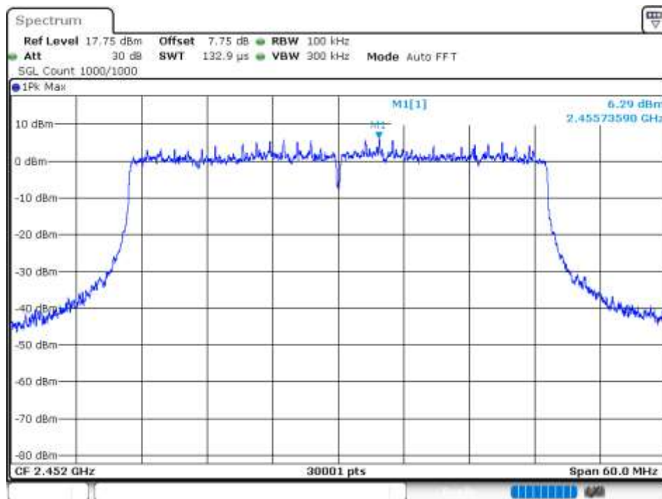
Tx. Spurious NVNT 802.11ax40 2452MHz Ant 2 Emission
