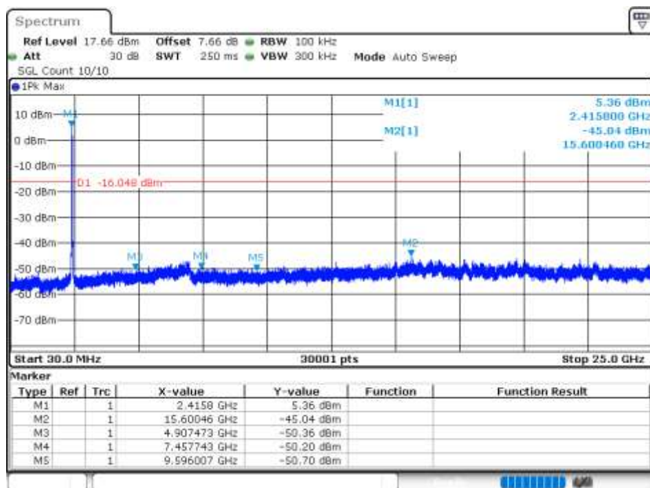
Tx. Spurious NVNT 802.11ax40 2422MHz Ant 3 Emission
