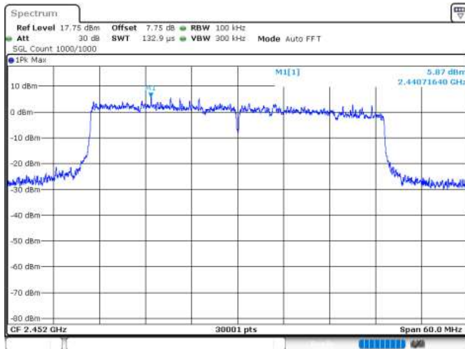
Tx. Spurious NVNT 802.11ax40 2452MHz Ant 0 Emission
